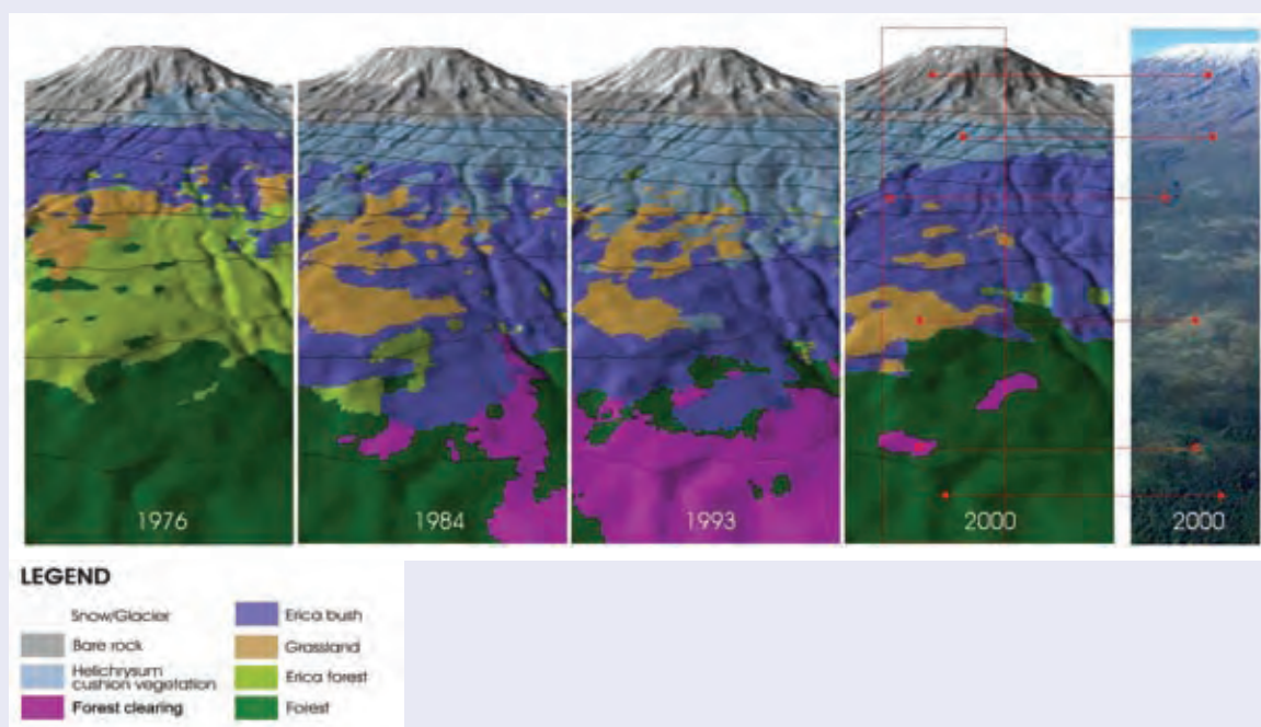
Figure 5.3: Land cover changes induced by complex land use and climate interactions on Kilimanjaro (Hemp, 2005). Reprinted by permission from Blackwell Publishing Ltd.
