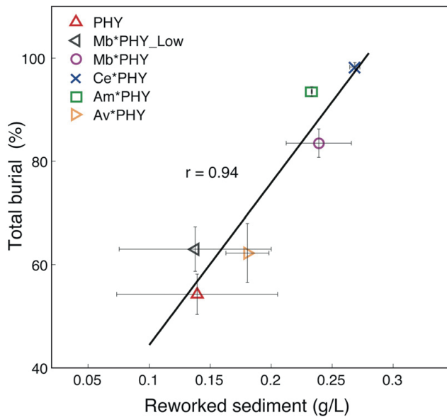
Fig.4.2. A linear correlation between total burial (Mean \pm SE, n=4 ) and the amount of reworked sediment (Peak SSC, Mean \pm SE, n=2 ) under purely physical process (PHY) and the coupling between currents and animals (the rest).
