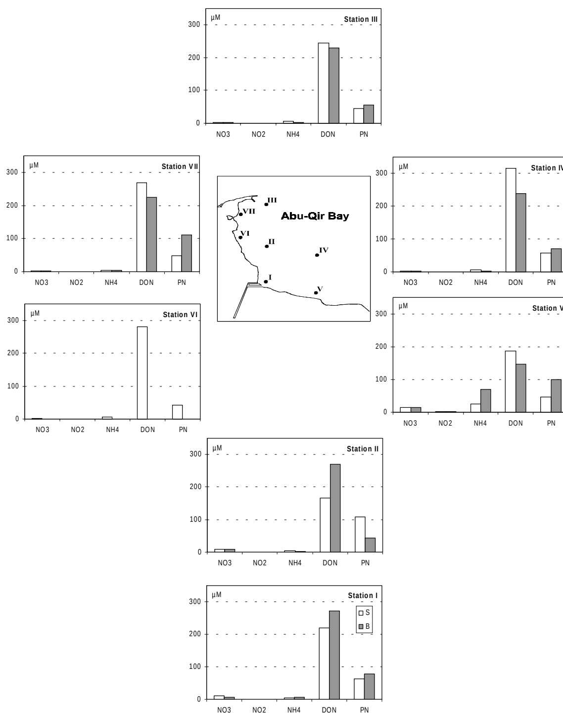
Figure 4. Regional variations of \text{NO}_3 , \text{NO}_2 , \text{NH}_4 , DON and PN ( \mu\text{M} ) in surface and bottom water layers of Abu-Qir Bay.
