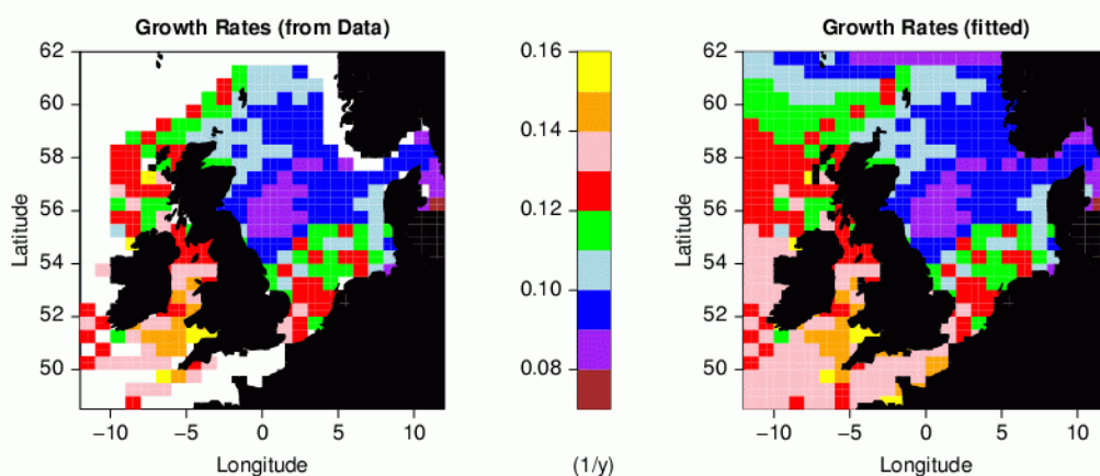
Figure 4.3.1 The left graph shows the growth rates fitted using SMALK data. The right graph shows the growth rates for the entire region, with missing data filled in using the correlation between growth and temperature and location.
