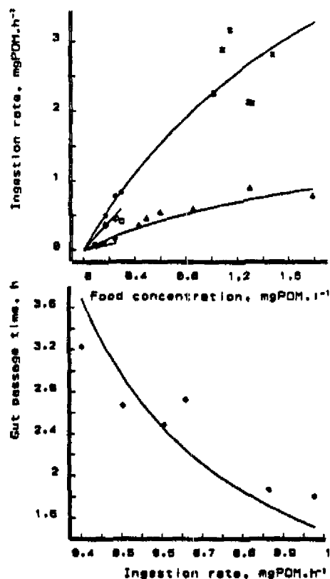
Figure 5: The ingestion rate, I , as function of food density, X , for different shell lengths, L . Food is added as mixtures of algae or organic matter with silt (anorganic particles). Rates are corrected to 15°C and the shell lengths are resp. (from bottom to top) 1.75, 2.5, 4.25, 4.8 and 4.8 cm, data from resp. Kjørboe et al. , (1981); Bayne et al. (1989); Bayne et al. (1987) and Smaal et al. (1988). The simultaneously least squares fitted curves are I = \{I_m\}(\alpha L)^2 X / (K + X) , with \{I_m\} = 3.0 (SD 1.0) \text{mg POM.cm}^{-2}.\text{h}^{-1} and K = 2.4 (SD 1.3) \text{mg POM.l}^{-1} .
