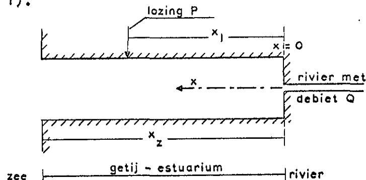
fig. 1 Defenitie - schets
