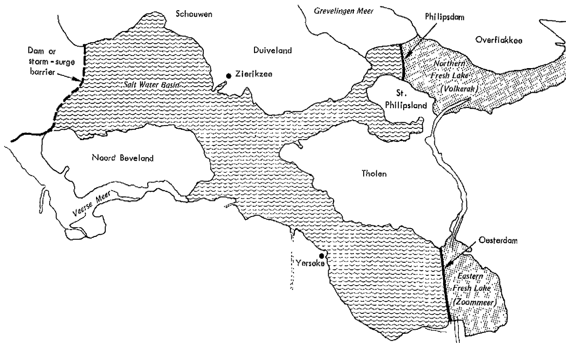
Fig. 12.1a — Compartment design "3"
