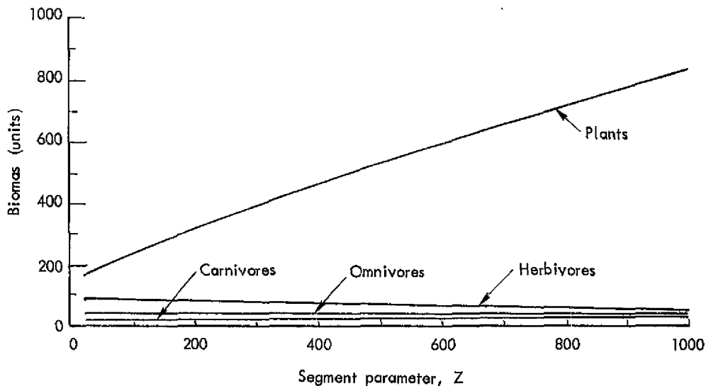
Fig. 4.3 — Abundances vs. segment parameter, Z (nominal value of Z = 100 )
