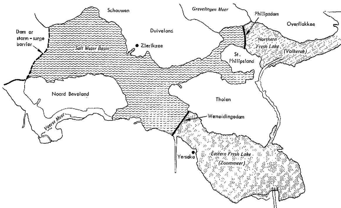
Fig. 1.2b — Compartment design "4"
