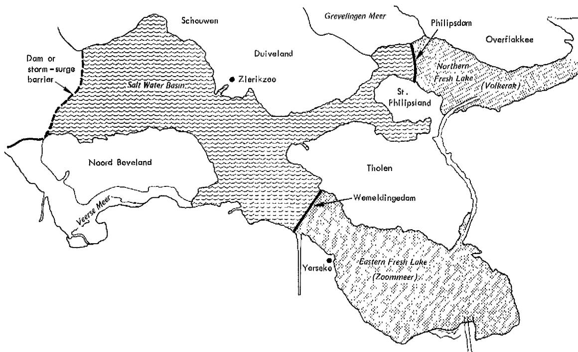
Fig. 12.1b — Compartment design "4"
