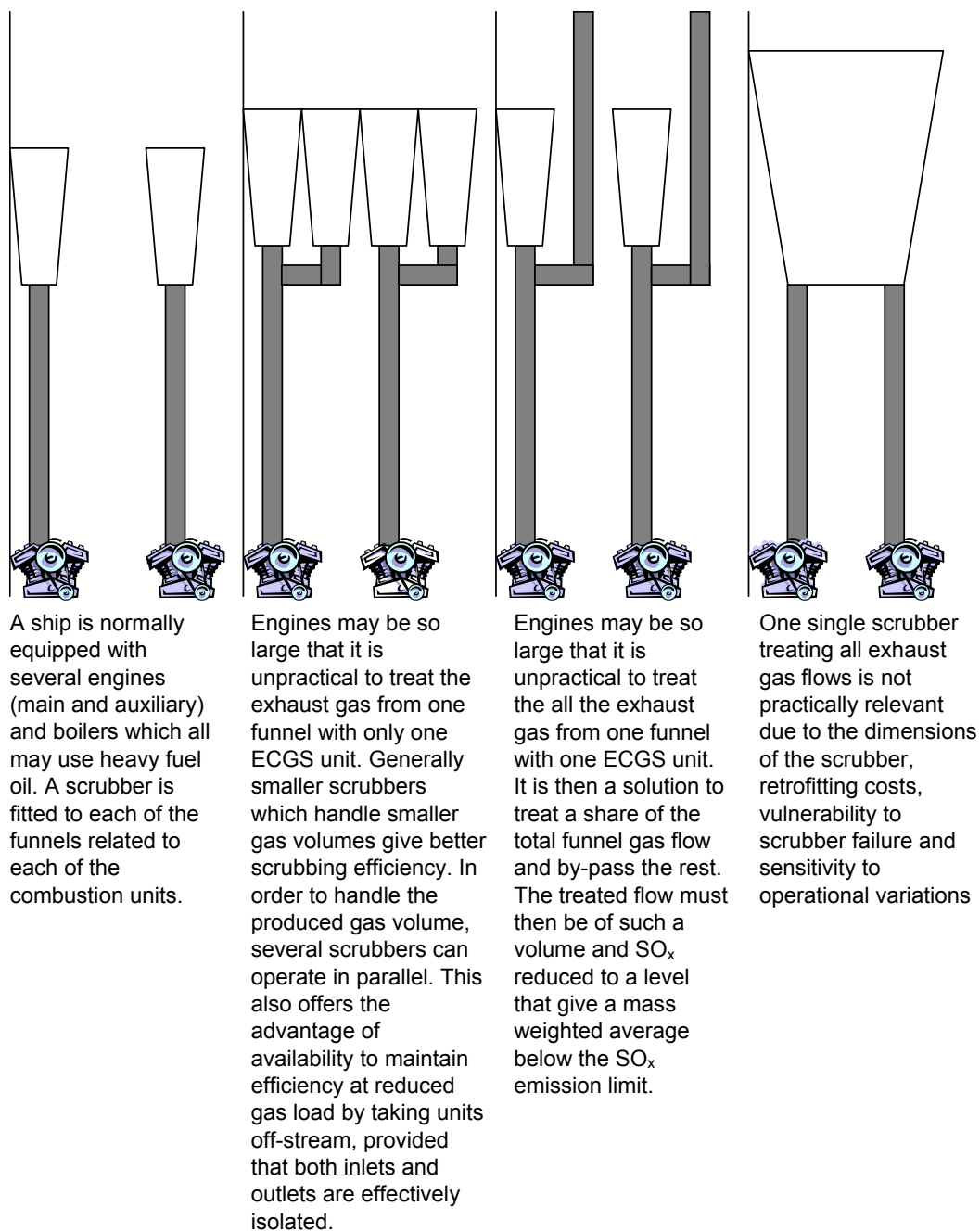
Figure 26 Alternative arrangements of scrubbers to the funnels
