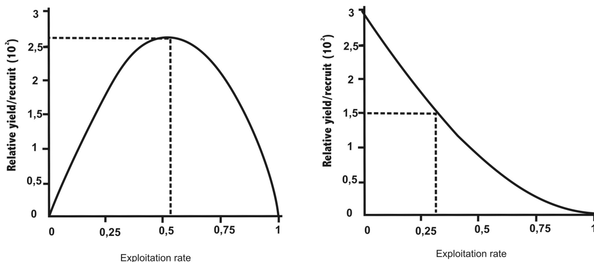
FIG. 4. – Relative yield-per-recruit (left) and relative biomass-per-recruit (right) for M. macrobrachion females of the Cross River estuary, Nigeria, based on the selection ogive option ( E_{\max} = 0.53 , E_{0.1} = 0.51 , E_{0.5} = 0.31 ).
