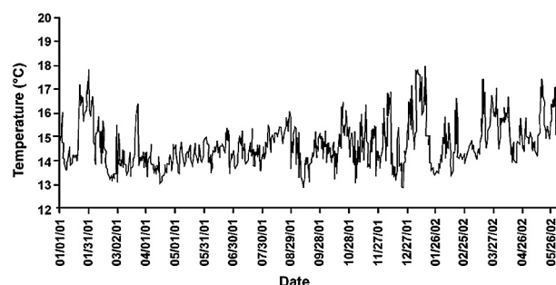
FIG. 2. – Average daily water temperature obtained at 16 m depth at the La Rinconada Marine Reserve, Antofagasta, Chile between January 2001 and May 2002.
