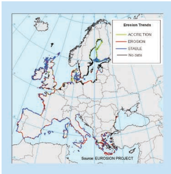
Fig. 72: Coastal erosion patterns; Length of coastline dynamics, based on EUROSION database.
