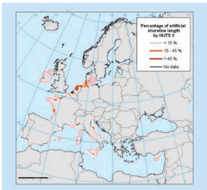
Fig. 76: Percentage of artificial shoreline length by NUTS3, source: ETC-ET (EEA).
