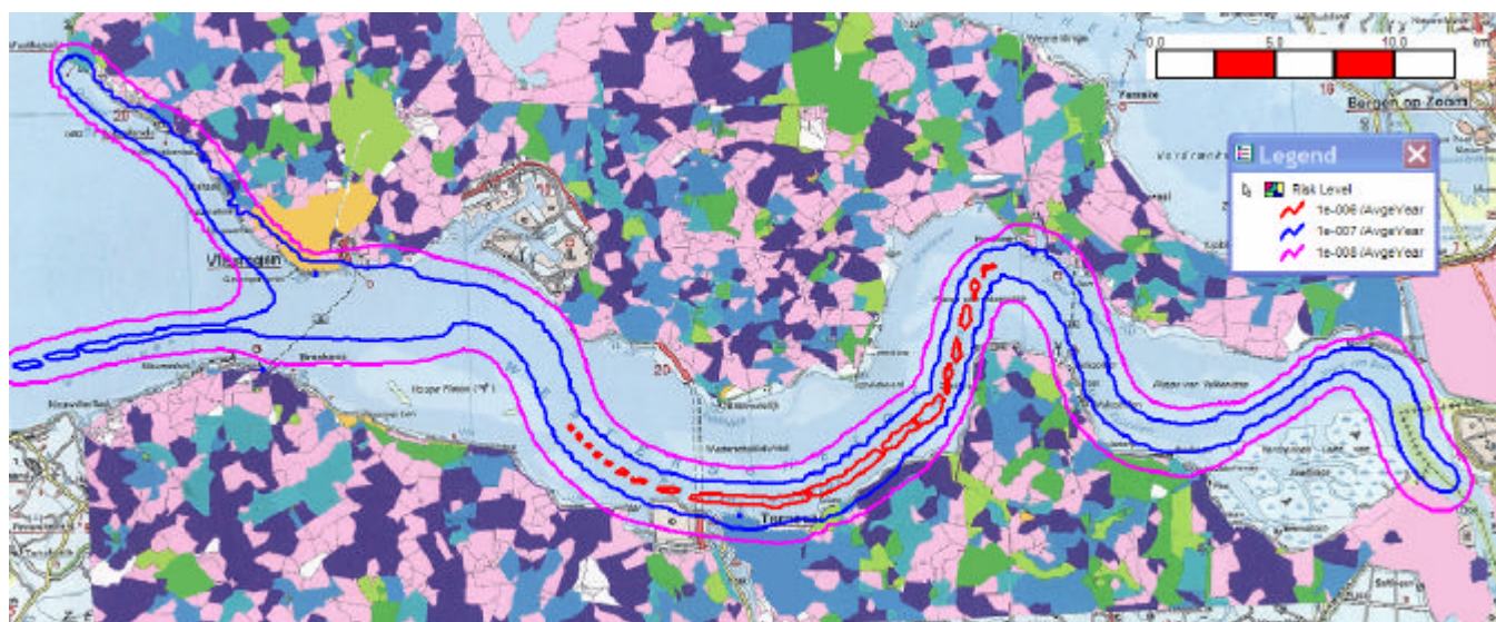
FIGURE II.6. –COMBINED INDIVIDUAL RISK CONTOURS for 2010 GC Y
