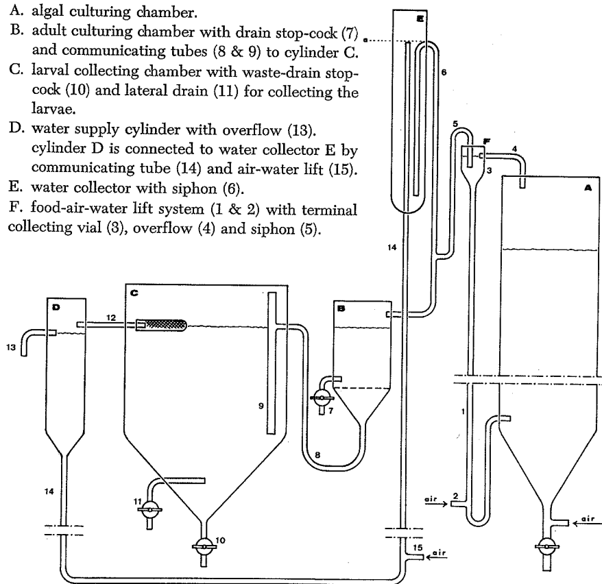
Fig. 1. Schematic presentation of the apparatus.
