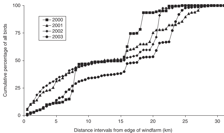
Figure 3. Cumulative percentage distribution of Long-tailed Ducks Clangula hyamelis at 500 m intervals from the periphery of the Nysted offshore wind farm, based on all aerial survey data in 2000, 2001 and 2002 (pre-construction), and post-construction in 2003. See Kahlert et al. (2004) for full explanation and methods.
