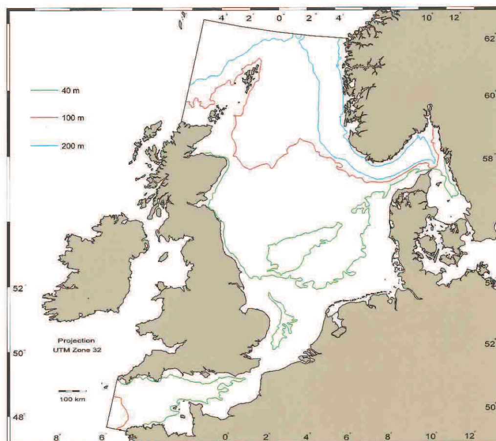
Bathymetry of the study region.
