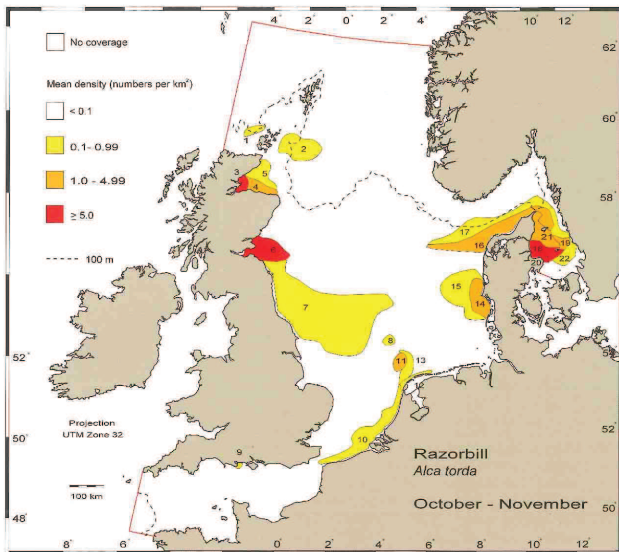
Distribution and density of Razorbill Alca torda in the North Sea, the Channel and the Kattegat from October to November 1980-1994.
