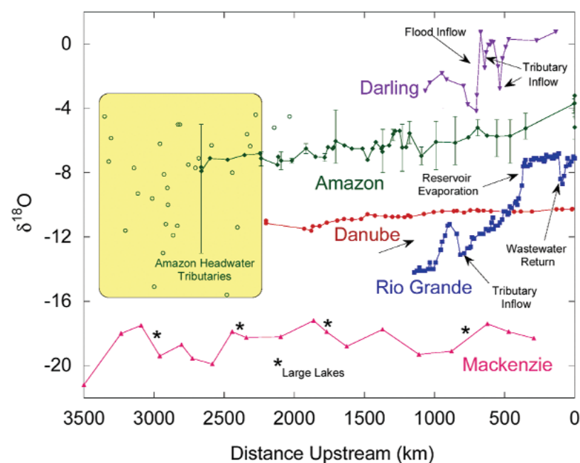
Figure 4.3: Oxygen-18 content of stream water along the main stem of large rivers
