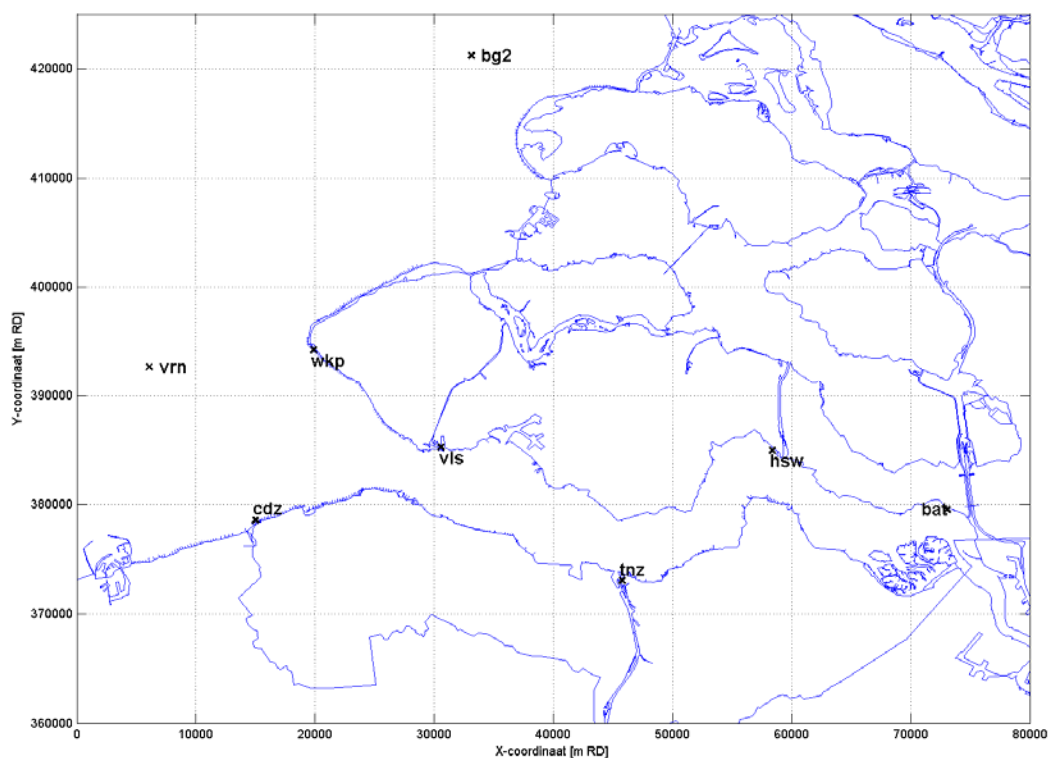
Figuur 4.1: Waterstandmeetlocaties.
