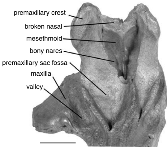
FIG. 19. — Detail of the premaxillary sac fossae and the vertex of Choneziphius planirostris (Cuvier, 1823) (IRSNB 3775-M.1883) in anterodorsal view. Scale bar: 50 mm.
