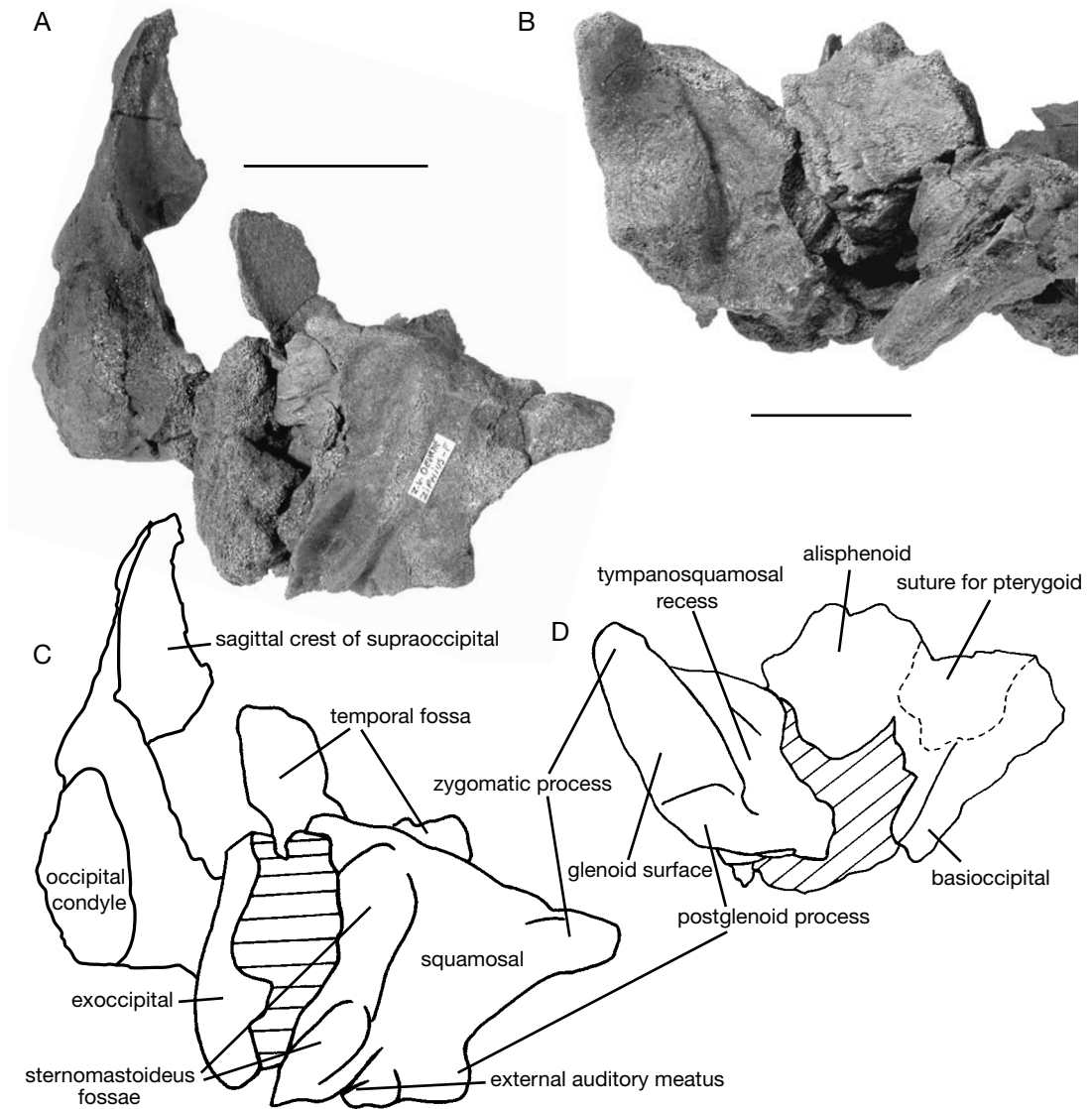
FIG. 8. — Ziphirostrum marginatum du Bus, 1868 (IRSNB M.1877) from the Deurne Sands Member, late Miocene, Deurne, Antwerp; A , right lateral view of the basicranium; B , ventral view of the right part of the basicranium; C , line drawing in right lateral view; D , line drawing in ventral view. Scale bars: 50 mm.
