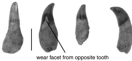
FIG. 9. — Four detached teeth of Ziphirostrum marginatum du Bus, 1868 (IRSNB M.1877) from the Deurne Sands Member, late Miocene, Deurne, Antwerp. One of the teeth displays a wear facet from contact with an opposite tooth. Scale bar: 10 mm.
