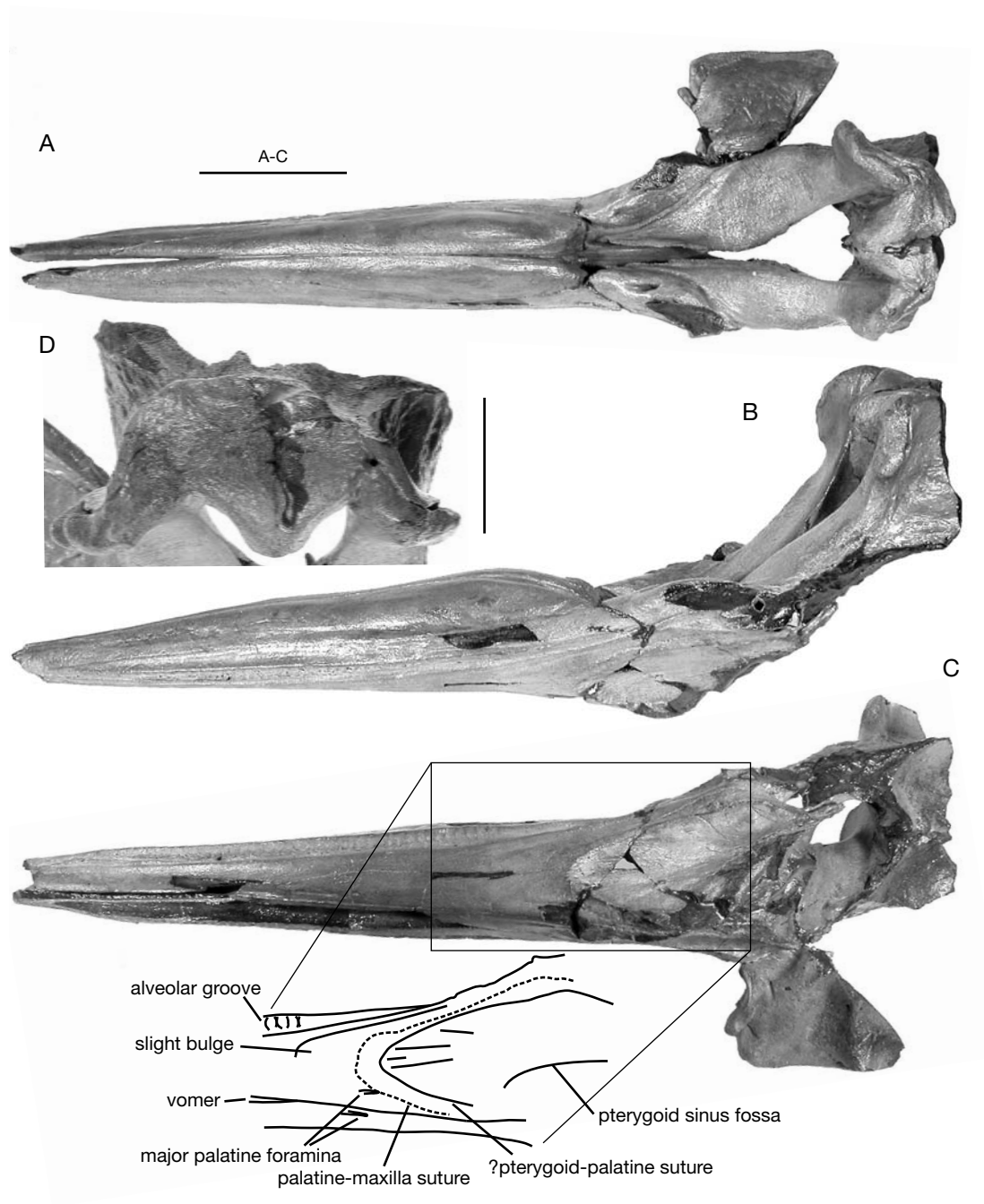
FIG. 5. — Skull of Ziphirostrum marginatum du Bus, 1868 (IRSNB 3847-M.537); A , dorsal view; B , left lateral view; C , left ventrolateral view and line drawing detailing the palate; D , detail of the vertex in dorsal view. Scale bars: A-C, 100 mm; D, 50 mm.
