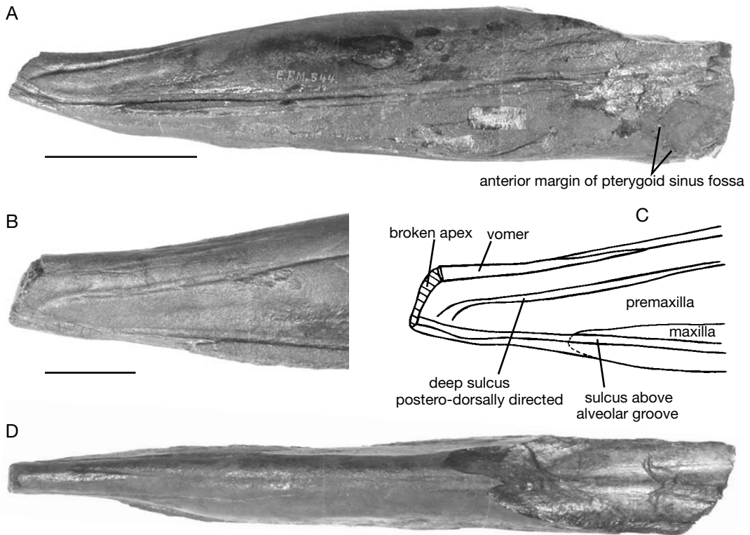
FIG. 15. — Rostrum of Ziphrostrum recurvus (du Bus, 1868) n. comb. (IRSNB 3805-M.544, holotype); A , left lateral view; B , detail of the apex in dorsolateral view; C , line drawing of the apex in dorsolateral view, indicating the filling of the mesorostral groove by the dense vomer; D , dorsal view. Scale bars: A, D, 100 mm; B, C, 50 mm.
