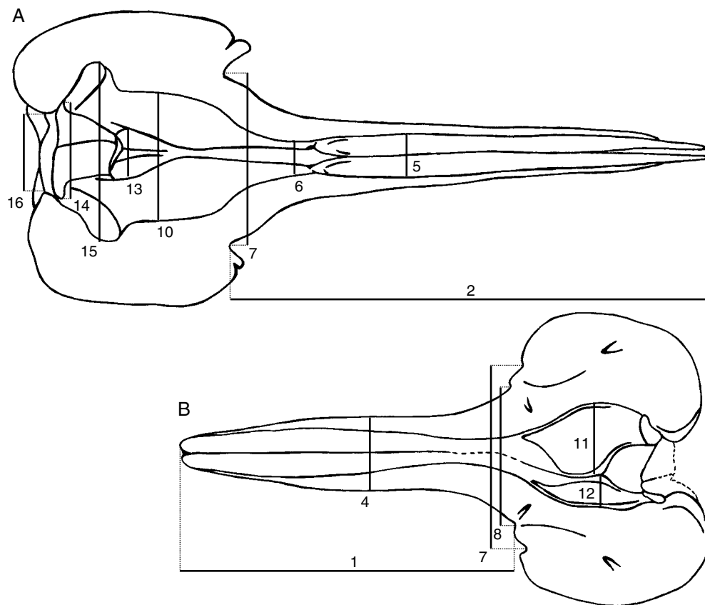
FIG. 1. — Line drawings showing the measurements used for the different ziphiid taxa in this work; A , Ziphiostrum marginatum du Bus, 1868 (combination of IRSNB 3845-M.536 and IRSNB 3847-M.537); B , Choneziphius planirostris (Cuvier, 1823) (reconstruction from IRSNB 3774-M.1881). For the values of each measurement, see Tables 1–4 and 6.
