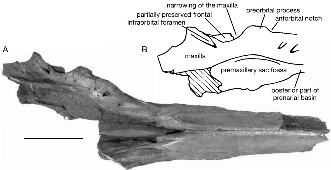
FIG. 7. — A , rostrum and left supraorbital process of Ziphiostrum marginatum du Bus, 1868 (IRSNB 3830-M.542) ( Z. laevigatum sensu du Bus, 1868) in dorsal view; B , line drawing of the left supraorbital process displaying an unusual narrowing of the maxilla posterior to the preorbital process. Scale bar: A, 100 mm.
