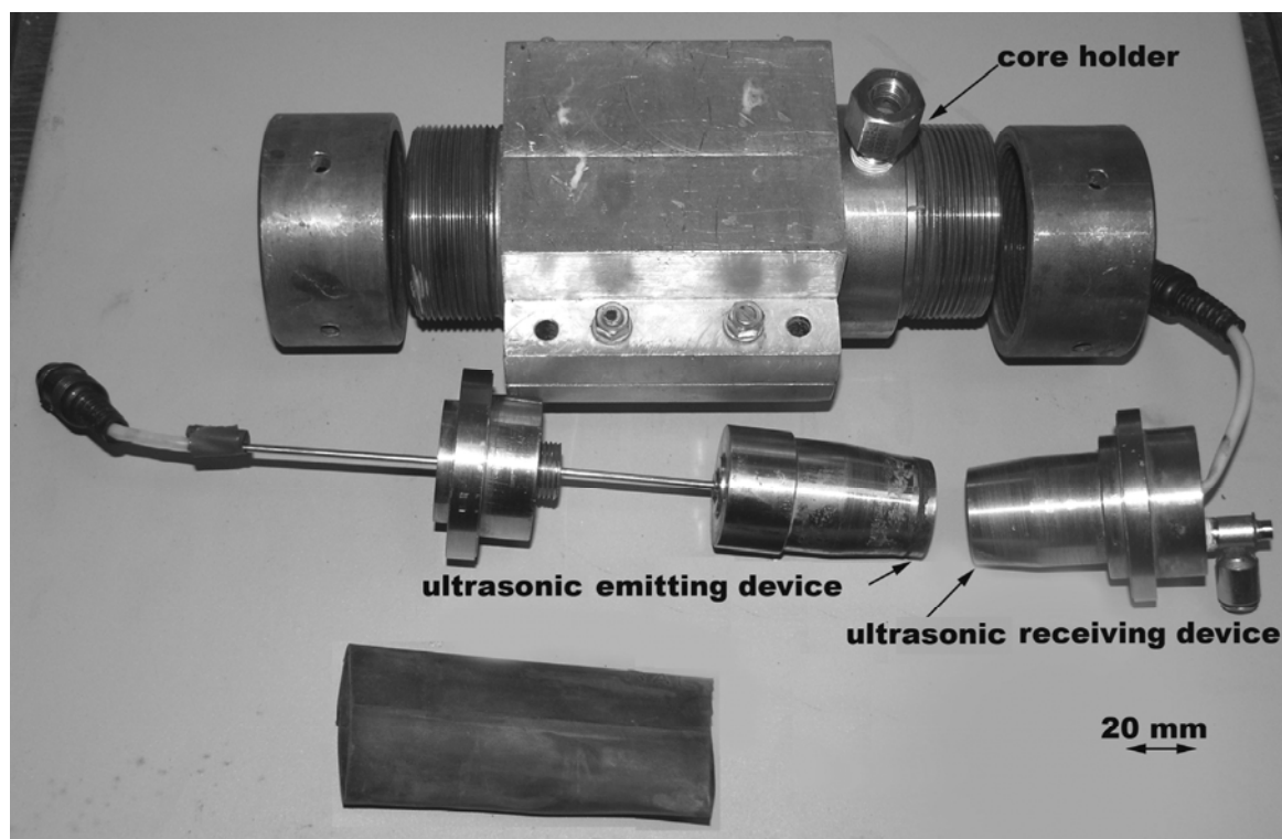
Figure 2. Acoustic measurement block of the PUMA-650 analyser
