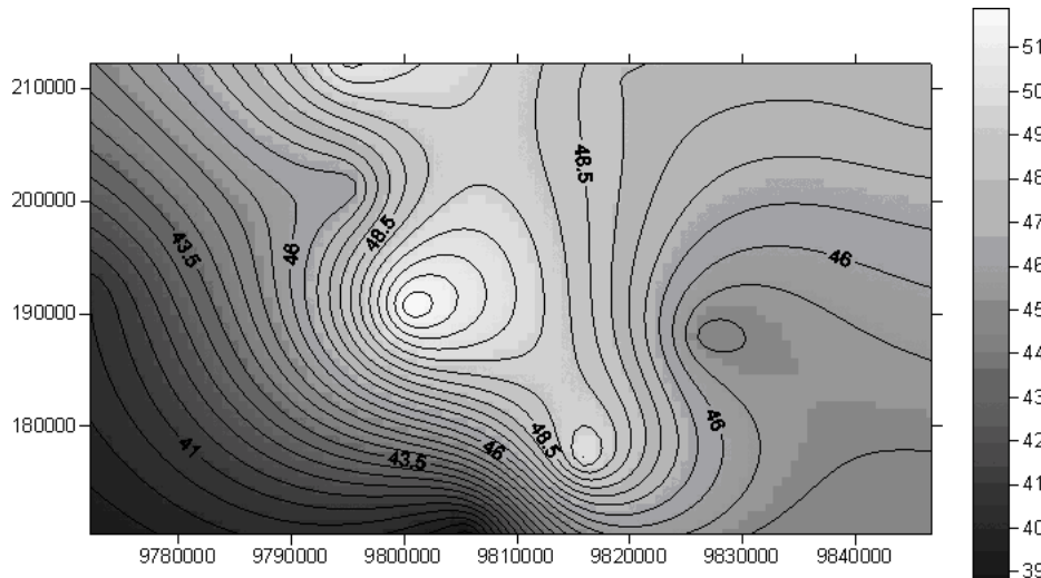
Figure 2. Porosity map of the Miocene formation
