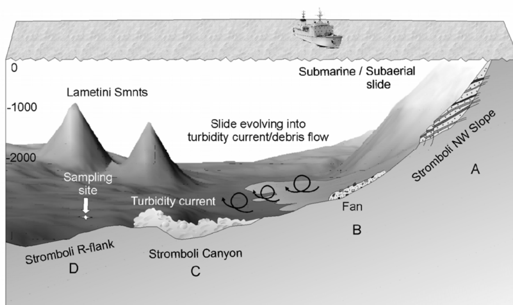
Figure 2. The likely model of formation of the volcanoclastic turbidite deposit, on the right flank of Stromboli canyon. a) Accumulations of unstable volcanoclastic material (lava flows and loose volcanoclastic sediments) on the NW flank of Stromboli volcano collapse when perturbed ( ex: magma dike intrusion, gravity instabilities, earthquake activity...) , resulting in a sub aerial-submarine landslide inside the Sciara del Fuoco depression, b) the slide consist of a coarse grained debris avalanche, accumulating on the sedimentary fan covering almost the whole NNW volcano flank c) coarse deposit evolves in a high energy turbidity currents down the volcano slope d) thanks to their great mobility the turbidity currents override the 200 m-high flank of Stromboli Canyon depositing the volcanoclastic turbidite sequences
