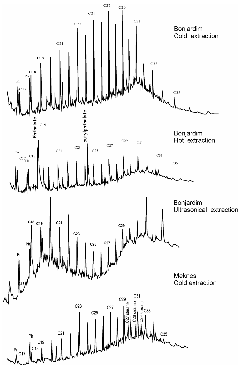
Figure 2. Chromatograms of cold, hot, and ultrasonic extract from the Bonjardim and Meknes mud volcanic deposits
