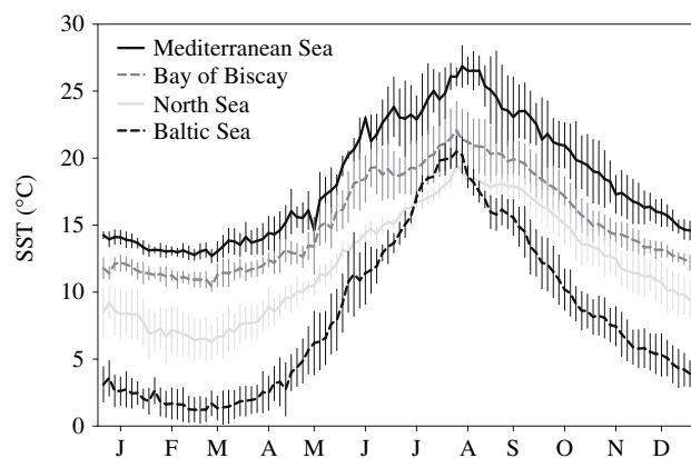
Fig. 2 Annual sea surface temperature (SST) regimes for the sampling stations in the Baltic Sea, the North Sea, the Bay of Biscay, and the Mediterranean Sea. Lines and error bars represent monthly averages and standard deviations, based on measurements taken by satellite twice daily, at 9 a.m. and 2 p.m., during the period 2003D2005. This data were taken from the NASA JPL website (NASA Jet Propulsion Laboratory 2005)
