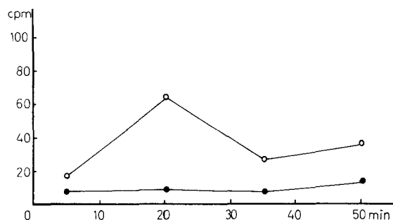
Fig. 4. Corophium volutator . Uptake of labelled bacteria (Strain g) in 125 to 250 \mu\text{m} sand fraction with (open circles) and without (filled circles) addition of 5% silt and clay
