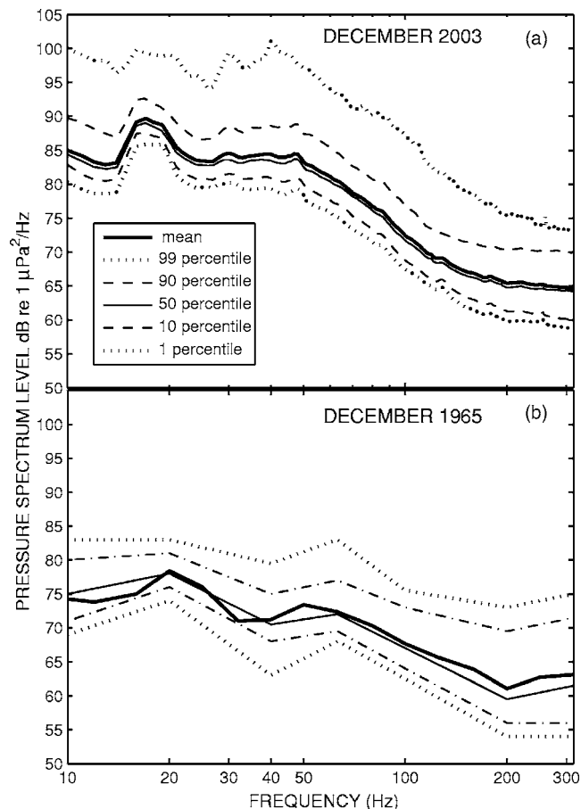
FIG. 6. (a) December 2003 cumulative distribution function for pressure spectrum levels at the San Nicolas South site. (b) December 1965 at the San Nicolas South site, after Wenz (1968a). Note the 50th percentile line does not closely track the mean because the mean was computed at 1/3 as many frequencies as the 50th percentile, each over a wider bandwidth.
