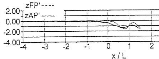
Figure 11: Bulkcarrier (260x43x17 m 3 ) entering lock (h/T=1.2, W/B=1.23, Δy/B=0.087, drift 0, 1.6 knots, rpm 64%): undimensioned forces; sinkage (%T)
