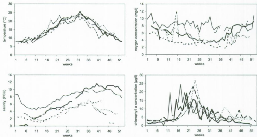
Fig. 2: Seasonal variation throughout the years in environmental variables in the cooling water system at BASF, Antwerpen N.V. ( --- 2000; ---- 2001; - - 2002; — 2003; — 2004)
