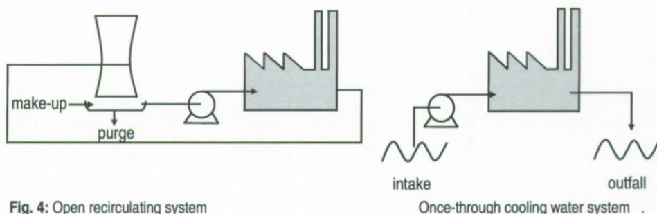
Fig. 4: Open recirculating system
