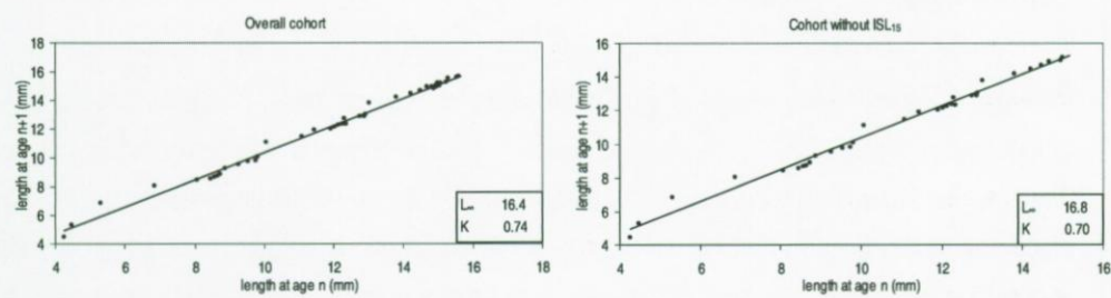
Fig. 6: Graphical presentation of the Ford-Walford method for the estimation of L_{\infty} and K. L_{\infty} = intercept / (1 - slope); K = (-1/dt) \cdot \ln(\text{slope}) .
