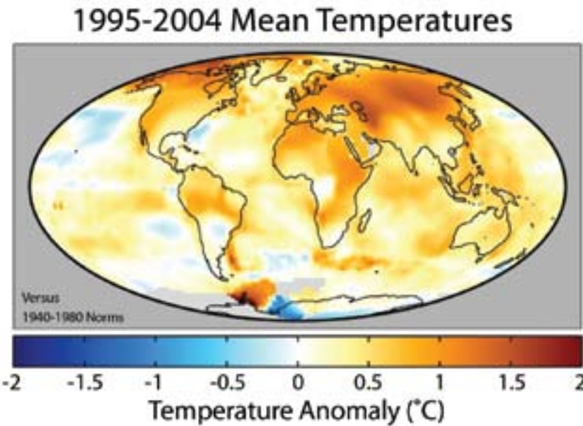
Figure 2.1.2. Regional variation in global temperature change. This plot is based on the NASA GISS Surface Temperature Analysis (GISTEMP), which combines the 2001 GISS land-station analysis dataset (Hansen et al., 2001) with the Rayner-Reynolds oceanic sea surface temperature dataset (Rayner, 2000; Reynolds et al., 2002). The data themselves were prepared through the GISTEMP online mapping tool, and the specific dataset used is available at http://data.giss.nasa.gov/cgi-bin/gistemp/do_nmap.py?year_last=2007&month_last=10&sat=4&sst=1&type=anomaly&mean_gen=0112&year1=1995&year2=2004&base1=1940&base2=1980&radius=1200&pol=reg . These data were replotted in a Mollweide projection with a continuous and symmetric colour scale. The smoothing radius is 1200 km, meaning that the reported temperature may depend on measurement stations located up to 1200 km away, if necessary. Image prepared by Robert A. Rohde from public domain data for Global Warming Art ( http://www.globalwarmingart.com/wiki/Image:Global_Warming_Map.jpg ).
