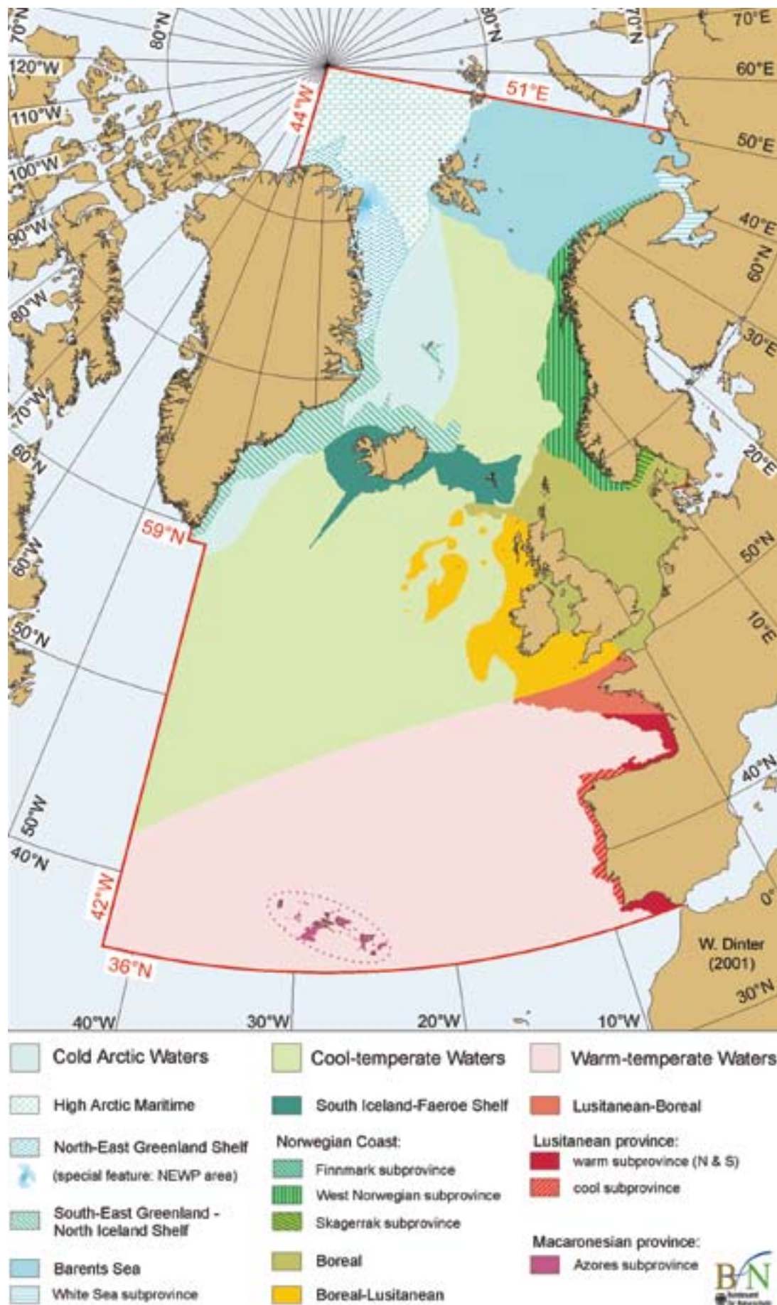
Figure 1.1.2. Biogeographical classification of the benthic and neritic provinces of the shelf and upper continental slope (<1000 m depth), and of ice-cover biomes combined with the superordinate holopelagic provinces (<1000 m depth) of the OSPAR Maritime Area (reproduced from Dinter (2001) and based on Forbes and Godwin-Austen (1977)).
