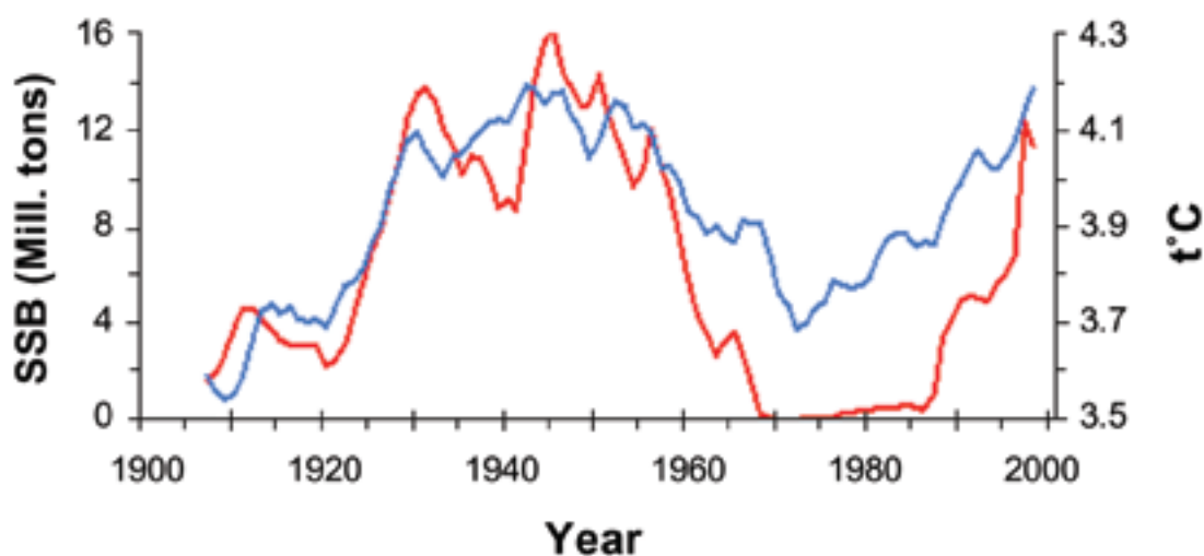
Figure 3.3.6. Variations in the spawning-stock biomass of Norwegian spring-spawning herring (red line) and sea temperature (blue line). The stock collapse in the 1960s was a combined effect of the decrease in sea temperature and high fishing pressure (from Tøresen and Østvedt, 2000).
