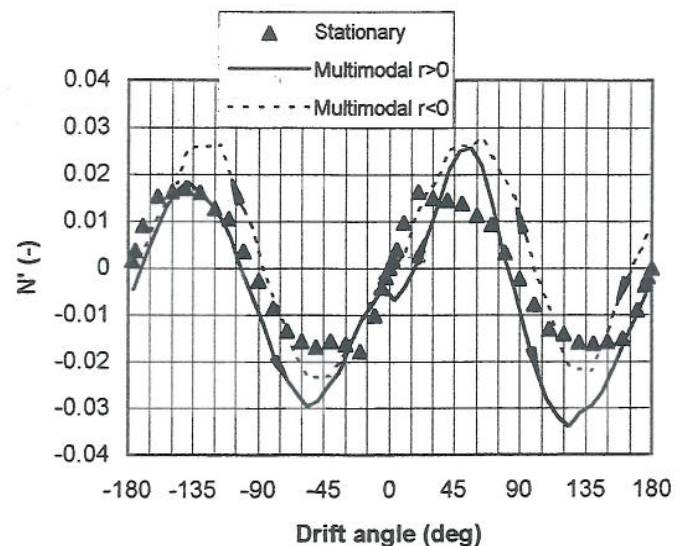
Figure 9: Non-dimensional yawing moment N' measured during stationary oblique towing tests and non-stationary multimodal tests (C2, |r| = 1 deg/s).
