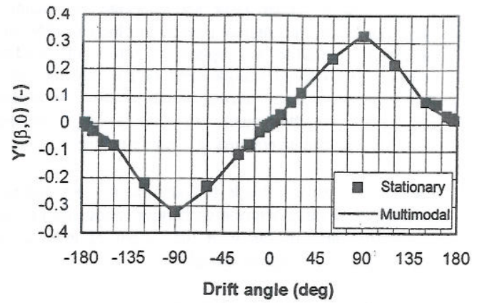
Figure 1: Comparison between the non-dimensional lateral force Y'(\beta, 0) due to drift without propeller action resulting from stationary and multimodal tests (GE).
