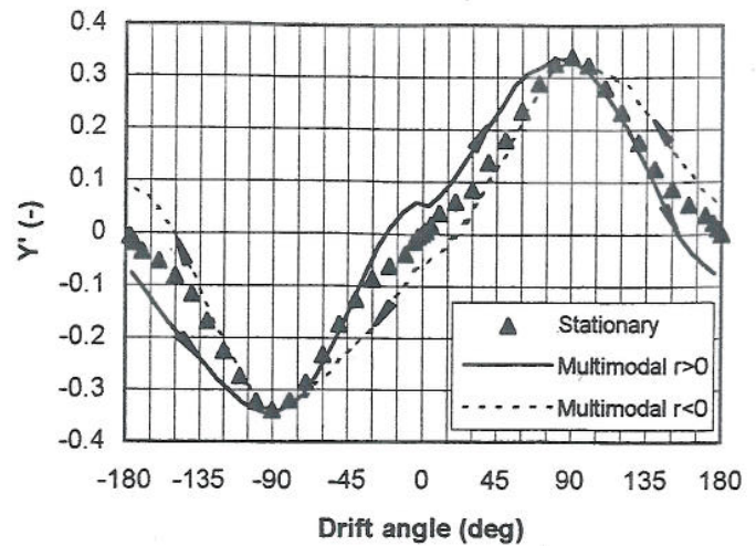
Figure 8: Non-dimensional lateral force Y' measured during stationary oblique towing tests and non-stationary multimodal tests (C2, |r| = 1 deg/s).
