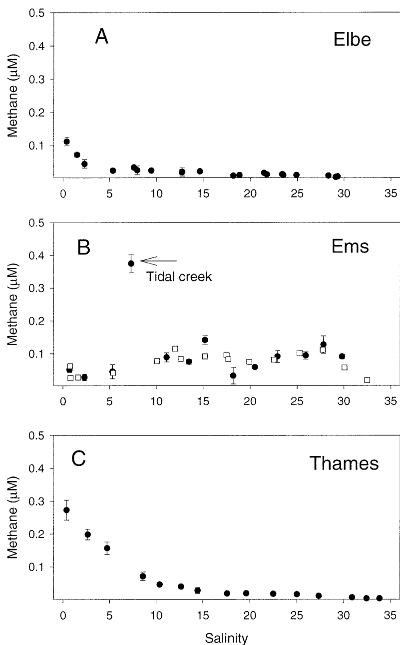
Figure 3. Dissolved methane versus salinity. A: Elbe estuary; B: Ems estuary; C: Thames estuary; D: Loire estuary; E: Douro estuary; F: Sado estuary. Solid symbols: average \pm standard deviation of discrete samples; Open squares: equilibrator-GC-FID data. Notice the difference and breaks in methane concentration scale for the Loire and Sado estuaries. Arrows indicate samples collected in tidal creeks (Ems and Sado).
