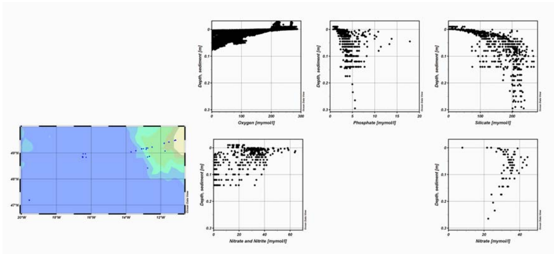
Figure 13: PAP pore water concentration data.
