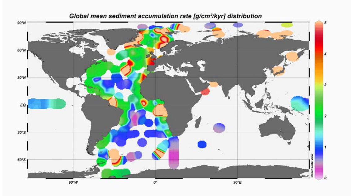
Figure 18: Global solid surface sediment mean accumulation rate (AR) data [ \text{g}/\text{cm}^2/\text{kyr} ].
