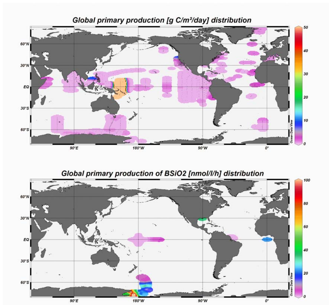
Figure 29: Global distribution of carbon and biogenic silica primary production data in the water column.
