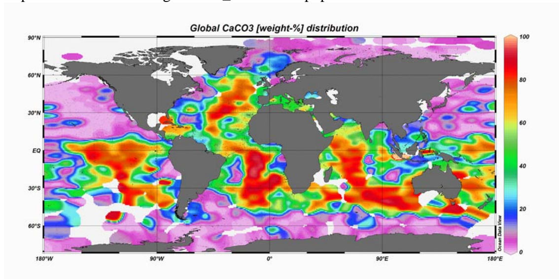
Figure 16: Global solid surface sediment Calcium Carbonate ( \text{CaCO}_3 ; calcite) concentration data [weight-%].
