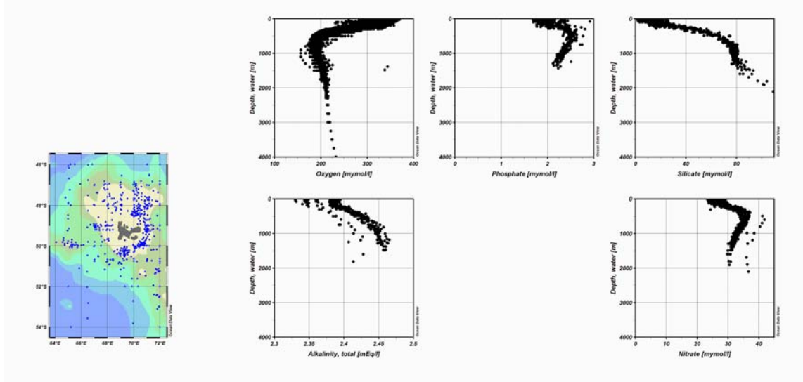
Figure 10: KERFIX water column concentration data.
