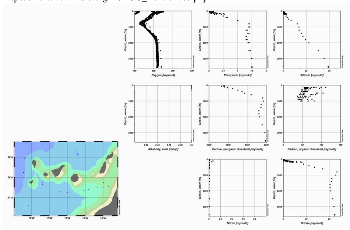
Figure 7: ESTOC water column concentration data.
