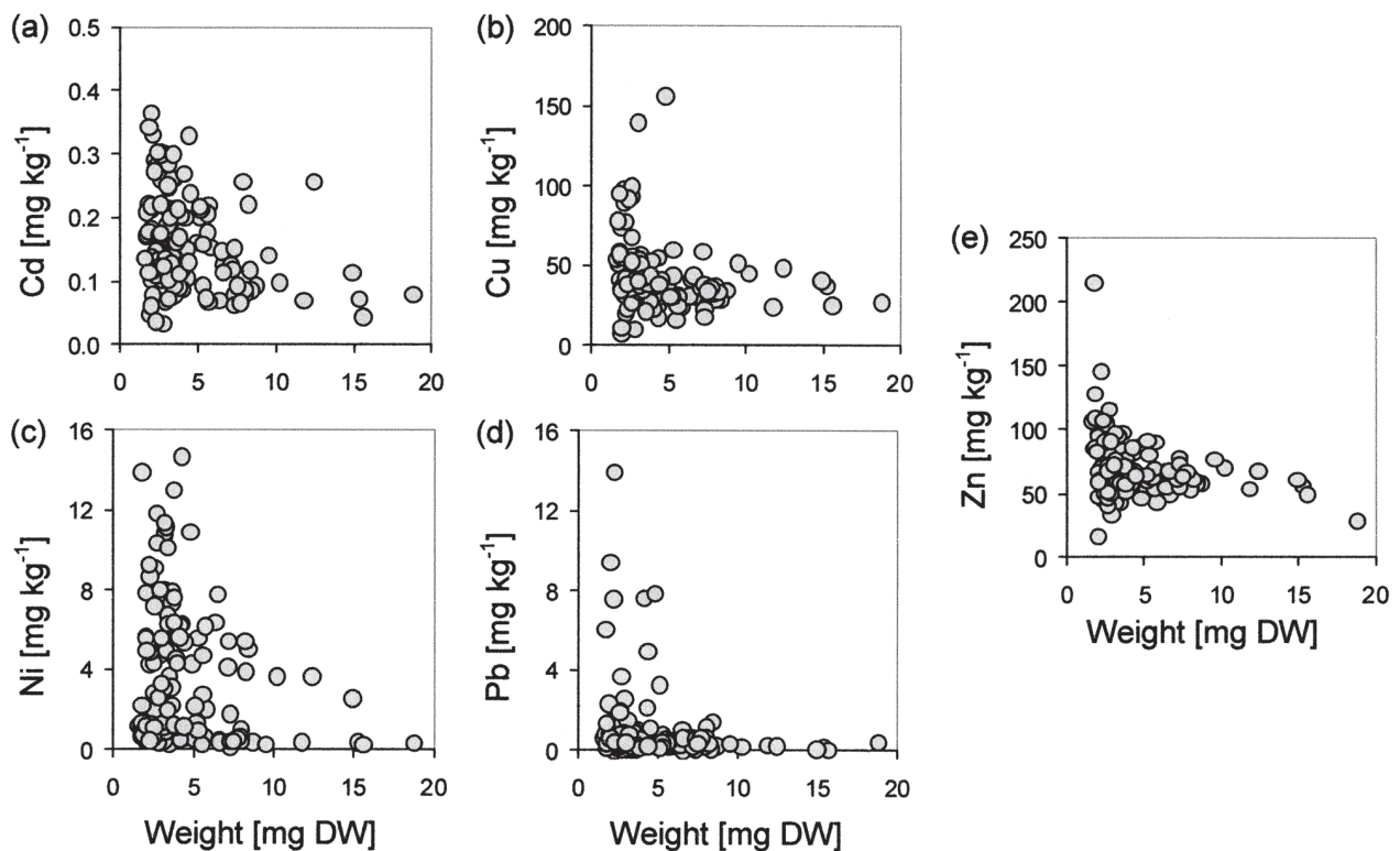
FIG. 5. – Relationships between concentrations of (a) Cd , (b) Cu , (c) Ni , (d) Pb and (e) Zn ( \text{mg kg}^{-1} DW, respectively) and body dry weight (mg) for individually measured Crangon crangon sampled in July 2004 and 2005 in Schillig, German Wadden Sea Coast (Fig. 1).
