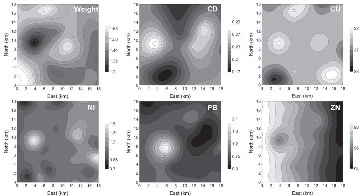
FIG. 4. – Mapped spatial distribution of weight ( mbw = mean body wet weight of shrimps per sample in g), Cd , Cu , Ni , Pb and Zn in Crangon crangon ( \text{mg kg}^{-1} DW, respectively) within Box A (Fig. 1) in universal kriging plots showing contour lines.
