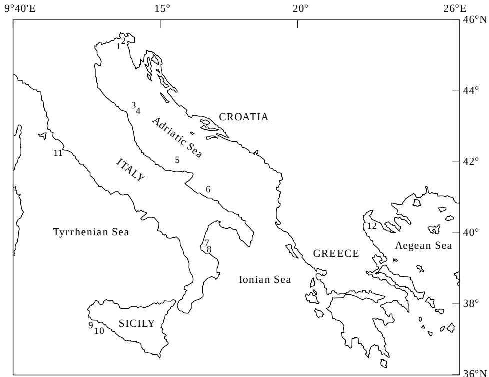
Figure 1. Map of the northern Mediterranean showing sample sites where E. encrasicolus were collected. Sample month + year are given in parentheses. 1: Trieste (5/93), 2: Trieste (9/93), 3: Ancona (5/93), 4: Ancona (9/93), 5: Vieste (4/93), 6: Vieste (9/93), 7: Ionian Sea (5/93), 8: Ionian Sea (7/93), 9: Sicily (4/93), 10: Sicily (7/93), 11: Tyrrhenian Sea (2/94), 12: Aegean Sea (5/94).
