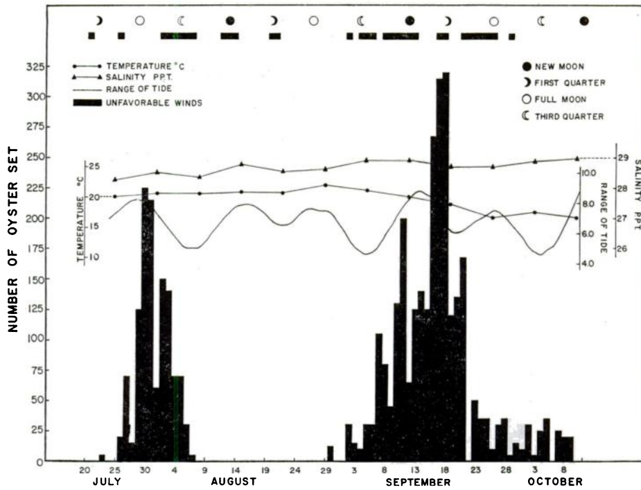
FIGURE 5. Average daily number of oyster set per station recorded in 100 oyster shell-surfaces in Long Island Sound, 1950. Two definite waves of setting, separated by a "dead period," can be seen. Some of the environmental conditions are also shown.
