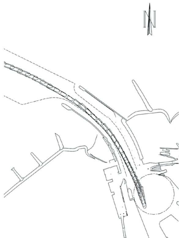
Sailing course plot: vessel entering the port of Ostend
