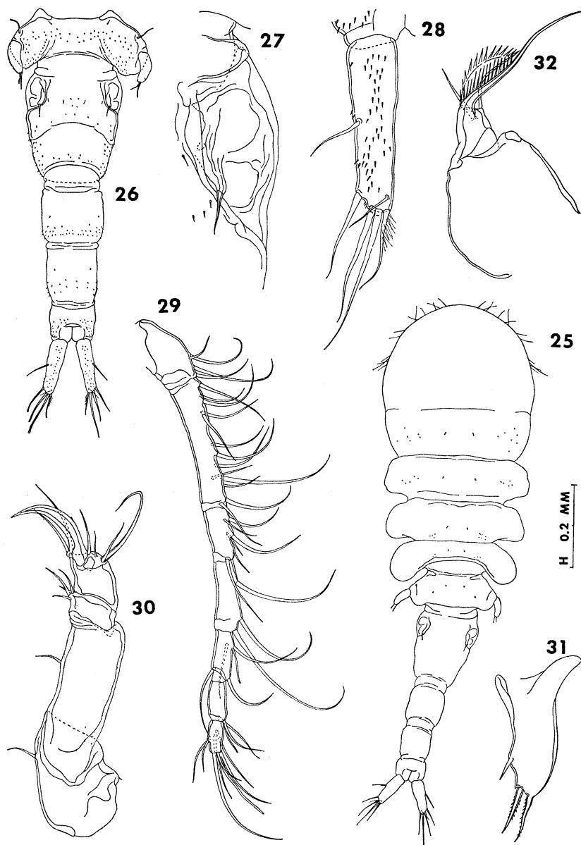
Figs. 25-32. Diogenidium spinulosum Stock, 1968, female. 25, dorsal (A); 26, urosome, dorsal (H); 27, area of attachment of egg sac, dorsal (E); 28, caudal ramus, dorsal (D); 29, first antenna, ventral (D); 30, second antenna, anterior (D); 31, first maxilla, posterior (C); 32, second maxilla, anterior (E).
