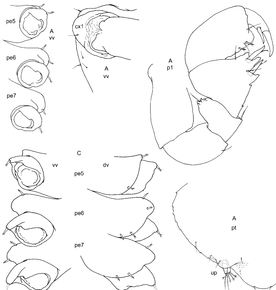
FIGURE 17. Stephenseniellus palliolatipes , sp. nov. A, holotype, male; C, paratype, female C. cx1 , coxa I; dv , dorsal view; p1 , pereopod I; pe5-7 , pereonites 5-7 with coxae; pt , pleotelson; up , uropod; vv , ventral view.
