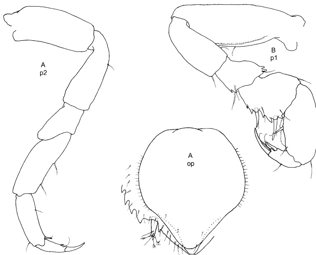
FIGURE 12. Austroananus mawsoni , sp. nov. A, holotype, female; B, paratype, female B. op , operculum; p1, 2 , pereopods I, II.
