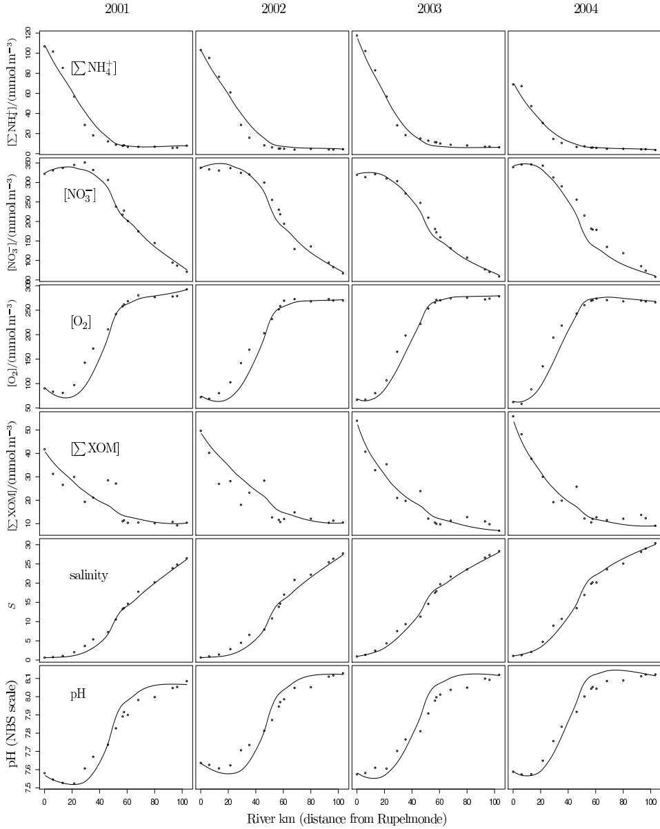
Figure 2.3.: Fit of the biogeochemical model for 4 consecutive years. Calibration was done on data for 2003 only. Data and model output are yearly averages.
