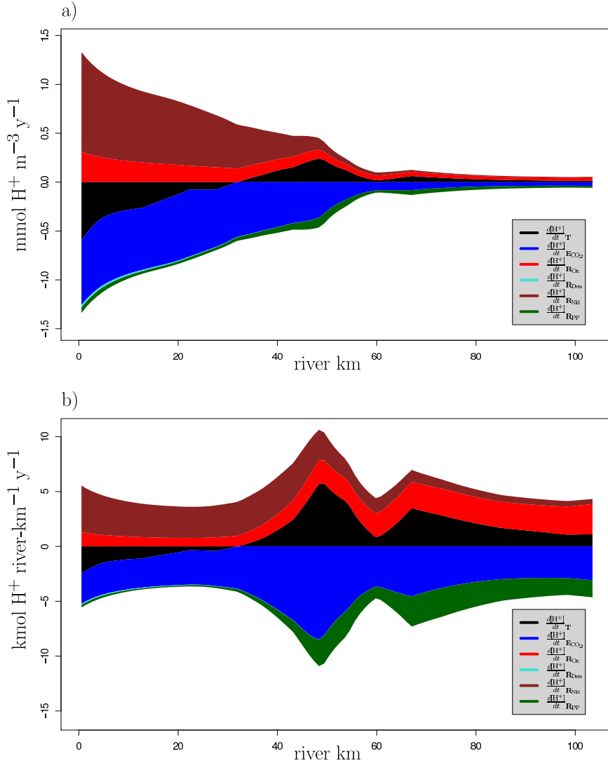
Figure 4.4.: The influences of kinetically modelled processes on the pH – volumetrically and volume integrated.
