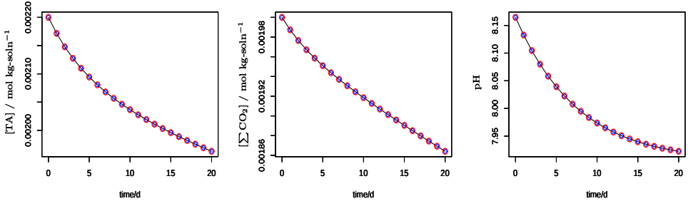
Figure 6.2.: Comparison of the results of the implicit and explicit pH modelling approaches using the function aquaenv . Black line: implicit approach, Blue circles: explicit approach expressing sensitivities of pH with partial derivatives (Eqs. (18) and (19)), Red circles: explicit approach expressing sensitivities of pH using ionization fractions (Eqs. (20) and (21)). Initial values and model parameters are given in the R code in Appendix 6.6.1.1
