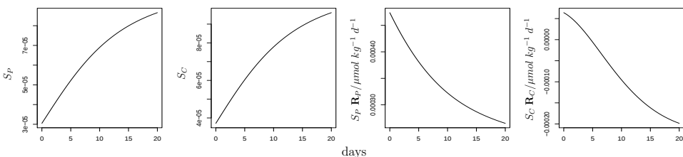
Figure 5.2.: The sensitivities of the pH to calcite precipitation and \text{CO}_2 air-water exchange and the overall influences of both processes on the pH (i.e., the product of their rate and the respective sensitivity of the pH) in the example system over the course of 20 days. The sensitivities are dimensionless quantities. The consistency between the explicit and the implicit pH modelling approach has been confirmed for the given example model: the obtained temporal pH profiles are identical.
