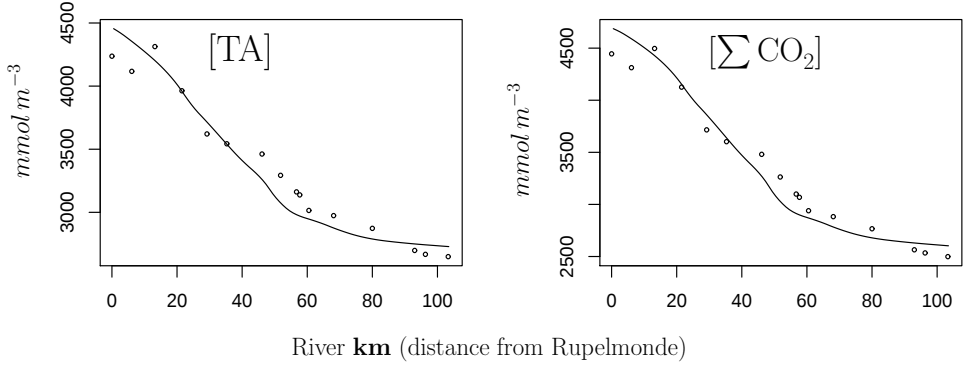
Figure 2.4.: Yearly averaged [TA] and [\Sigma CO_2] (model output, 2003) vs. field data provided by Frederic Gazeau (personal communication and Gazeau et al., 2005 ). [TA] data are measurements, [\Sigma CO_2] data are consistently calculated using conditions of the model.
