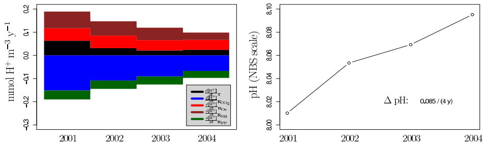
Figure 4.6.: Trends in pH and the influences of major kinetically modelled processes on [\text{H}^+] from 2001 to 2004.
