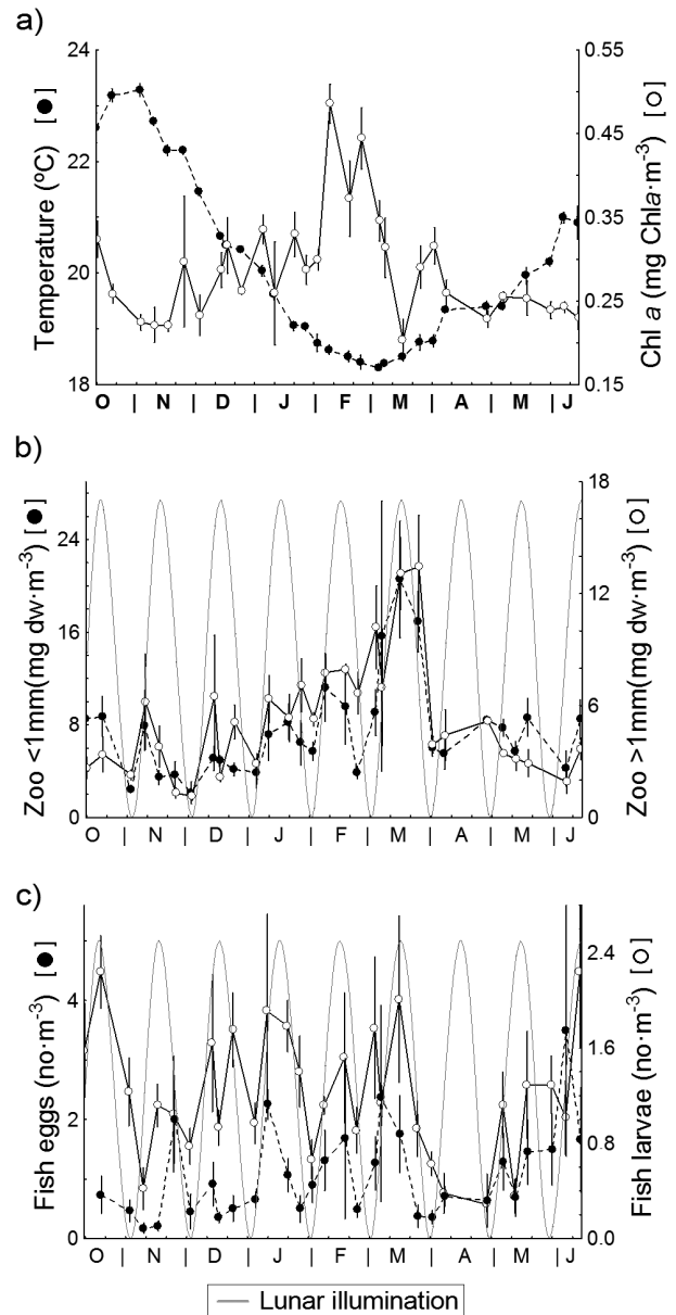
FIG. 3. – Temporal distribution of a ) average temperature in the mixed layer (°C) and average chlorophyll a (mg chl a ·m -3 ), b ) Size fractionated mesozooplankton biomass (mg dry weight·m -3 ), c ) concentration of fish eggs (no.eggs·m -3 ) and fish larvae (no.larvae·m -3 ). Average values for the five sampling stations are shown. Note that lunar illumination is plotted as a fine grey line in the background for 3b and 3c.
