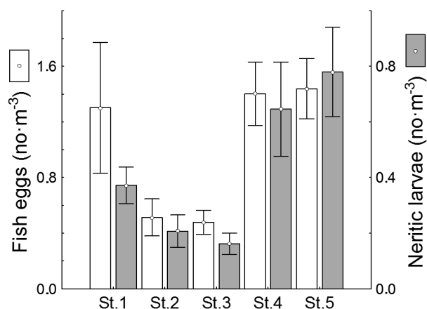
FIG. 5. – Average abundance (no·m -3 ) and standard error (SE) along the five sampling stations of total fish eggs (white bars) and neritic larvae (grey bars).
