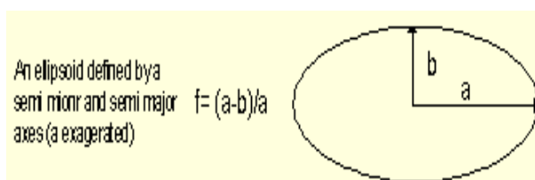
Figure5 - 18 (a), Semi-major axis (b) Semi-minor axis
