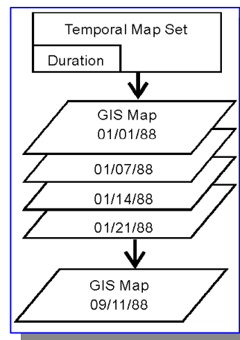
Figure 7- 1: TMS Model (after Beller et, 1991)
