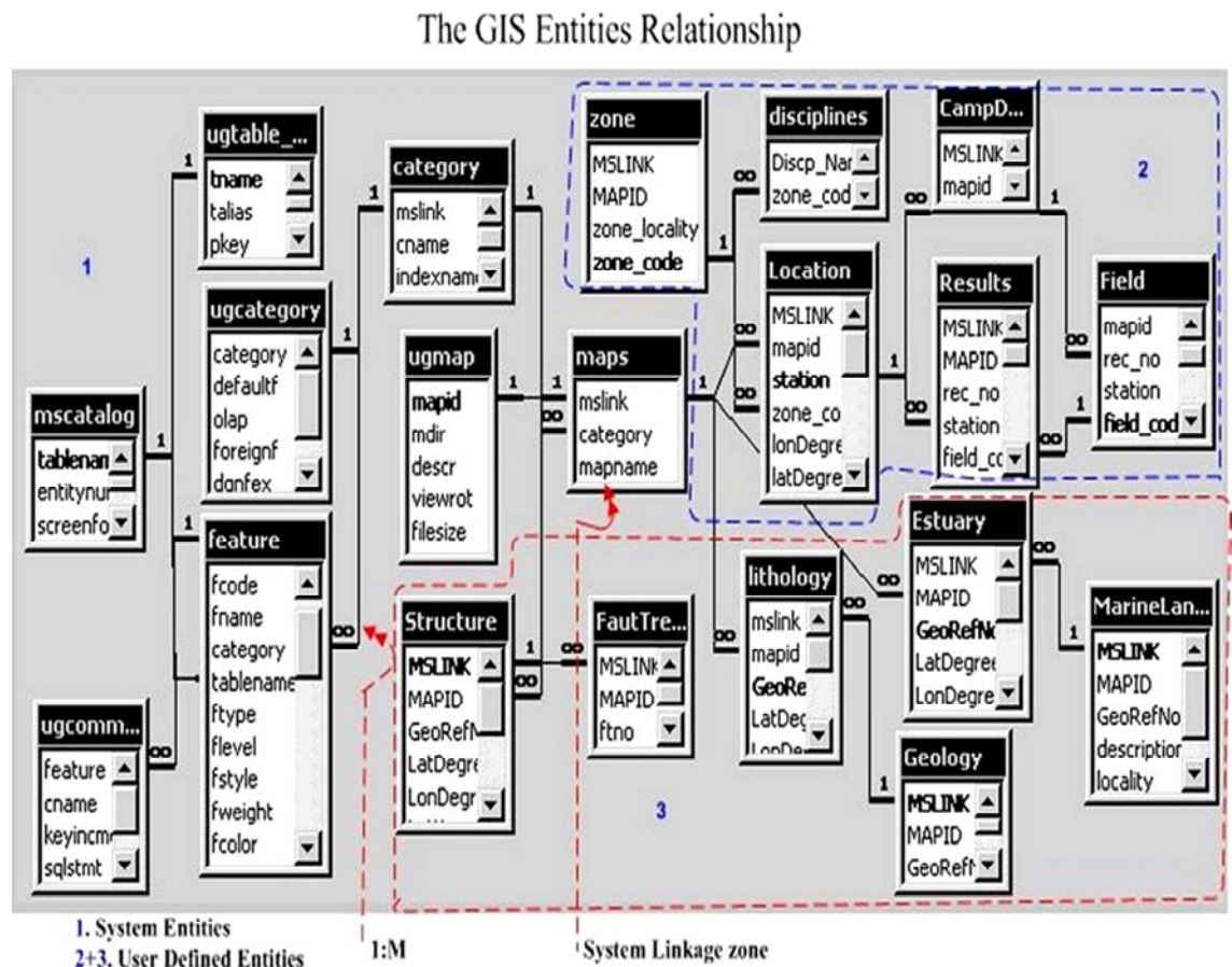
Figure 3-11 Integrated GIS Database
