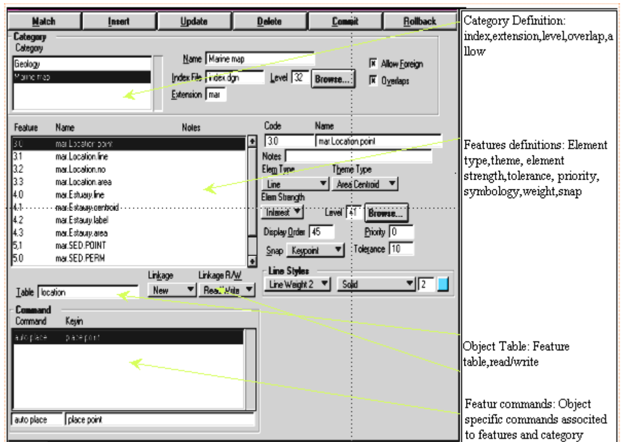
Figure 3-8 Categories and Features Definitions (Geographic GIS)
