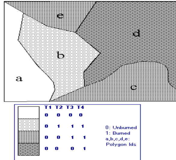
Figure 7- 2: An example of an STC layer for burns (Modified from Lnagan and Chrisman, 1988)
