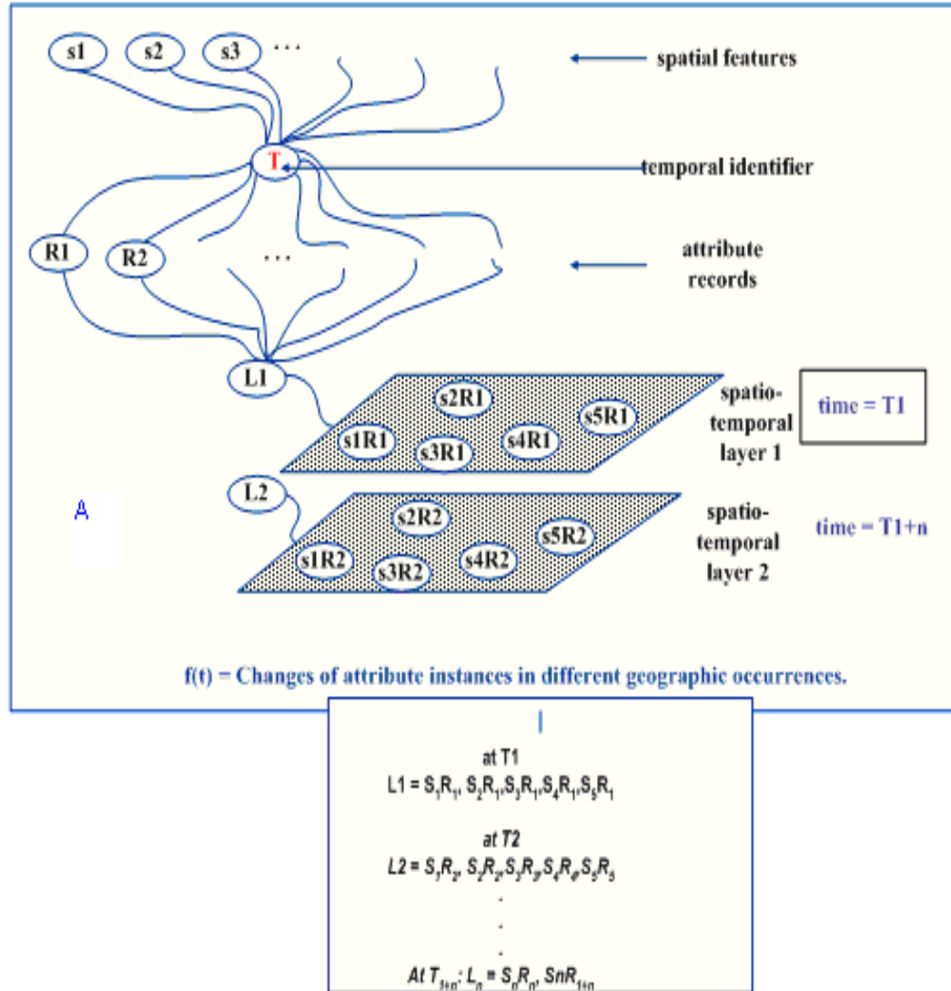
Figure 7- 5: (A) Multiple Spatial Objects at Time1 (t1) (B) Changes R to R1+1 in S1 as F (t)
