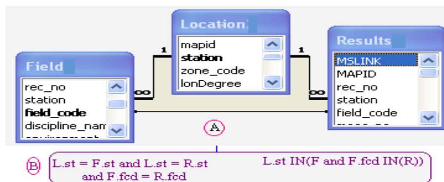
Figure 8-1 Tir-Table Information Extraction on a defined Relationship
