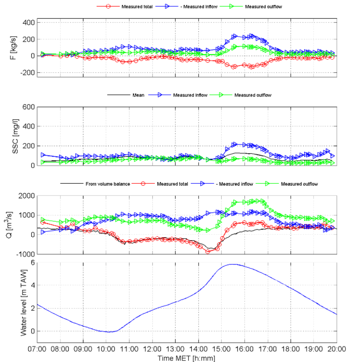
Figure 5-1 Total in/out/net flux, Total incoming/outgoing SSC, average in/out/net discharge and water level at DGD on March 8th 2012.
