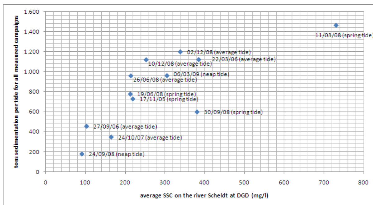
Figure 5-9: Overview of measured sediment deposition in Deurganckdok per tide by means of Sediview technique compared to average SSC on the river Scheldt.
