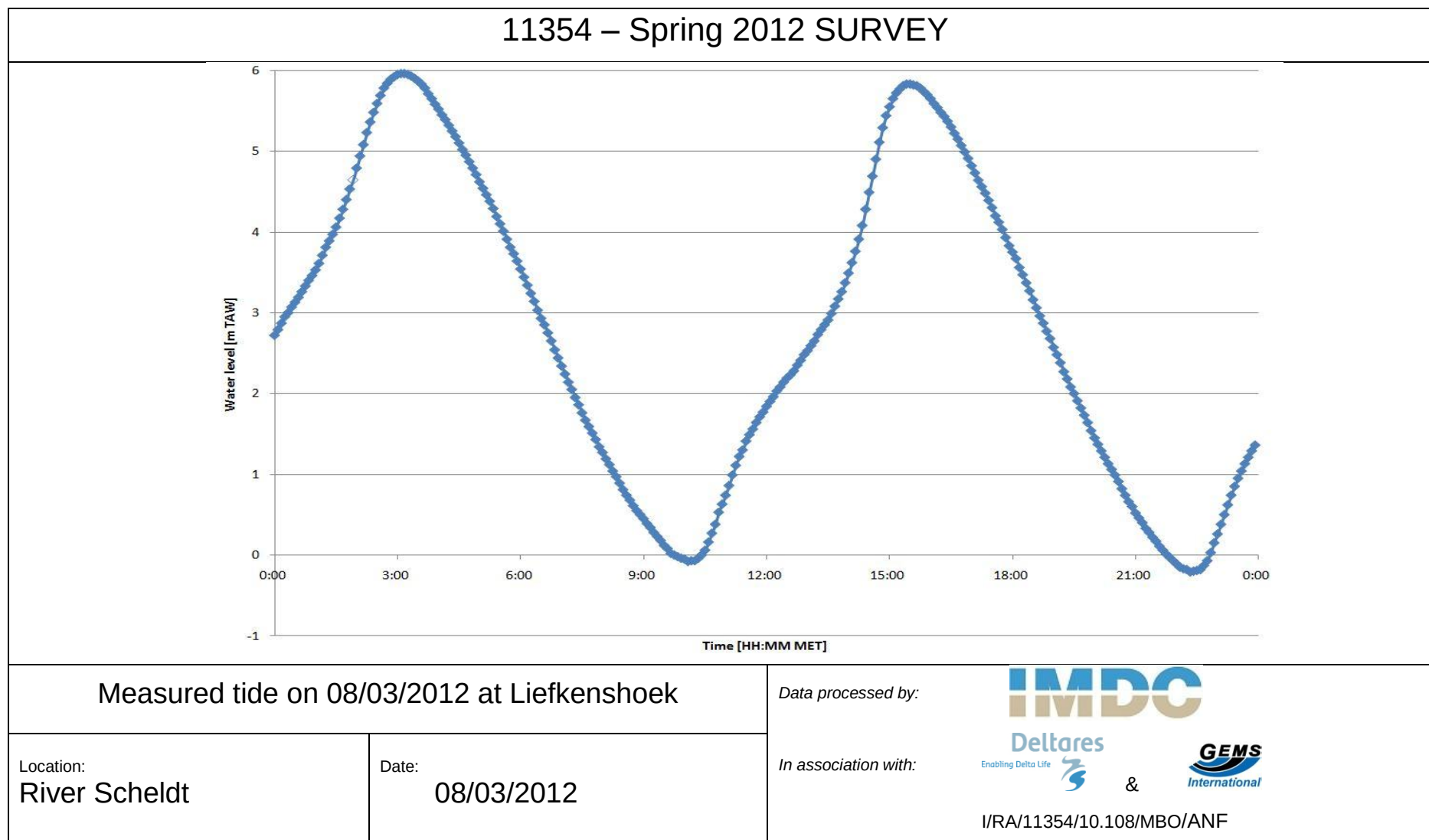
Annex Figure 5: Measured tide in MET on 8 March 2012 at Liefkenshoek
