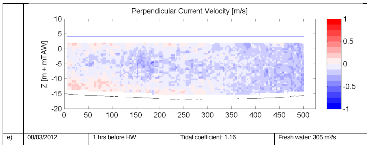
Figure 5-5: Perpendicular current velocity at 1hr before high water
