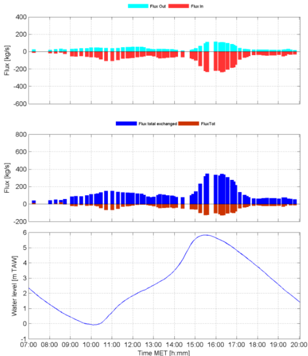
Figure 5-8: The sediment flux at the entrance of Deurganckdok on 08/03/2012 (negative values represent incoming sediment). Top: Total incoming (flux in) and outgoing sediment flux (flux out); Central: total sediment exchange versus total sediment flux; below: tidal curve
