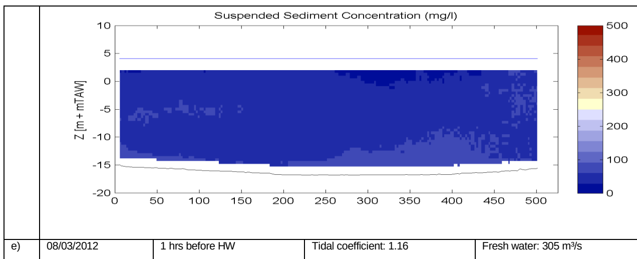
Figure 5-6: Suspended sediment concentration at 1hr before high water
