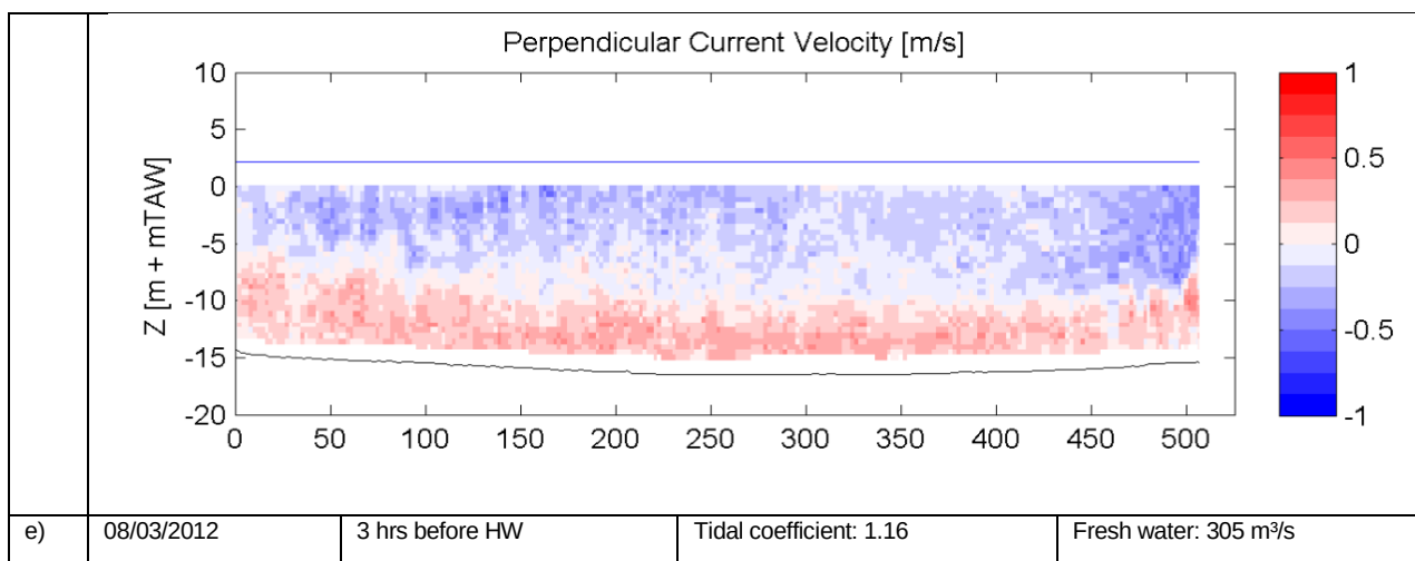
Figure 5-3: Perpendicular current velocity at 3hrs before high water during spring measurements
