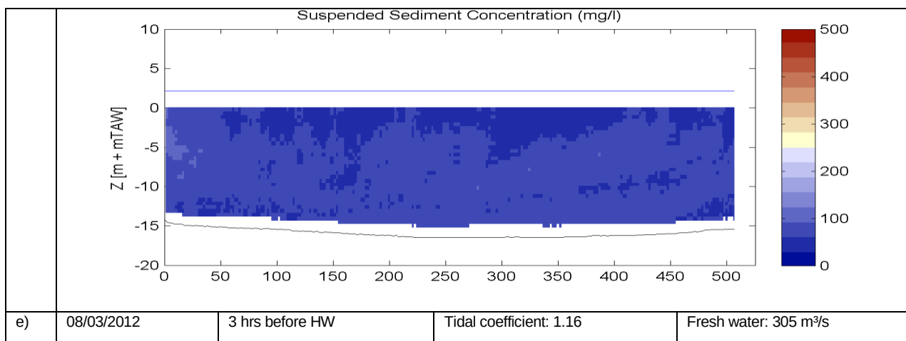
Figure 5-4: Suspended sediment concentration at 3hrs before high water
