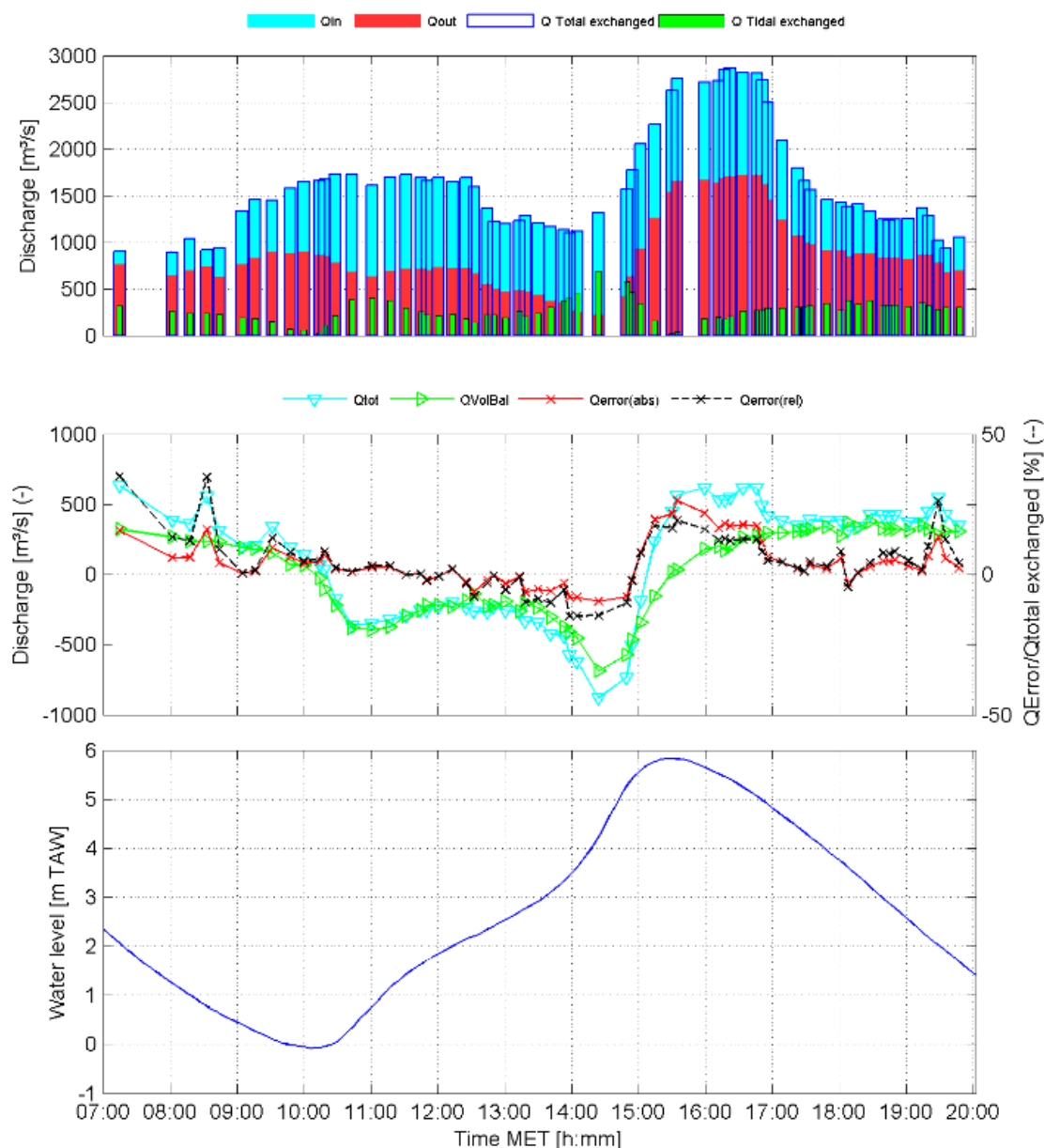
Figure 5-7: The water discharge at the entrance of Deurganckdok over a tidal curve on 08/03/2012. Top: Total incoming ( Q_{in} ) and outgoing ( Q_{out} ) discharge including the total water en tidal exchange; Central: Measured residual discharge ( Q_{tot} ) versus theoretical residual discharge ( Q_{VolBal} ) and correction offset ( Q_{error} ) including relative error; Below: tidal curve.
