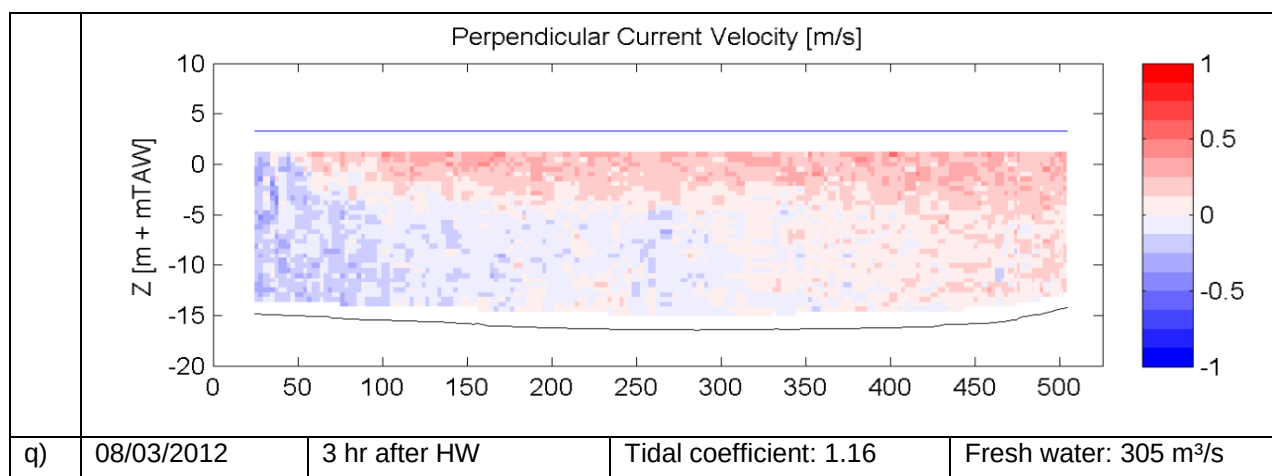
Annex Figure 11: Perpendicular current velocity at 3h after high water
