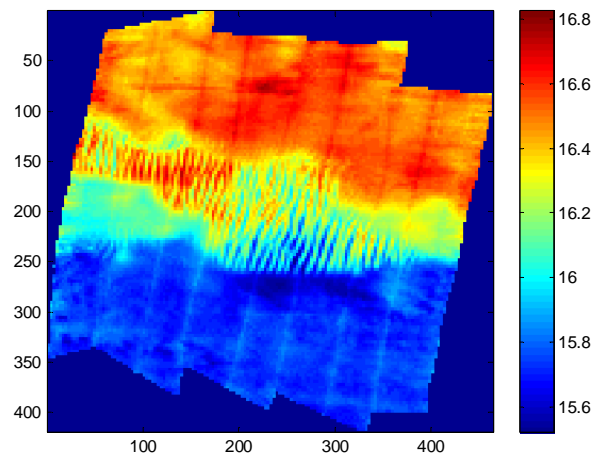
Figure 13. Test section in channel Scheur Oost : average values of the multi-beam soundings per grid cell of 3*3 m 2 (avg3avg1). Horizontal and vertical scale: distance (m, north up); colour scale: depth (m) referred to LAT.
