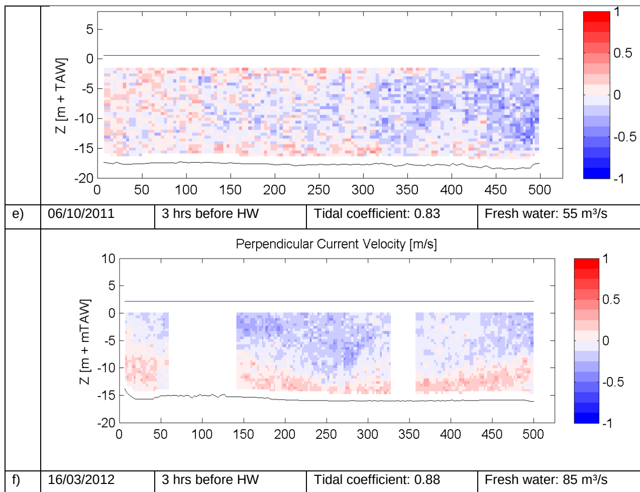
Figure 5-3: Perpendicular current velocity at 3hrs before high water
