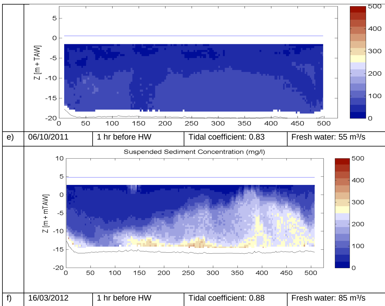
Figure 5-6: Suspended sediment concentration at 1hr before high water
