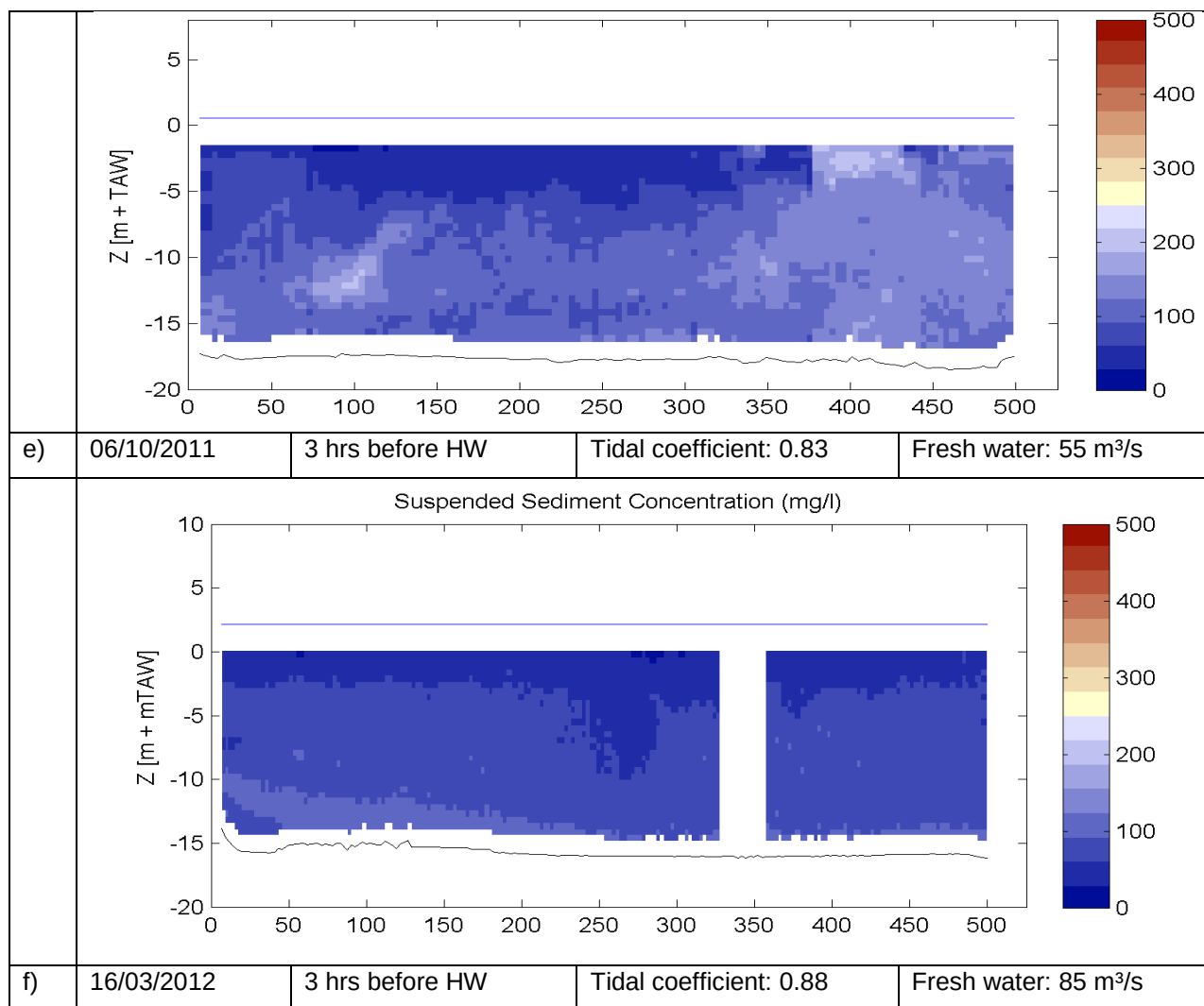
Figure 5-4: Suspended sediment concentration at 3hrs before high water
