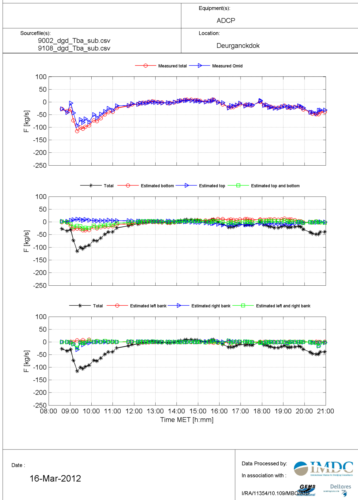
Annex Figure 9: Total flux through the measured cross section, positive is from dock to river
