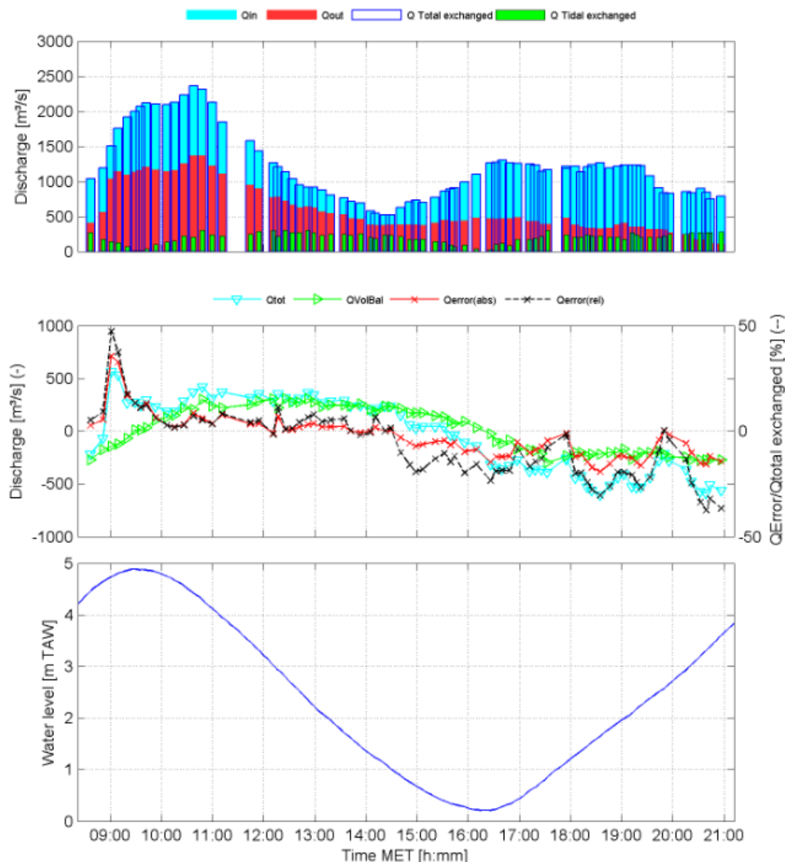
Figure 5-7: The water discharge at the entrance of Deurganckdok over a tidal curve on 16/03/2012. Top: Total incoming ( Q_{in} ) and outgoing ( Q_{out} ) discharge including the total water en tidal exchange; Central: Measured residual discharge ( Q_{tot} ) versus theoretical residual discharge ( Q_{VolBal} ) and correction offset ( Q_{error} ) including relative error; Below: tidal curve.
