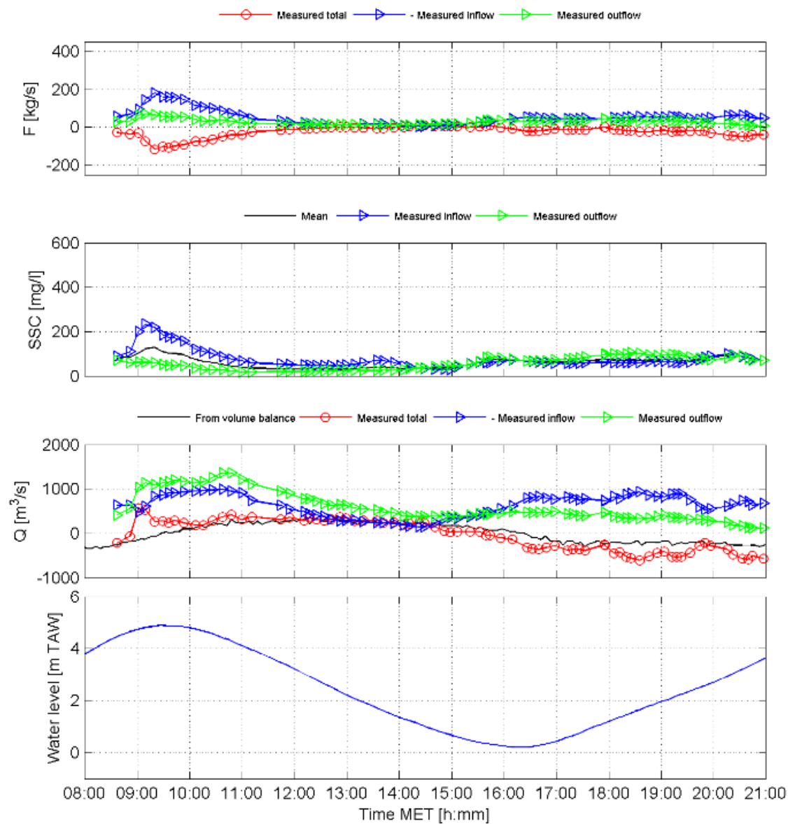
Figure 5-1 Total in/out/net flux, Total incoming/outgoing SSC, average in/out/net discharge and water level at DGD on March 16th 2012.
