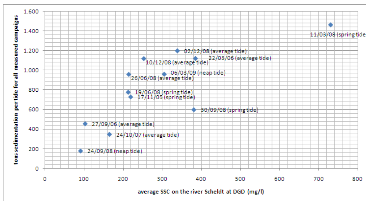
Figure 5-9 Overview of measured sediment deposition in Deurganckdock per tide by means of Sediview technique compared to average SSC on the river Scheldt.
