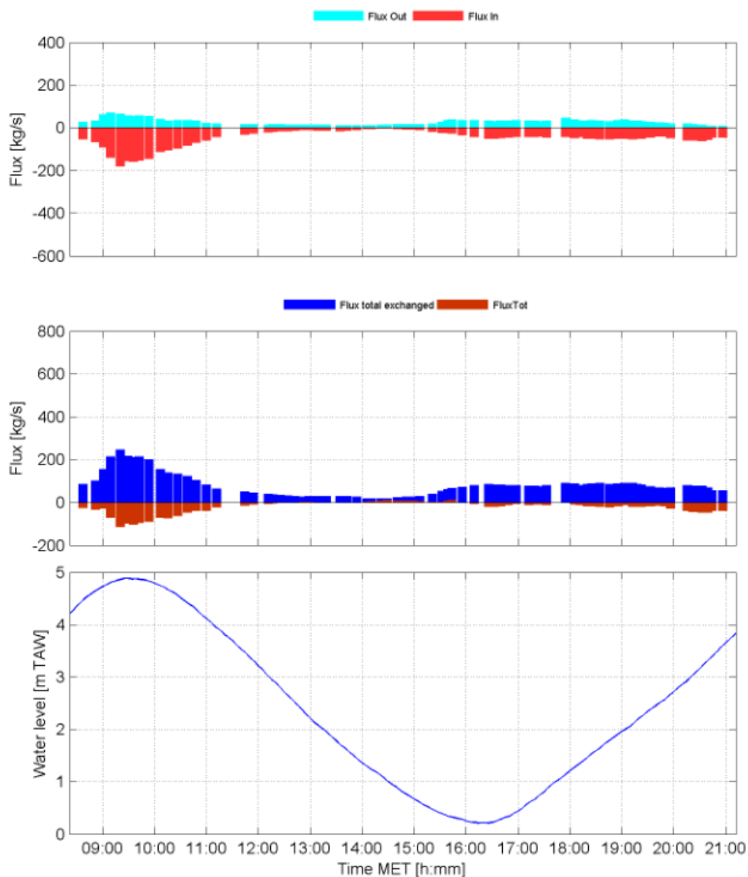
Figure 5-8: The sediment flux at the entrance of Deurganckdok on 16/03/2012 (negative values represent incoming sediment). Top: Total incoming (flux in) and outgoing sediment flux (flux out); Central: total sediment exchange versus total sediment flux; below: tidal curve
