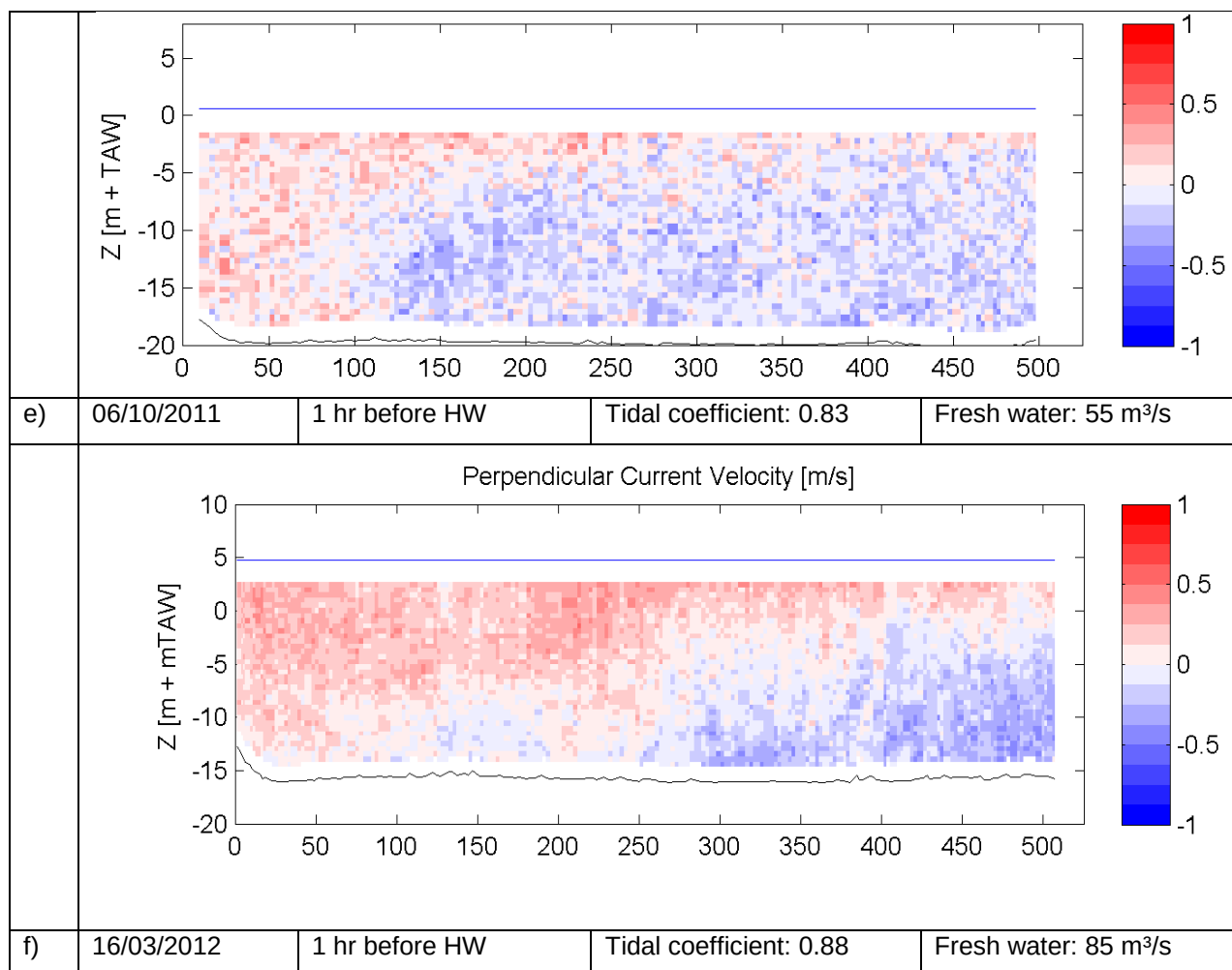
Figure 5-5: Perpendicular current velocity at 1hr before high water
