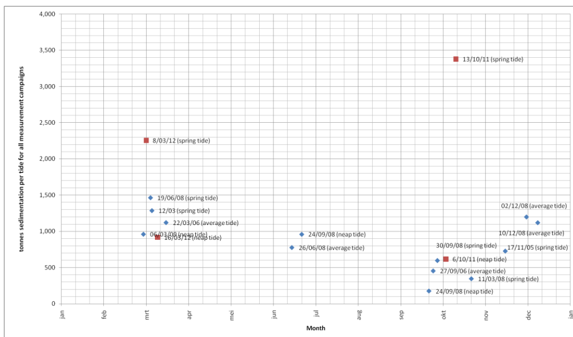
Figure 5-10: Evolution of the measured sediment deposition in Deurganckdok per tide by means of Sediview technique (blue dots: without CDW/with sill; red squares: with CDW/ without sill).
