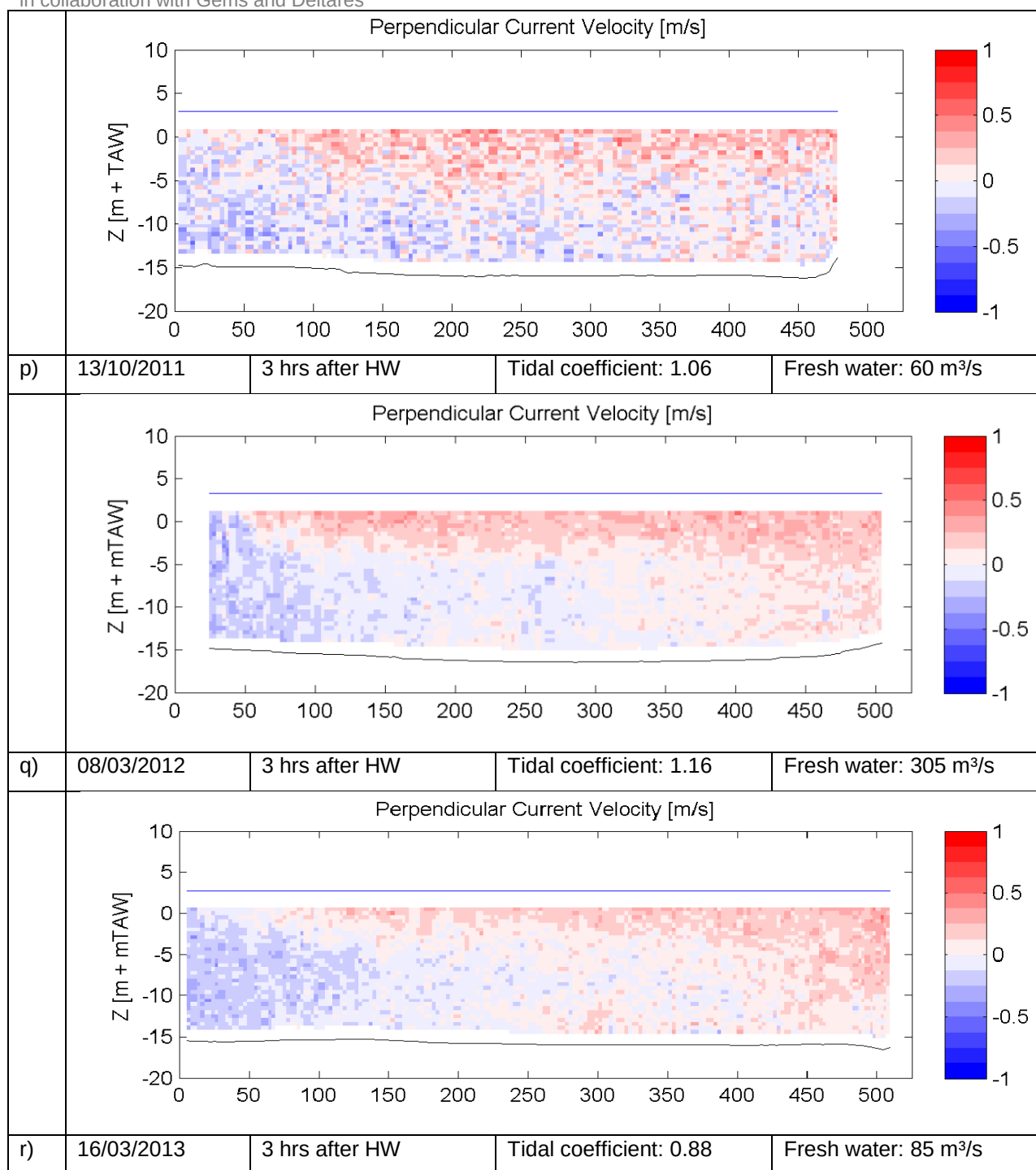
Annex Figure 11: Perpendicular current velocity at 3h after high water
