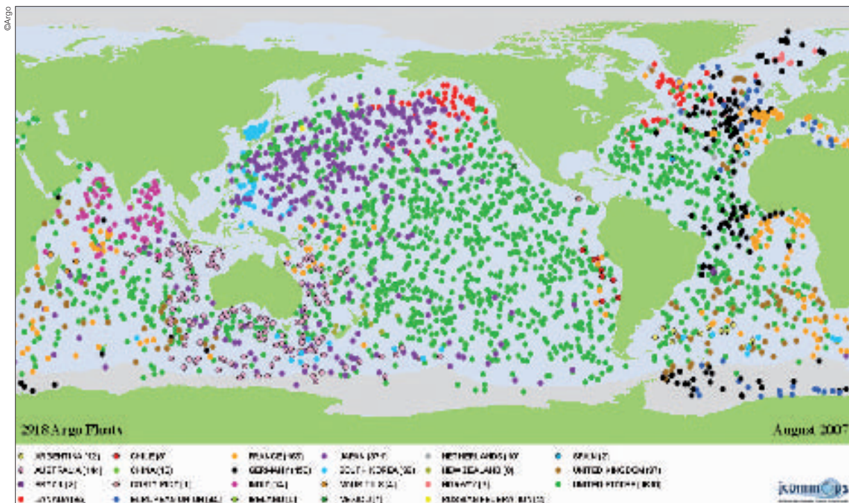
Figure 7. Global distribution of Argo profiling floats
