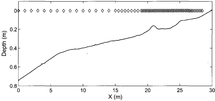
Figure 5.4: Setup of the Boers (1996) flume experiment, showing the depth profile of a barred beach and the wave gauge positions (diamonds).
