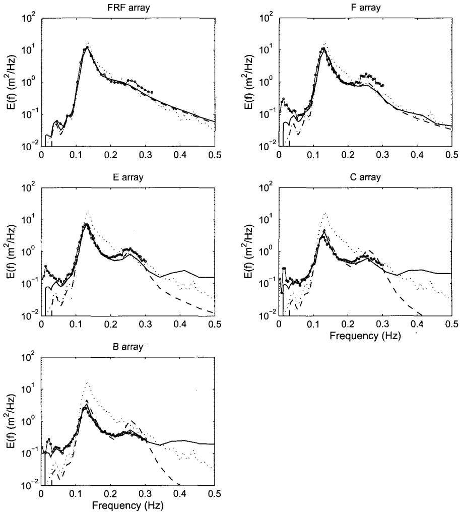
Figure 5.24: Comparison between simulated and observed frequency spectra, for Sandy-Duck '97 event of 13/11/1997 at 19:00. Simulation including both shallow and deep water source terms, but with quadruplet interaction (DIA) only active for Ur < 0.1 . Shown are the results of the LTA model (dashed line), the two-equation model (solid line) and observations (line with circles). Input spectrum at the WR630 buoy indicated by dotted line.
