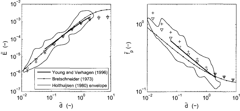
Figure 4.10: Depth-limited growth curves produced by the saturation-based model (inverted triangles) and the default model (plusses). Observations as indicated. Results for U_{10} = 10 m/s.
