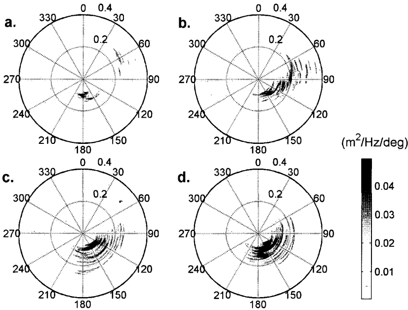
Figure 4.17: Directional spectra observed at the waverider buoy D. Observations shown at nine-hourly intervals: (a) 11/10/2004 at 17h30, (b) 12/10/2004 at 02h30, (c) 12/10/2004 at 11h30 and (d) 12/10/2004 at 20h30.
