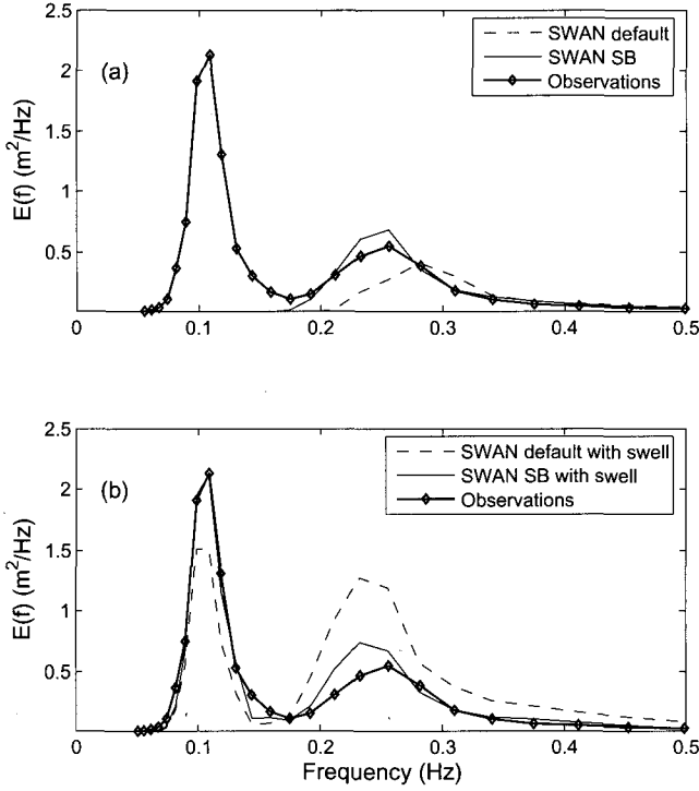
Figure 4.14: Results of simulations over the North Carolina shelf at downwind Station X3. (a) Spectra of the saturation-based and default models in simulations without swell. (b) Corresponding results of simulations with ambient swell. Average wind speed is U_{10} = 9.5 m/s.
