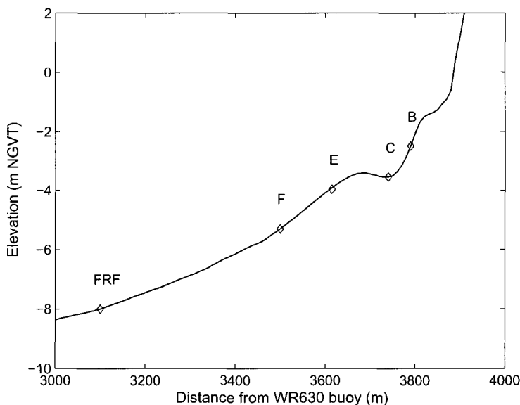
Figure 5.14: Profile of the barred beach at Duck, measured on 97/10/30, showing the locations of the nearshore arrays.
