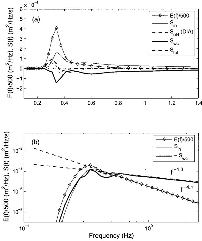
Figure 4.8: Source terms produced by the saturation-based model using the DIA quadruplet method. Panel (a): variance spectrum and all source terms on a linear scale, panel (b): variance spectrum and source terms of wind input and dissipation (absolute value) on logarithmic axes, with power law fits (dashed lines). Result for deep water, fetch-limited growth simulations with U_{10} = 10 m/s, at a fetch of X^* = 7 \times 10^5 .
