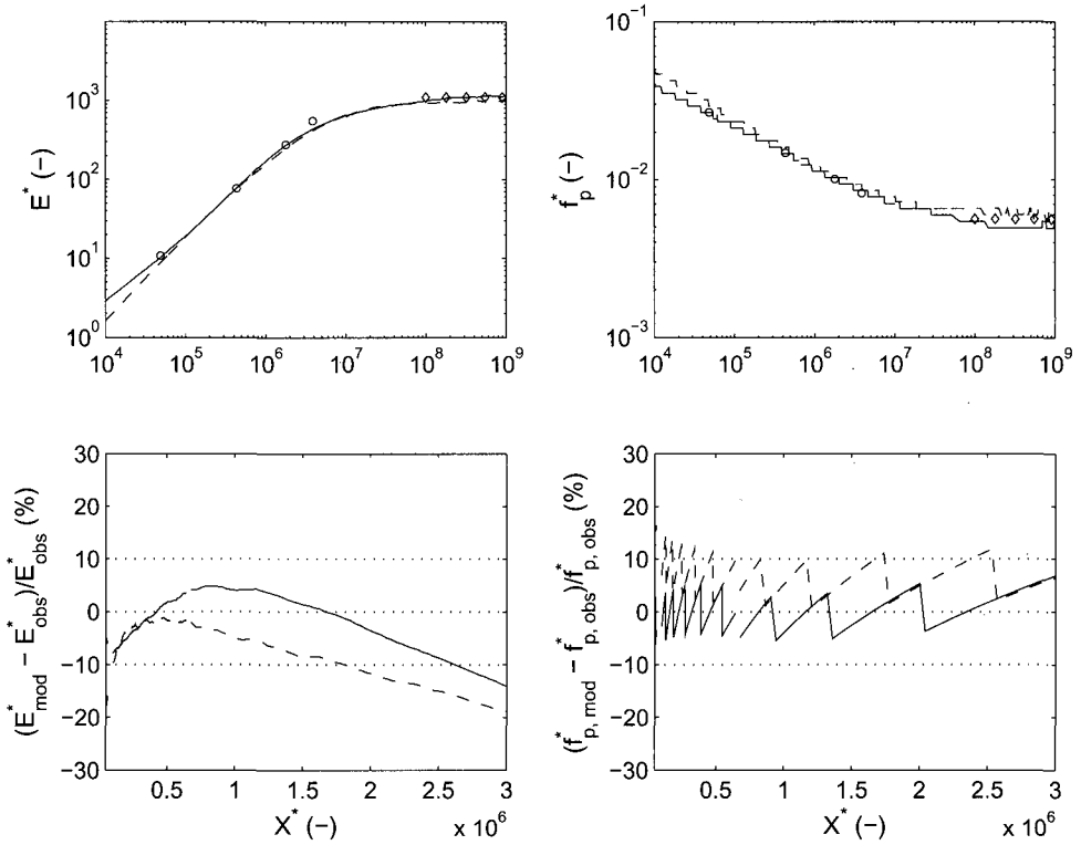
Figure 4.7: Deep water, fetch-limited growth curves produced by the saturation-based model (solid lines) and the default model (dashed lines), both using the DIA quadruplet method. Top panels: comparison with fetch-limited relations of Kahma and Calkoen (1992) (circles) and Pierson and Moskowitz (1964) (diamonds). Bottom panels: bias of model results with respect to Kahma and Calkoen (1992) data. Results for U_{10} = 10 \text{ m/s} .
