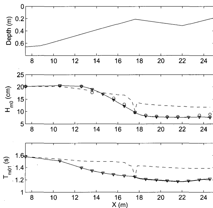
Figure 3.13: Spatial development of wave height and period during the iteration process of a case from the laboratory experiment of Battjes and Janssen (1978). Top panel: Depth profile of the experiment. Middle and lower panels: Simulation results obtained with the setting \alpha = 0.0 and \gamma = 0.1 after 50 iterations (dashed) and 1200 iterations (solid with plusses), and those obtained with \alpha = 0.0 and \gamma = \infty upon convergence (after about 25 iterations, solid with triangles). Note: all plusses virtually coincide with the triangles and for that reason are not separately visible. Observations indicated by circles.
