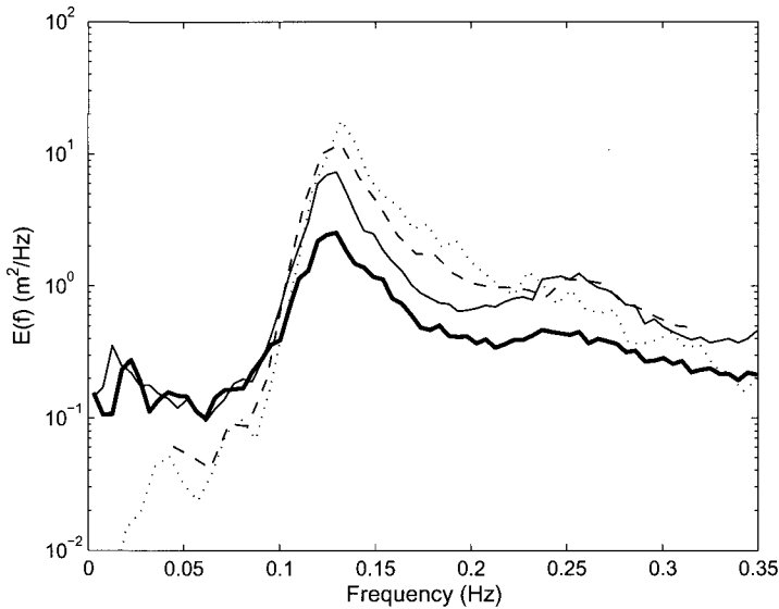
Figure 5.15: Frequency spectra observed during the SandyDuck '97 field experiment on 13/11/1997 at 19:00. Shown are the spectra offshore at the WR630 buoy (dots), at the FRF Array (dash), the E Array (thin solid line) and the B Array (thick solid line).
