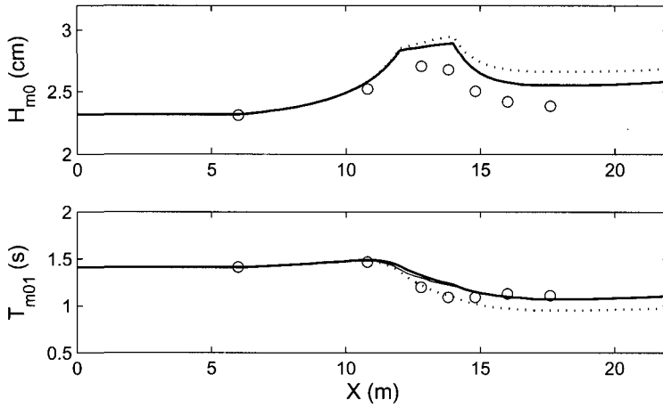
Figure 5.3: Comparison between significant wave height and mean period produced using the LTA and laboratory observations of Beji and Battjes (1993). Simulation results with parameter combinations (a) \alpha_{EB} = 0.1 and f_{max,EB} = 2.2f_{m01} (thin solid line), (b) \alpha_{EB} = 0.1 and f_{max,EB} = 2.5f_{m01} (dotted line) and (c) \alpha_{EB} = 0.05 and f_{max,EB} = 2.5f_{m01} (thick solid line) are shown. Observations are indicated by circles.
