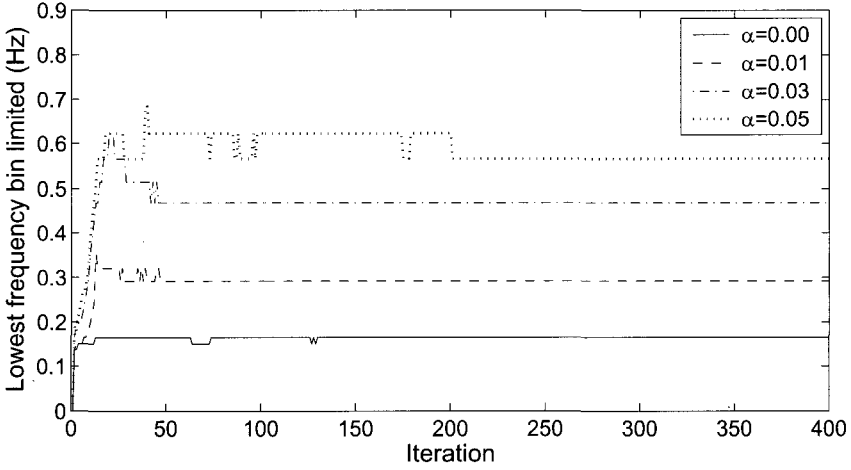
Figure 3.3: Lowest frequency bin at which limiter is active, as a function of iteration level. Results for deep-water, fetch-limited simulations for wind speeds U_{10} = 10 m/s (top panel) and 30 m/s (bottom panel), with \gamma = 0.1 and \alpha = 0.0 –0.05.
