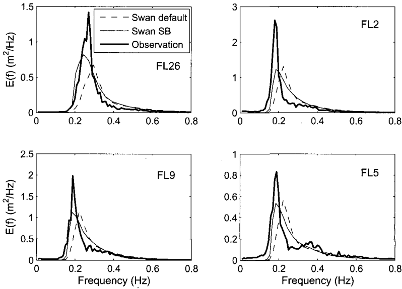
Figure 4.24: Simulated spectra at four observation points in Lake IJssel for case Y-B. Wind speed U_{10} = 23.8 m/s and direction 249^\circ (WSW). Compared are the simulation results of the saturation-based and default models, and observations.
