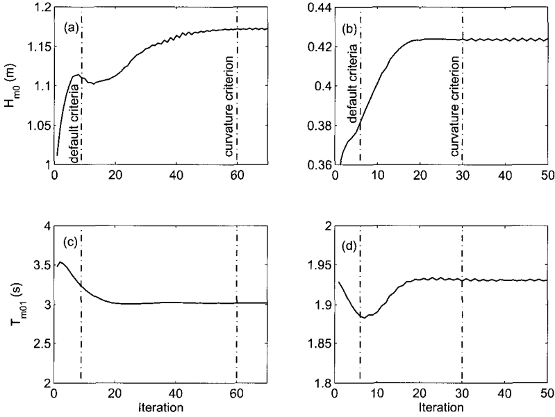
Figure 3.16: Iteration behaviour and location of break-off points for a field case from the Haringvliet Estuary (left hand panels) and from Lake George (right-hand panels). Shown are the positions of run termination using the default stopping criteria (3.5) and (3.6) with \varepsilon_H^r = \varepsilon_T^r = 0.02 , \varepsilon_H^a = 0.02 m and \varepsilon_T^a = 0.2 s (after 6 iterations) and criteria (3.5), (3.6) and (3.9) with \varepsilon_C = 2e-4 (after 30 iterations).
