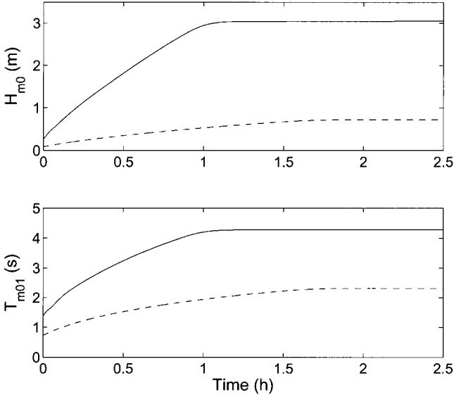
Figure 3.1: Deep-water, fetch-limited wave growth for wind speeds of U_{10} = 10 m/s (dashed line) and 30 m/s (solid), at fetch = 12.5 km. Results for nonstationary SWAN with \Delta t = 1 s and no limiter.
