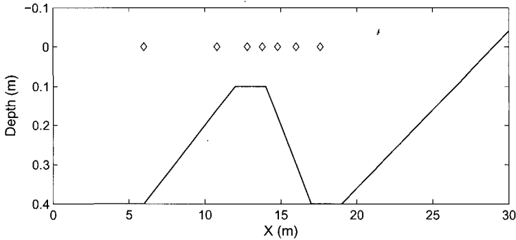
Figure 5.1: Setup of the Beji and Battjes (1993) flume experiment, showing the bottom profile and wave gauge positions (diamonds).
