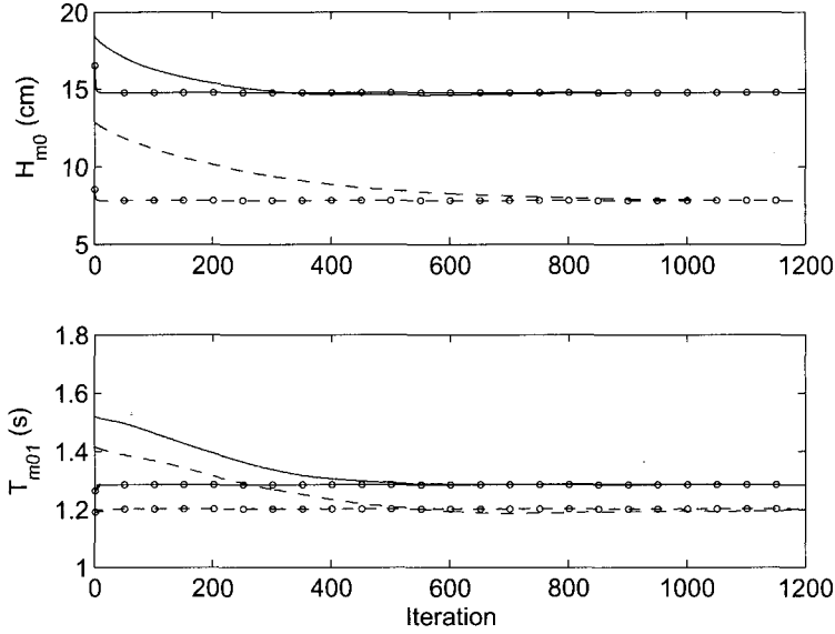
Figure 3.14: Iteration behaviour of wave height and period during the simulation of a case from the laboratory experiment of Battjes and Janssen (1978). Shown are the results obtained with the setting \alpha = 0.0 and \gamma = 0.1 at x = 15.6 m (solid) and x = 23.6 m (dashed), and those obtained with \alpha = 0.0 and \gamma = \infty at the same locations (solid and dashed respectively, with circles).
