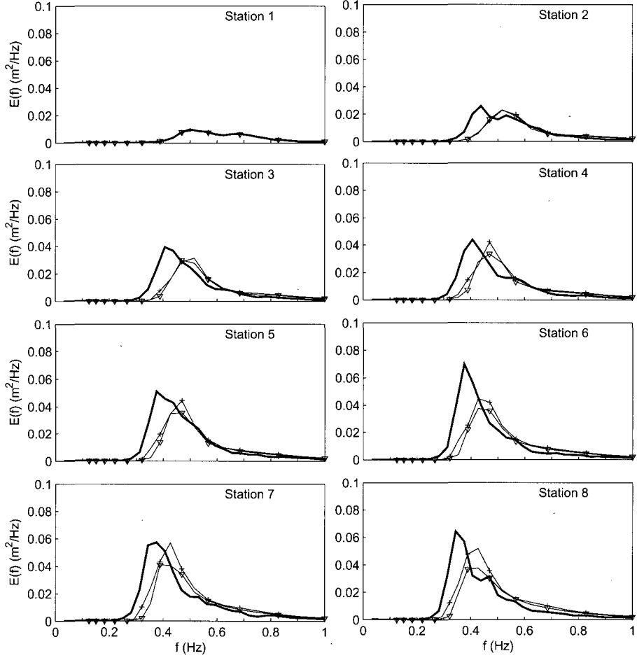
Figure 3.18: Lake George field experiment of near-idealised, depth-limited wave growth. Frequency spectra obtained with the default stopping criteria (3.5) and (3.6) with \varepsilon_H^T = \varepsilon_T^T = 0.02 , \varepsilon_H^a = 0.02 m and \varepsilon_T^a = 0.2 s (6 iterations; triangles), with the criteria (3.5), (3.6) and (3.9) with \varepsilon_C = 2e-4 (30 iterations; plusses) and observations of Young and Verhagen (1996) (thick line).
