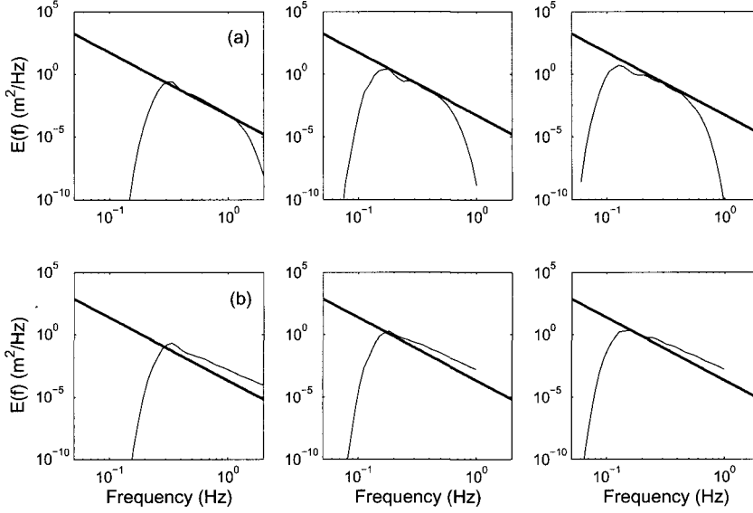
Figure 4.6: Comparison between frequency spectra produced during deep water fetch-limited wave growth and the level of the saturation threshold. Row (a): Spectra produced using Alves and Banner (2003) with the calibration BYM1, featuring a threshold level of B_r = 4.25 \times 10^{-3} , in combination with the DIA. Row (b): Corresponding results for the saturation-based model (4.11) and (4.15) with threshold level of B_r = 1.75 \times 10^{-3} . Results for X^* = 7 \times 10^4 (left), X^* = 7 \times 10^5 (centre) and X^* = 1 \times 10^7 (right), with U_{10} = 10 m/s.
