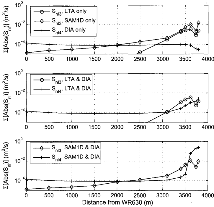
Figure 5.21: Integrated magnitudes of the nonlinear source terms during simulation of the SandyDuck '97 event of 13/11/1997 at 19:00. Results for various combinations of the LTA, the two-equation model and the DIA.
