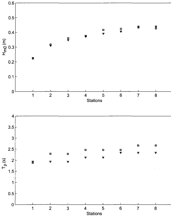
Figure 3.9: Lake George field experiment of near-idealised, depth-limited wave growth. Wave height and peak period obtained with \alpha = 0.0 and \gamma = 0.1 after 500 iterations (plusses), with \alpha = 0.05 and \gamma = 0.5 after 500 iterations (triangles) and observations of Young and Verhagen (1996) (squares). Note: all plusses virtually coincide with the triangles and for that reason are not separately visible.
