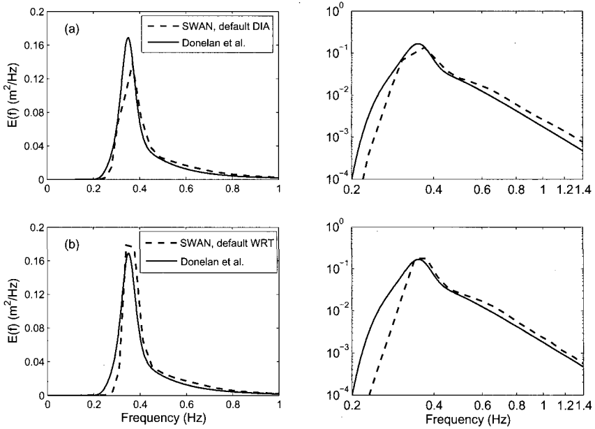
Figure 4.3: Comparison between the deep water, fetch-limited spectra produced using the default Komen et al. (1984) wind and whitecapping expressions and the DIA (row (a)) and the WRT exact method (row (b)) and the parametric form of Donelan et al. (1985) with the peak frequency and total energy according to Kahma and Calkoen (1992). Results for U_{10} = 10 m/s.
