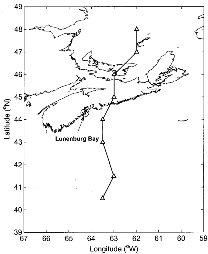
Figure 4.15: Map showing location of Lunenburg Bay in Nova Scotia, Canada, and the track of Tropical Storm Nicole, which passed in October 2004 (line with triangles).
