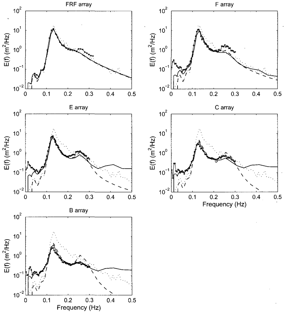
Figure 5.26: Comparison between simulated and observed frequency spectra, for Sandy-Duck '97 event of 13/11/1997 at 19:00. Simulation including both shallow and deep water source terms, the latter according to the saturation-based combination. Quadruplet interaction (DIA) only active for Ur < 0.1 . Shown are the results of the LTA model (dashed line), the two-equation model (solid line) and observations (line with circles). Input spectrum at the WR630 buoy indicated by dotted line.
