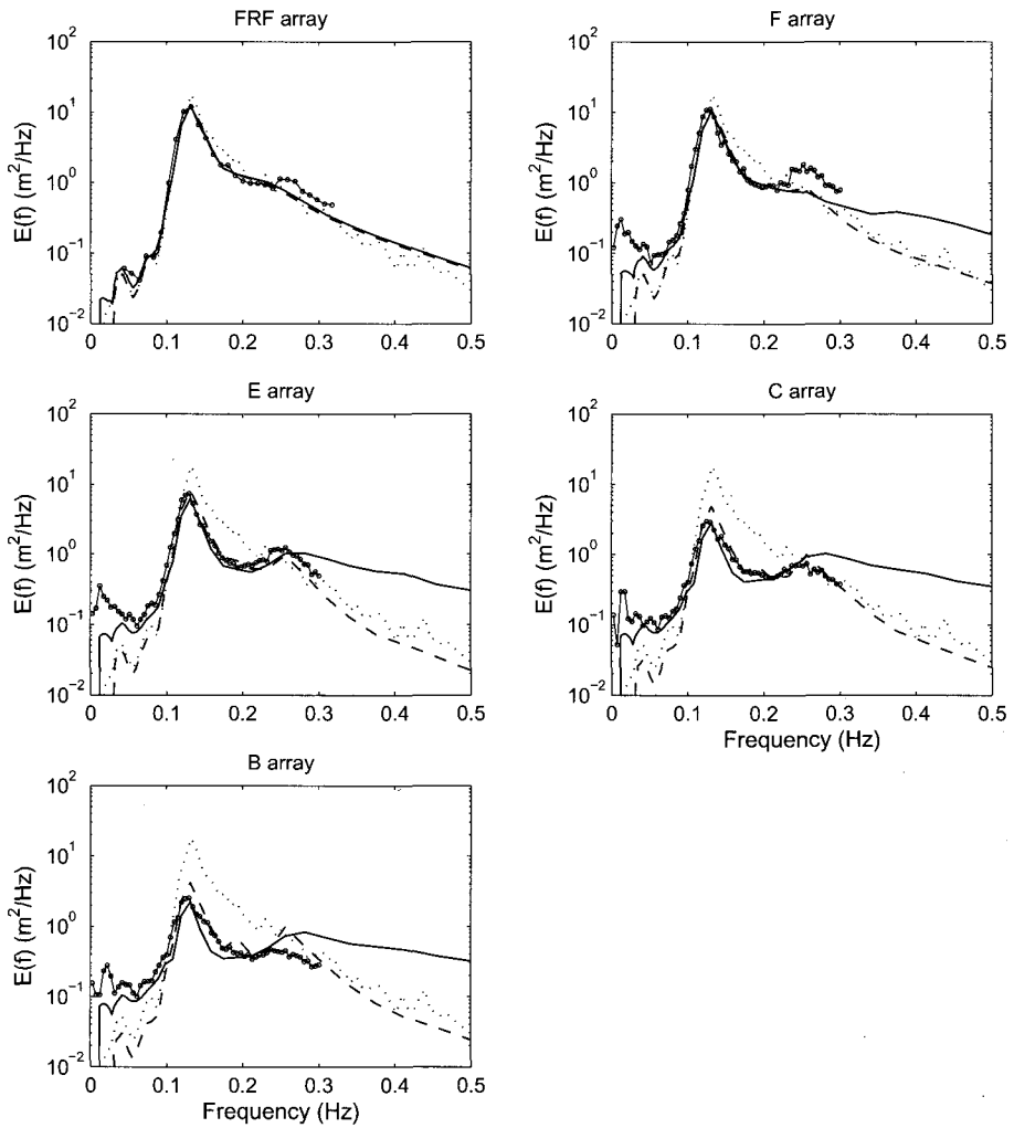
Figure 5.17: Comparison between simulated and observed frequency spectra, for Sandy-Duck '97 event of 13/11/1997 at 19:00. Simulation including both shallow and deep water source terms, active over the entire domain. Shown are the results of the LTA model (dashed line), the two-equation model (solid line) and observations (line with circles). Input spectrum at the WR630 buoy indicated by dotted line.
