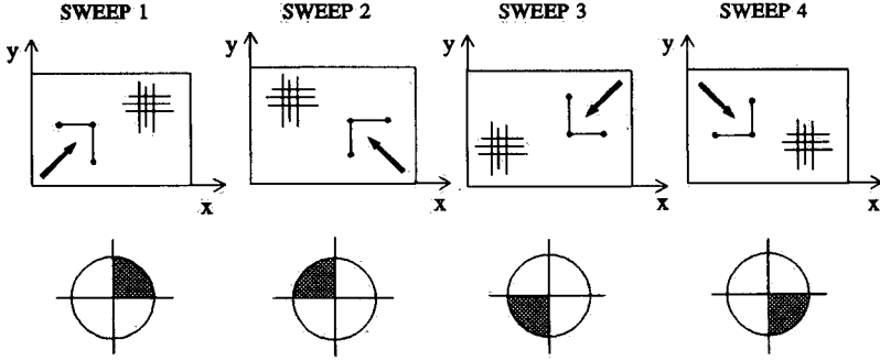
Figure 2.1: The solution procedure for wave energy propagation in geographical space with the appropriate directional quadrant (indicated by shaded area) for each of four sweeps (Ris 1997).
