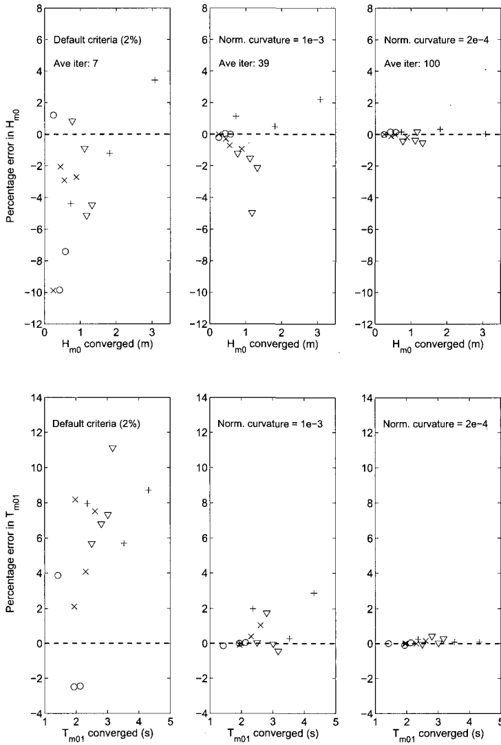
Figure 3.20: Top panels: Percentage error in H_{m0} at output points incurred using three different stopping criteria, defined as (H_{m0,stopped} - H_{m0,converged})/H_{m0,converged} , plotted against H_{m0,converged} , for various test cases. Left-hand panel: default criteria, centre panel: new curvature criterion with \varepsilon_C = 1e-3 , right-hand panel: curvature criterion with \varepsilon_C = 2e-4 . The average number of iterations before run termination is indicated in each case. Bottom panels: Corresponding results for T_{m01} . In all panels the results plotted are of 14 individual cases, featuring: + deep water fetch-limited growth, O Lake George, x Norderneyer Seegat and \nabla Haringvliet.
