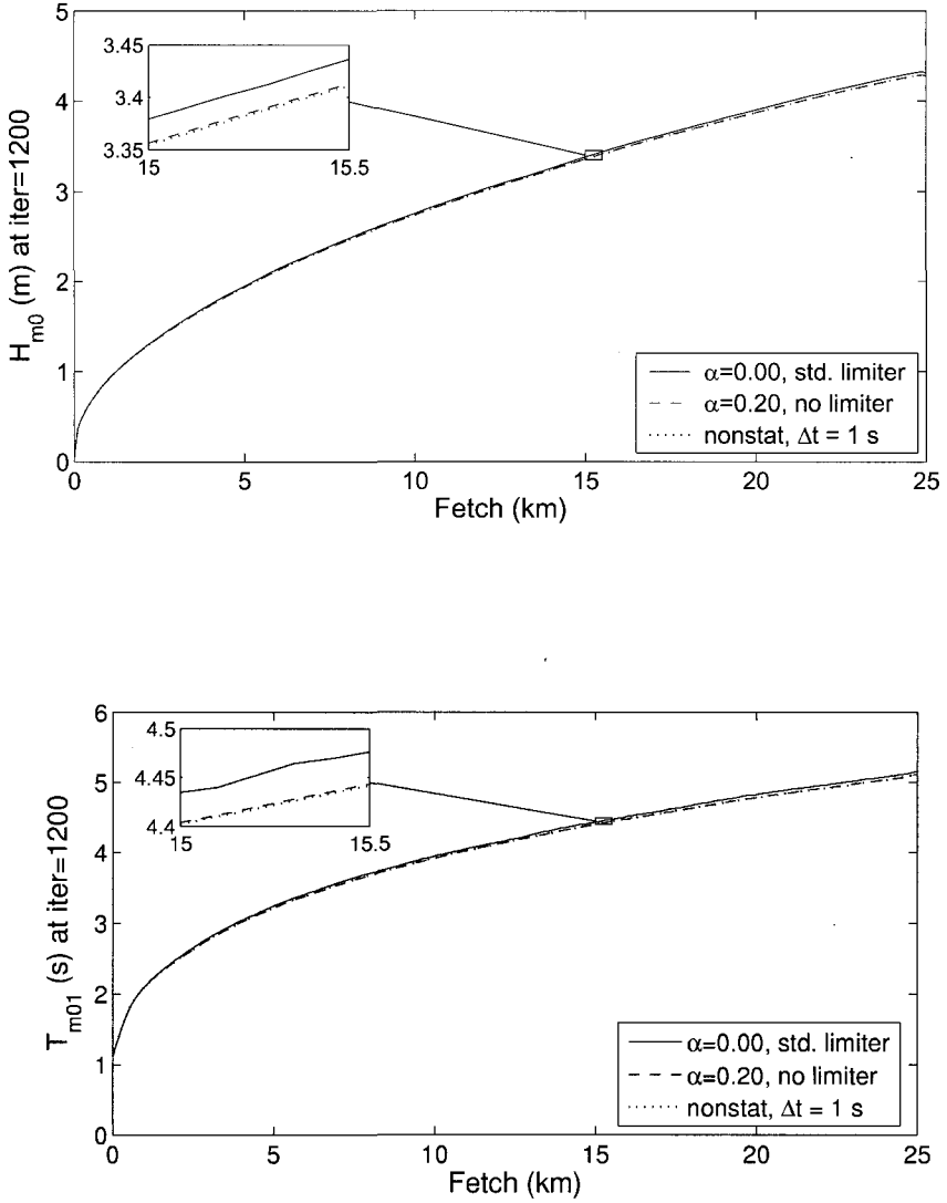
Figure 3.5: Growth curves of H_{m0} (top panel) and T_{m01} (bottom panel) in deep-water, fetch-limited simulations for a wind speed of U_{10} = 30 m/s. Results for stationary SWAN with limiter, for \alpha = 0.20 without limiter and nonstationary SWAN with \Delta t = 1 s.
