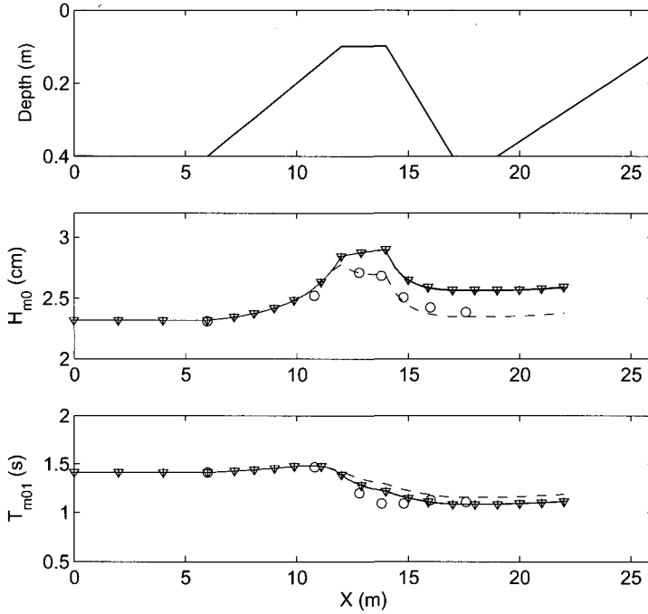
Figure 3.10: Spatial development of wave height and period during the iteration process of a case from the laboratory experiment of Beji and Battjes (1993). Top panel: Depth profile of the experiment. Middle and lower panels: Simulation results obtained with the setting \alpha = 0.0 and \gamma = 0.1 after 10 iterations (dashed) and 100 iterations (solid with plusses), and those obtained with \alpha = 0.0 and \gamma = \infty upon convergence (after about 10 iterations, solid with triangles). Note: all plusses virtually coincide with the triangles and for that reason are not separately visible. Observations indicated by circles.
