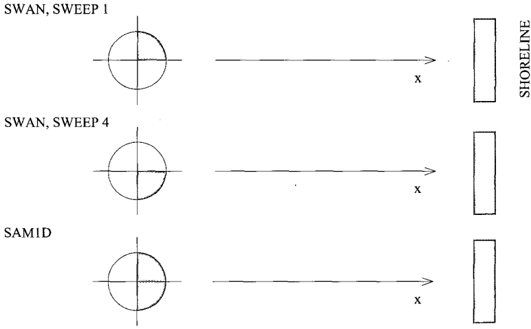
Figure 5.7: Diagram of the propagation directions in geographical space for the combination model of SWAN and SAM1D. Shown are the directional quadrants of sweeps 1 and 4 in SWAN that exchange information with SAM1D (shaded areas, refer Figure 2.1), and the semi-circle of directions that is solved during one spatial step in SAM1D.
