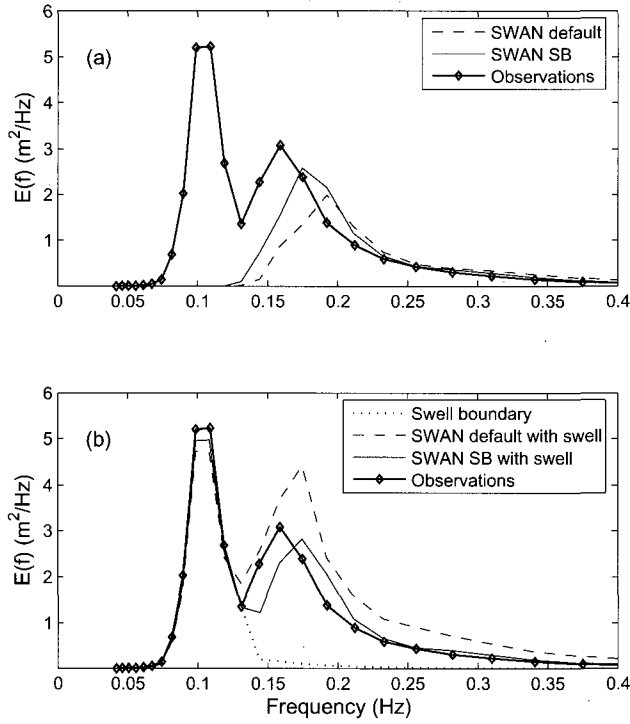
Figure 4.13: Results of simulations over the North Carolina shelf at downwind Station X6. (a) Spectra of the saturation-based and default models in simulations without swell. (b) Corresponding results of simulations with ambient swell. Average wind speed is U_{10} = 9.5 m/s.
