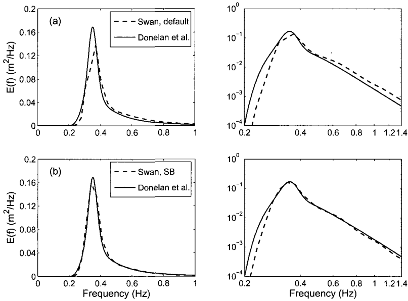
Figure 4.9: Deep water fetch-limited spectra produced using the default model (row (a)) and the saturation-based model (SB) (row (b)). Spectra on the left are repeated on the right on logarithmic axes. Results for U_{10} = 10 m/s at X^* = 6 \times 10^5 .
