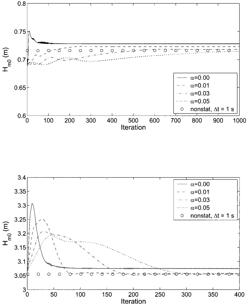
Figure 3.2: Convergence behaviour of H_{m0} in deep-water, fetch-limited simulations for wind speeds U_{10} = 10 m/s (top panel) and 30 m/s (bottom panel), at fetch = 12.5 km. Results for SWAN with \gamma = 0.1 and \alpha = 0.0 –0.05. Also shown is nonstationary SWAN with \Delta t = 1 s.
