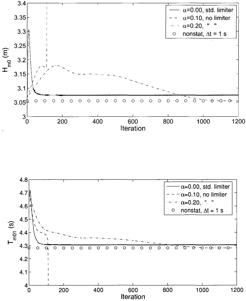
Figure 3.4: Convergence behaviour of H_{m0} (top panel) and T_{m01} (bottom panel) in deep-water, fetch-limited simulations for a wind speed of U_{10} = 30 m/s, at fetch = 12.5 km. Results for SWAN without limiter ( \gamma = \infty ) and various large under-relaxation factors ( \alpha = 0.10 – 0.20 ). Also shown are stationary SWAN with \gamma = 0.1 and \alpha = 0 , and nonstationary SWAN with \Delta t = 1 s.
