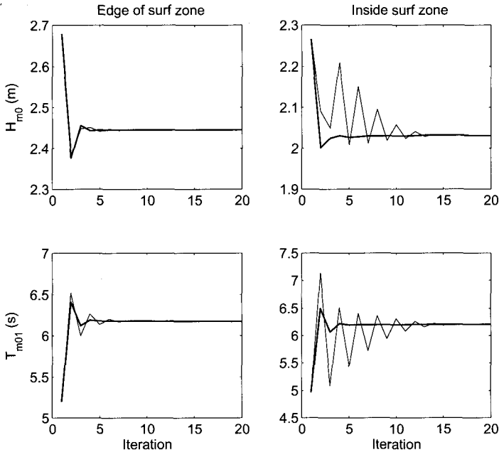
Figure 5.8: Comparison between the iteration behaviour of the combined SWAN-SAM model when computing triad interactions per sweep (thick line) and per iteration (thin line). Results for a bar beach field case at Duck, North Carolina, at the offshore edge of the surf zone (left-hand panels) and deep inside the surf zone (right-hand panels).
