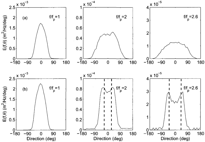
Figure 4.4: Simulated directional distributions at the peak and energy-containing tail produced using the DIA (row (a)) and the WRT method (row (b)) at three different frequencies. Results for deep-water, fetch-limited growth with U_{10} = 10 m/s at X^* = 6 \times 10^5 . The dashed lines in row (b) are the locations of the bi-modal peaks observed by Hwang et al. (2000).
