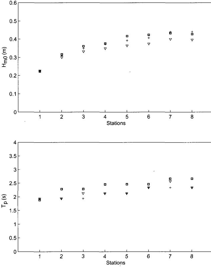
Figure 3.19: Lake George field experiment of near-idealised, depth-limited wave growth. Wave height and peak period obtained with the default stopping criteria (3.5) and (3.6) with \varepsilon_H^r = \varepsilon_T^r = 0.02 , \varepsilon_H^a = 0.02 m and \varepsilon_T^a = 0.2 s (6 iterations, triangles), with the termination criteria (3.5), (3.6) and (3.9) with \varepsilon_C = 2e-4 (30 iterations, plusses) and observations of Young and Verhagen (1996) (squares).
