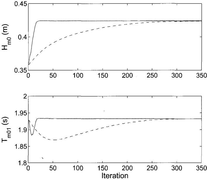
Figure 3.7: Lake George field experiment of near-idealised, depth-limited wave growth. Iteration curves at Station 8 for significant wave height (top panel) and mean period (bottom panel), for simulations with the setting \alpha = 0.0 and \gamma = 0.1 (default limiter, solid) and the setting \alpha = 0.05 and \gamma = 0.5 (strong under-relaxation and weak limiter, dashed). Wind speed is U_{10} = 10.8 m/s.
