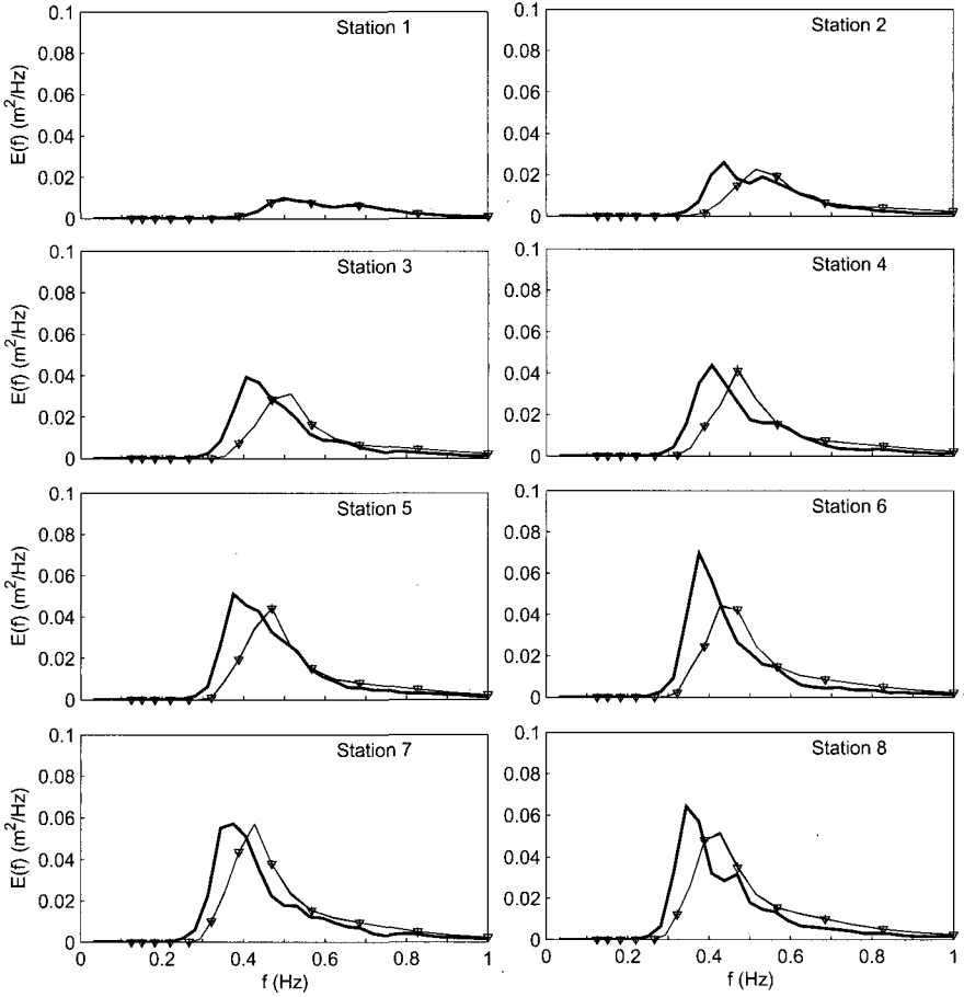
Figure 3.8: Lake George field experiment of near-idealised, depth-limited wave growth. Frequency spectra obtained with \alpha = 0.0 and \gamma = 0.1 after 500 iterations (plusses), with \alpha = 0.05 and \gamma = 0.5 after 500 iterations (triangles) and observations of Young and Verhagen (1996) (thick line). Note: all plusses virtually coincide with the triangles and for that reason are not separately visible.
