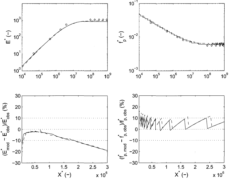
Figure 4.2: Deep water, fetch-limited growth curves produced using the default Komen et al. (1984) formulations for wind and whitecapping combined with respectively the DIA (dashed lines) and WRT (solid lines) quadruplet interaction expressions. Top panels: comparison with fetch-limited relations of Kahma and Calkoen (1992) (circles) and Pierson and Moskowitz (1964) (diamonds). Bottom panels: bias of model results with respect to Kahma and Calkoen (1992) data. Results for U_{10} = 10 m/s.
