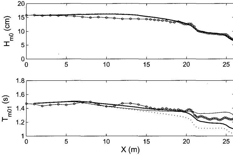
Figure 5.6: Comparison between wave height and mean period produced using the LTA and laboratory observations of Boers (1996) (Case 1A). Simulation results with parameter combinations (a) \alpha_{EB} = 0.1 and f_{max,EB} = 2.2f_{m01} (thin solid line), (b) \alpha_{EB} = 0.1 and f_{max,EB} = 2.5f_{m01} (dotted line) and (c) \alpha_{EB} = 0.05 and f_{max,EB} = 2.5f_{m01} (thick solid line) are shown. Observations are indicated by line with circles.
