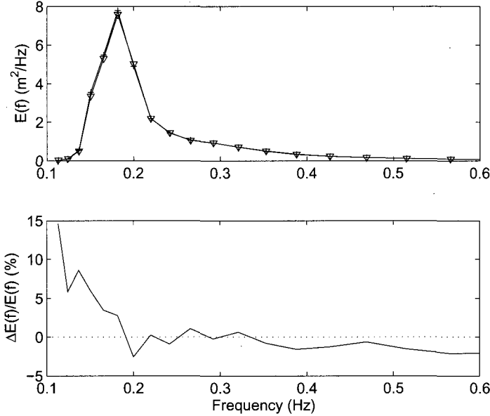
Figure 3.6: Spectra produced during deep-water, fetch-limited simulations with and without action limiter. Top panel: comparison between the converged results for the setting \alpha = 0 and \gamma = 0.1 (default limiter, line with plusses) and for the setting \alpha = 0.20 and \gamma = \infty (under-relaxation and no limiter, line with triangles). (Note that all plusses virtually coincide with the triangles and for that reason are not separately visible.) Bottom panel: the difference between these results, expressed as [E_{\gamma=0.1}(f) - E_{\gamma=\infty}(f)]/E_{\gamma=\infty}(f) . Wind speed is U_{10} = 30 m/s and fetch is 12.5 km.
