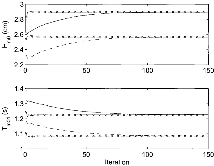
Figure 3.11: Iteration behaviour of wave height and period during the simulation of a case from the laboratory experiment of Beji and Battjes (1993). Shown are the results obtained with the setting \alpha = 0.0 and \gamma = 0.1 at x = 13.8 m (solid) and x = 17.6 m (dashed), and those obtained with \alpha = 0.0 and \gamma = \infty at the same locations (solid and dashed respectively, with circles).
