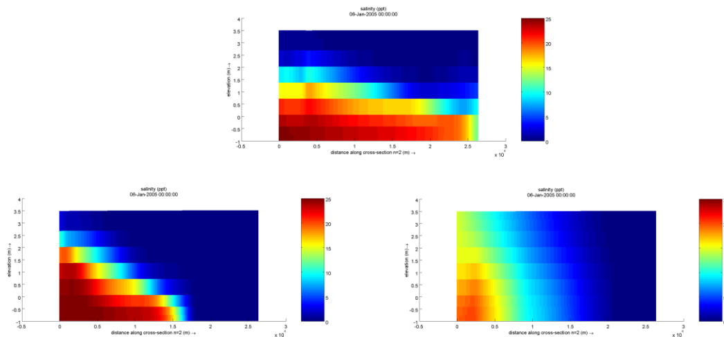
Figure 8: effect of viscosity and diffusion coefficients ( \text{m}^2/\text{s} ) on the simulation result (top: VicoWW 0,0001, DicoWW 1E-07 ; bottom left: VicoWW 0,001; bottom right DicoWW 0,0001) (red: salt water; blue: fresh water)
