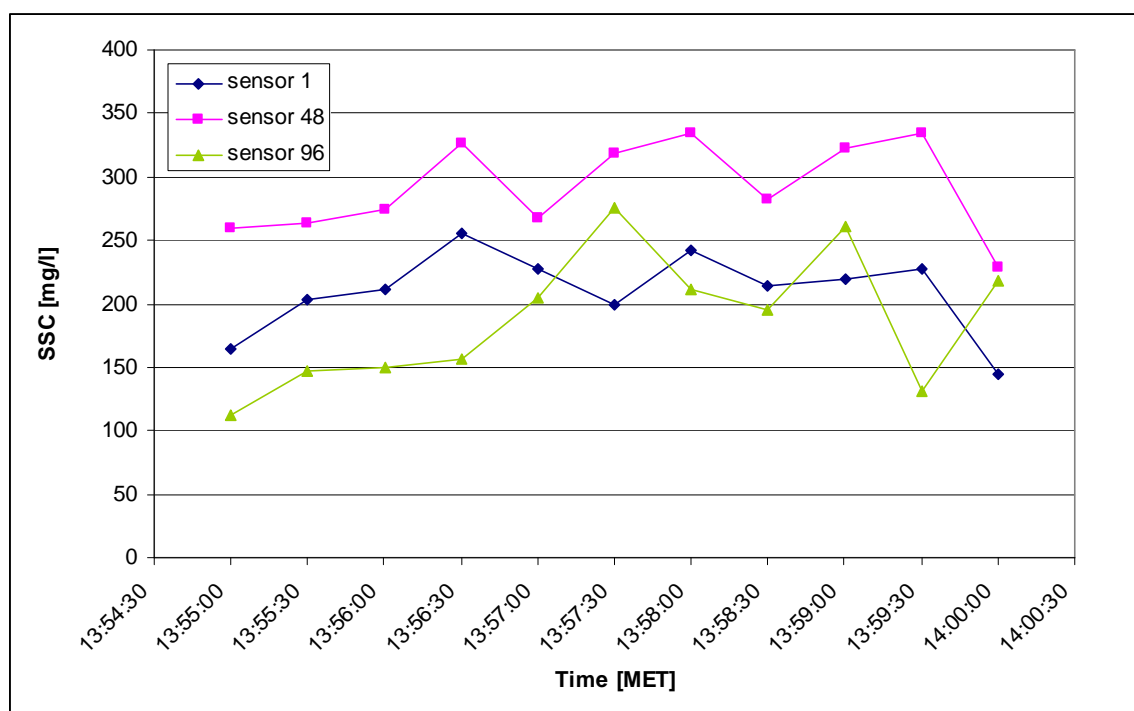
Figure 4-4: Timeseries in a high SSC environment for 3 sensors of Argus: X-axis shows time, Y-axis shows SSC: Argus sn 79.
