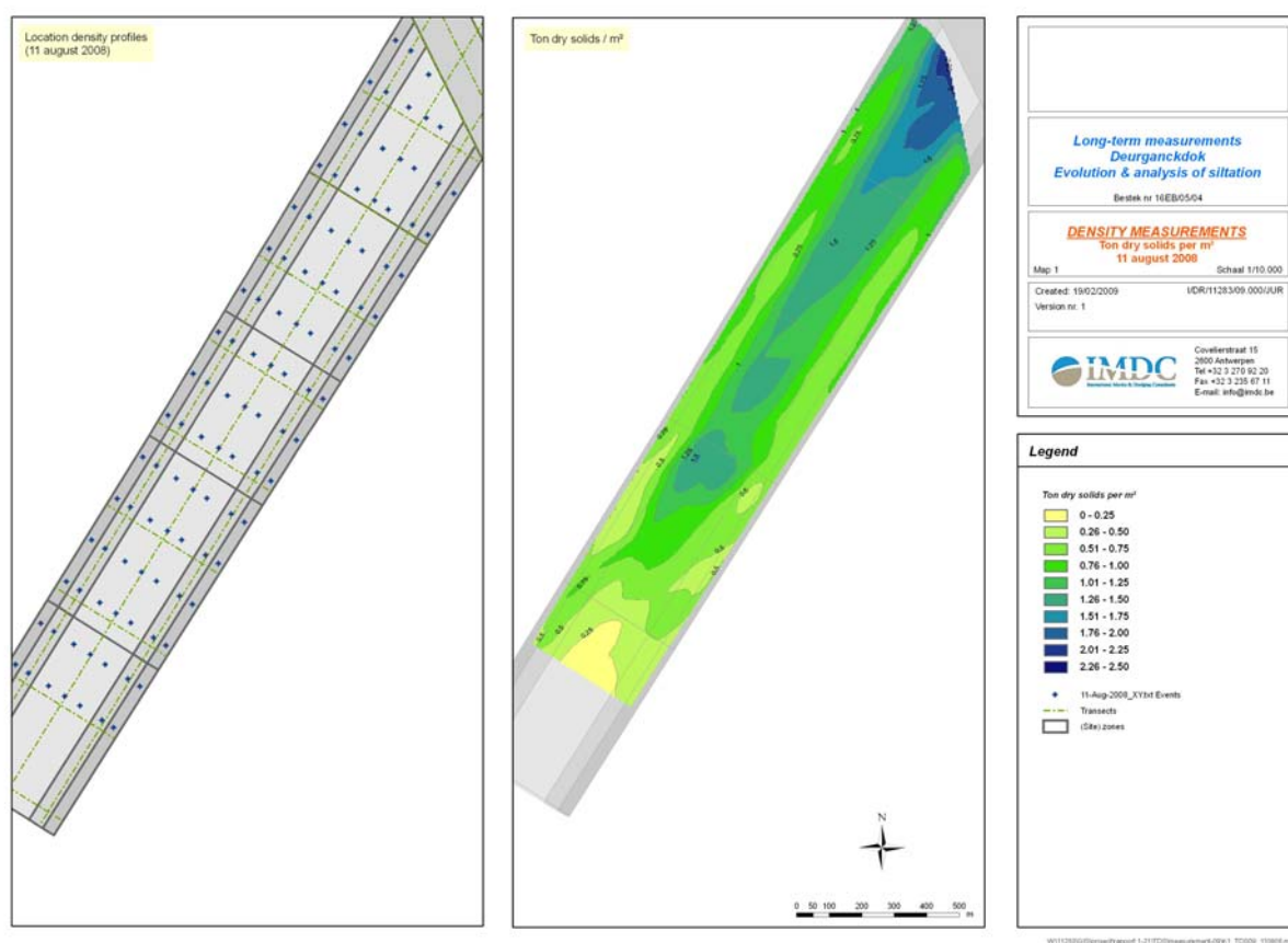
Figure 4-10: Map showing the location of the density profiles (left) and the calculation of TDS (right) on 11/08/08
