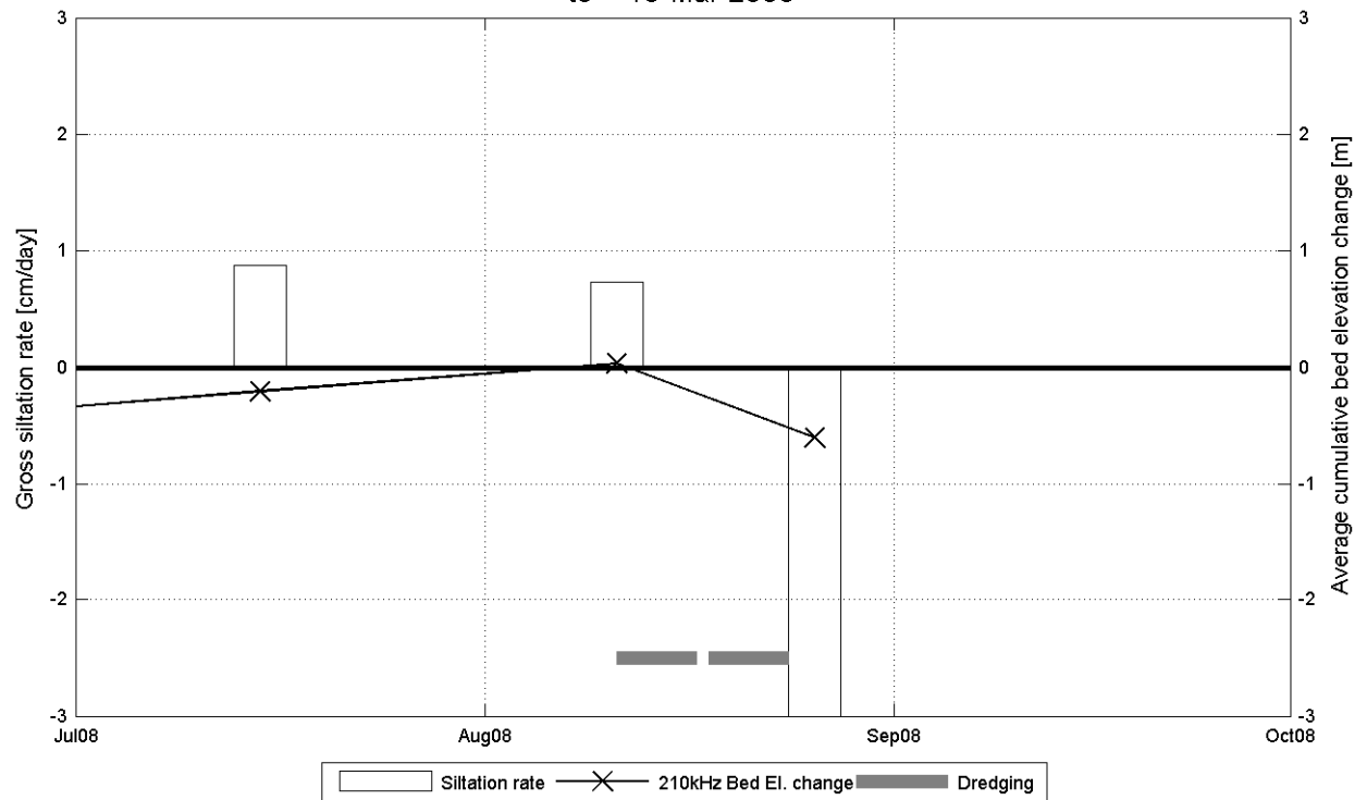
Gross siltation over section D2 t0 = 13-Mar-2008
