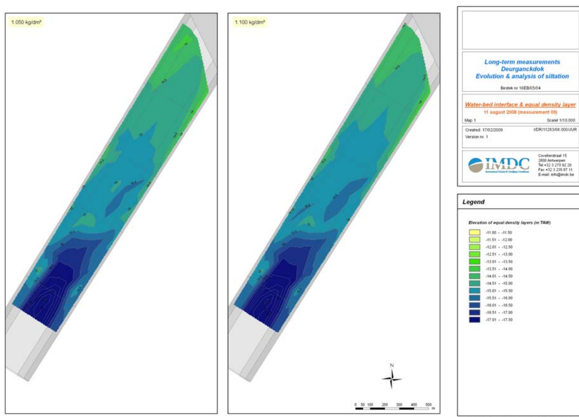
Figure 4-8: Map of the depth of the water-bed interface and equal density layers for 11/08/08
