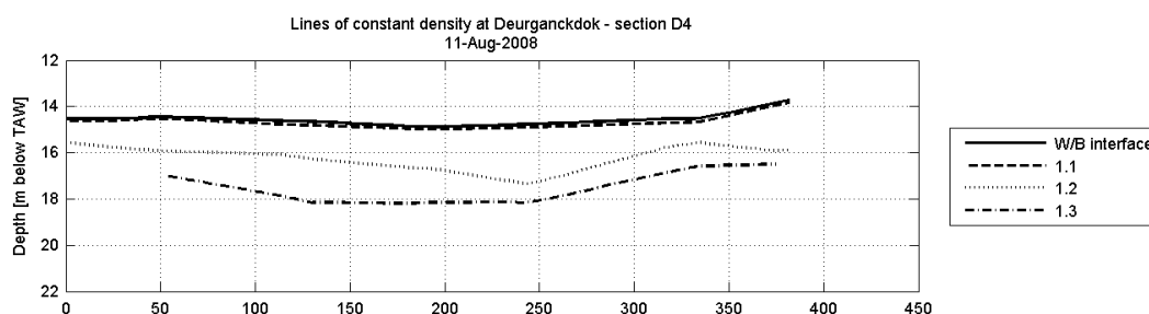
Figure 4-7: Depth of water-bed interface and equal density layers in section D4 on 11 August 2008
