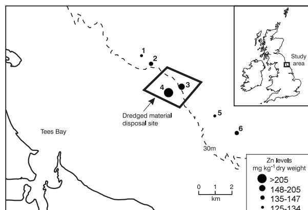
Figure 59. Concentrations of zinc ( \text{mg kg}^{-1} dry weight) in sediments from stations 1-6 along the Tees Bay transect
