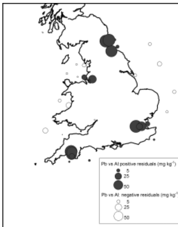
Figure 27. Lead vs. aluminium residuals ( \text{mg kg}^{-1} ). Concentrations are presented as area proportional symbols; scale symbols are shown in the legend
