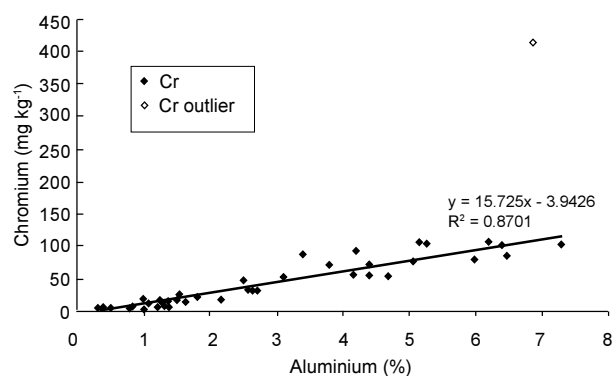
Figure 28. Chromium ( \text{mg kg}^{-1} ) vs. aluminium (%) in sediment
