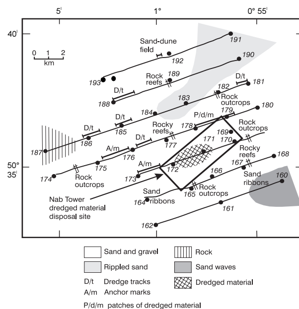
Figure 57. Distribution of sediments and seabed features over the survey area
