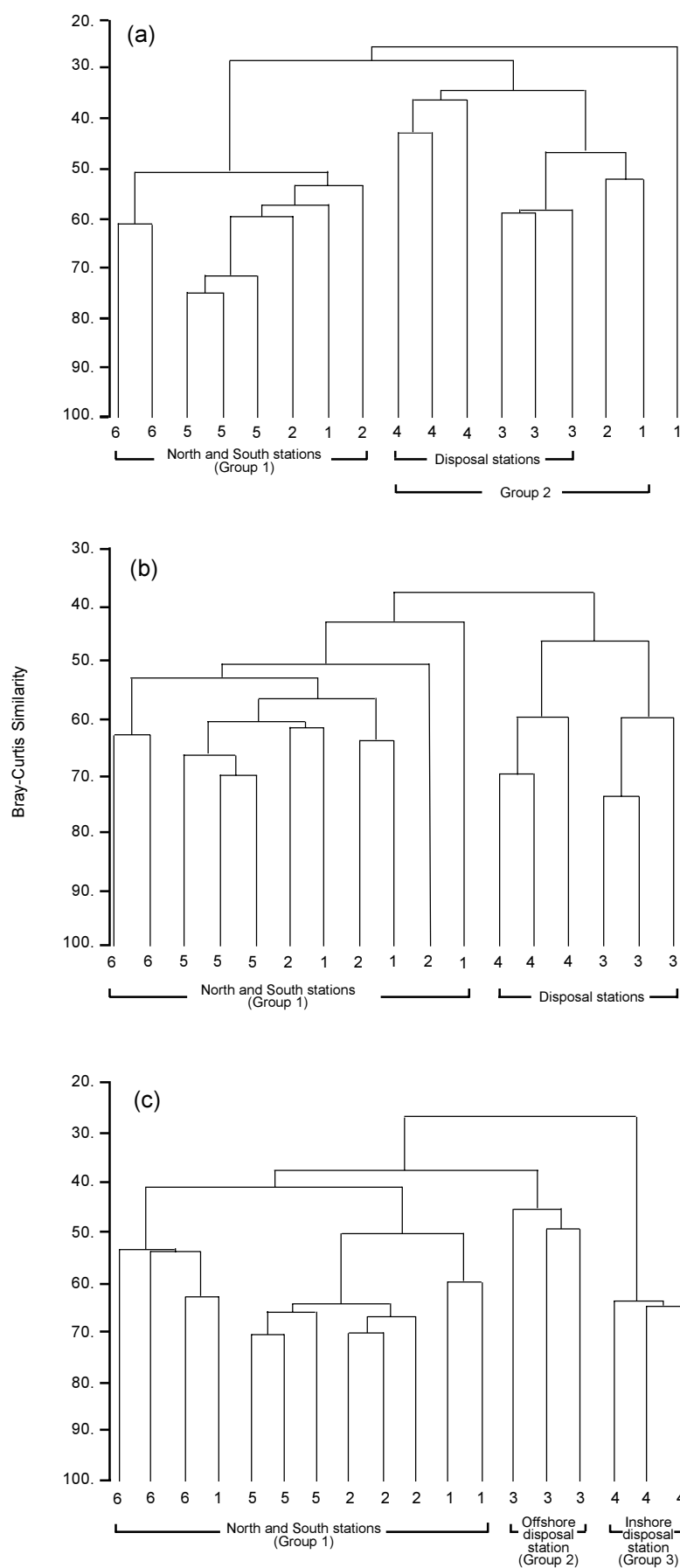
Figure 63. Dendrograms for group average clustering of Bray Curtis similarities based on square-root transformed data for stations 1-6 (a) macrofauna (b) meiografauna (grab sub-samples) (c) meiografauna (cores)
