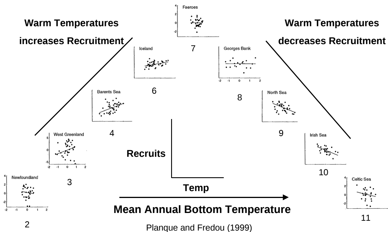
Figure A7. The relationship between recruitment and temperature for various cod stocks. The numerical values at the bottom of the plots represent mean annual bottom temperatures. Note that the relationship is generally positive for the cold-water stocks, but is negative for the warm-water stocks. There is no relationship in the mid-temperature range. (Based on Planque and Fr  dou, 1999.)
