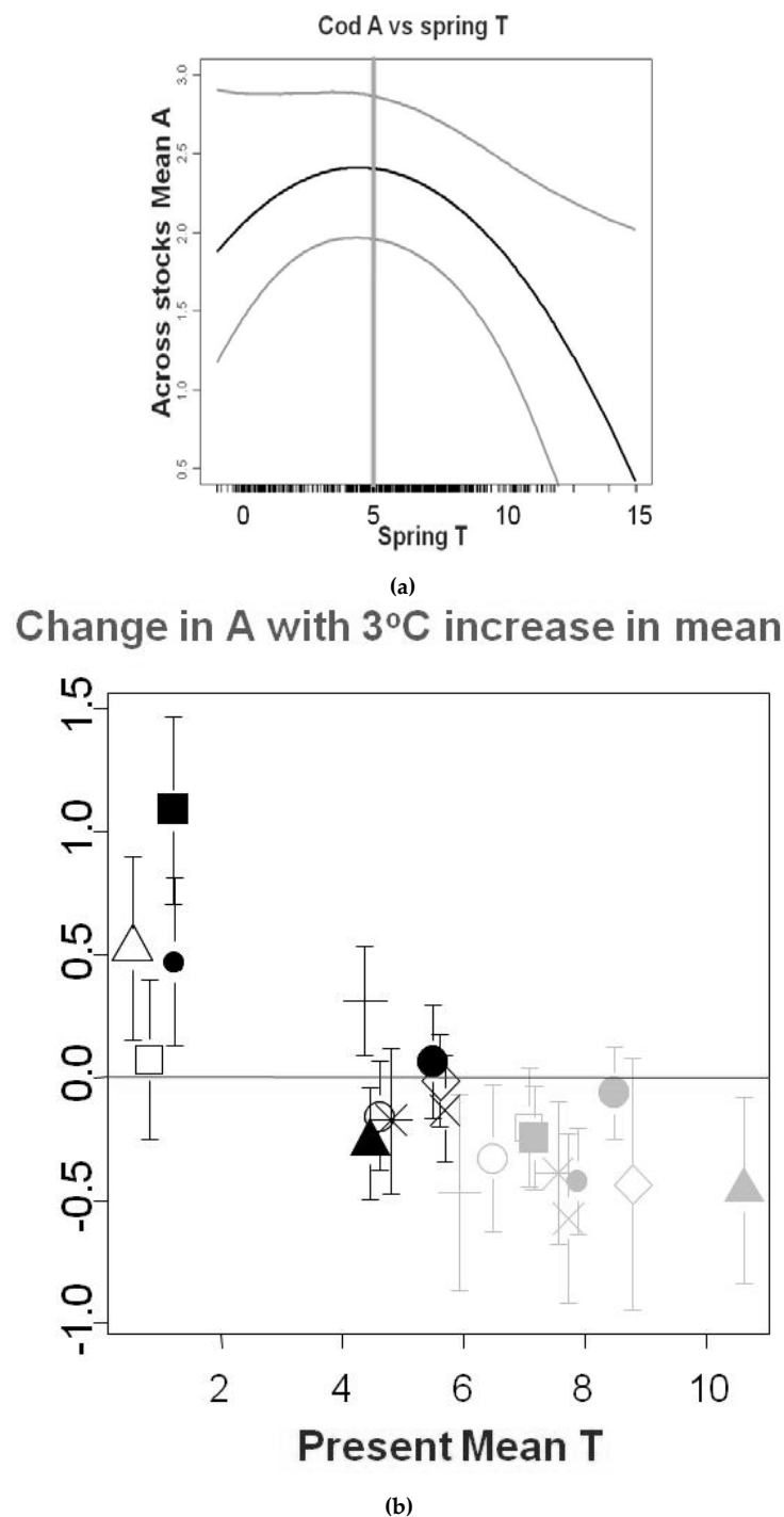
Figure A11. (a) The mean quadratic relationship of parameter alpha (slope at the origin in the Ricker model) with T . (b) The expected change in stock-specific alphas following an increase of 3°C in mean T . Grey (black) symbols correspond to stocks in warmer (or colder) waters.
