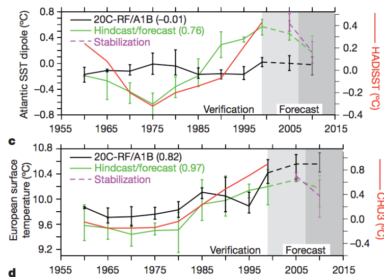
Figure 3.9. Modelled Atlantic SST dipole and European surface temperature with the decadal prediction systems of Keenlyside et al. (2008) and the IPCC 20th-century reference and an A1B projection run.
