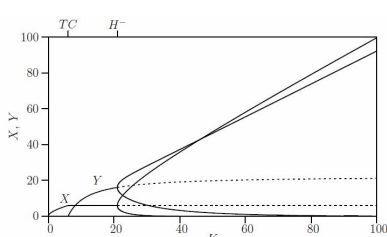
Figure 10: One-parameter bifurcation diagram of a system with species X and Y and bifurcation parameter K . Parameters are R = 0.5 , A = 0.5 , B = 9 , C = 0.4 , D = 0.08 . The first transcritical bifurcation occurs at the origin, with the invasion of X . Then, at K \approx 6 , also Y invades. The latter situation is referred to as coexistence of X and Y . At K \approx 20 a Hopf bifurcation H^- occurs, and a stable limit cycle is born. The minimal and maximal values of X and Y are also depicted; the unstable equilibrium is shown as dashed curves.
