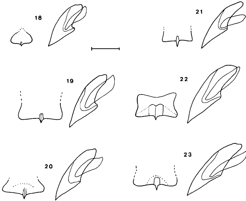
Figs 18–23. Radulae of: 18, Clionella subventricosa kaffraria ; 19, C. striolata ; 20, C. rosaria ; 21, Benthoclionella jenneri ; 22, Clavatula tripartita ; 23, Clionella bornii . Scale-line = 0,1 mm.
