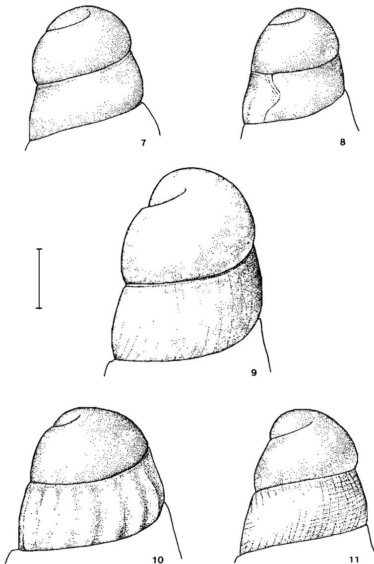
Figs 7-11. Protoconchs of: 7, Clavatula helena ; 8, C. halistrepta ; 9, Toxicionella tumida ; 10, T. (Caliendrula) elstoni ; 11, T. haliplex . Scale-line = 1 mm.
