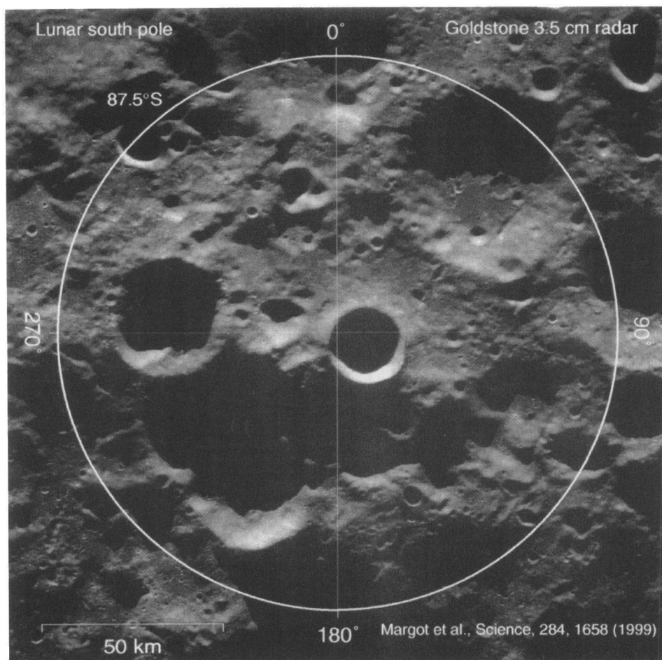
Fig. 1. The Adrien de Gerlache crater is located at 88.5^{\circ} S and 273^{\circ} E at about 40 km of the South Pole of the Moon, close to the already known Shackleton and Amundsen craters. The crater has a diameter of 32 kilometres and a probable depth of 3 kilometres.
